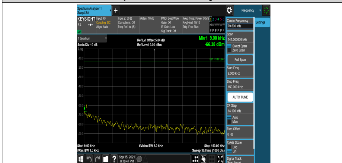
Band2-3MHz-16QAM-18900-1RB#0-Range1:0.009~0.15MHz
