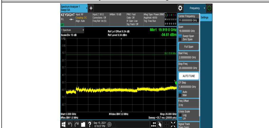
Band2-3MHz-16QAM-18900-1RB#0-Range5:2000~20000MHz
