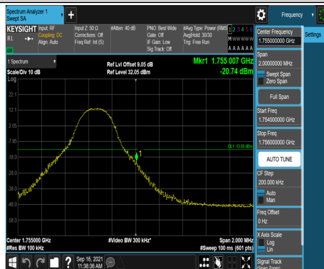
Band4-5MHz-QPSK-20375-1RB#24
