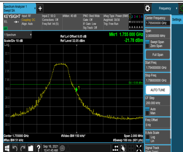
Band4-3MHz-16QAM-20385-1RB#14
