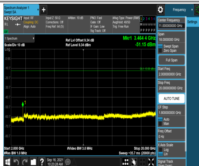
Band4-1.4MHz-16QAM-20175-1RB#0-Range5:2000~20000MHz
