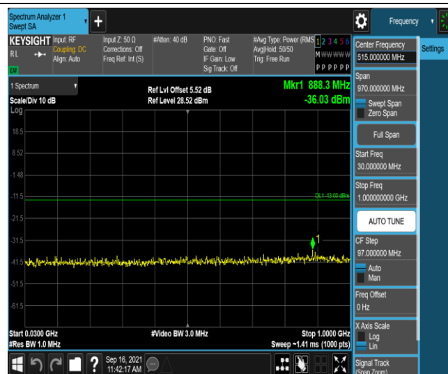
Band4-5MHz-QPSK-20175-1RB#0-Range3:30~1000MHz
