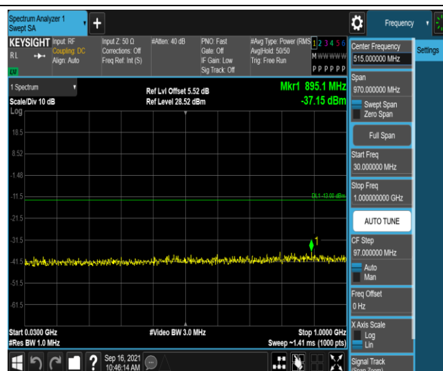
Band4-3MHz-16QAM-20175-1RB#0-Range3:30~1000MHz
