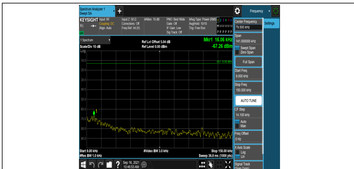
Band4-3MHz-QPSK-20385-1RB#0-Range1:0.009~0.15MHz
