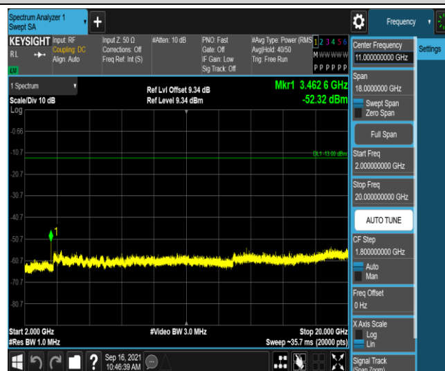
Band4-3MHz-16QAM-20175-1RB#0-Range5:2000~20000MHz
