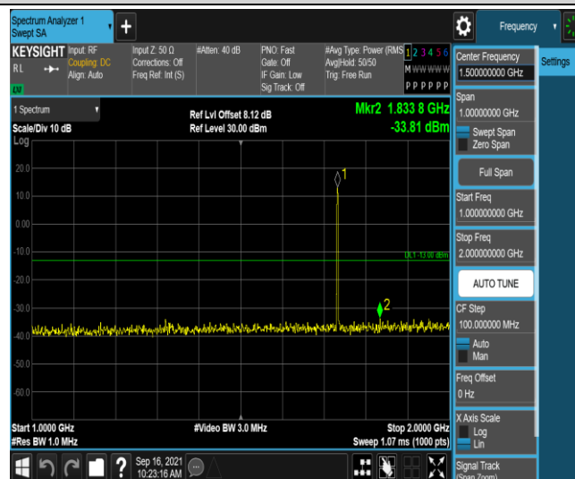
Band4-1.4MHz-16QAM-20175-1RB#0-Range4:1000~2000MHz
