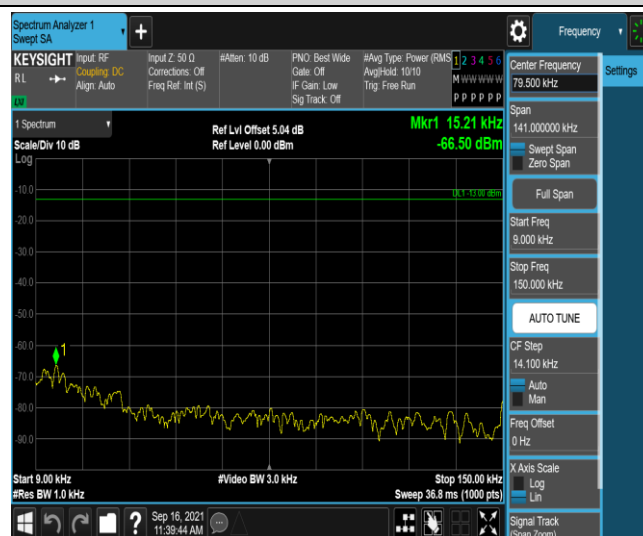
Band4-5MHz-QPSK-19975-1RB#0-Range1:0.009~0.15MHz
