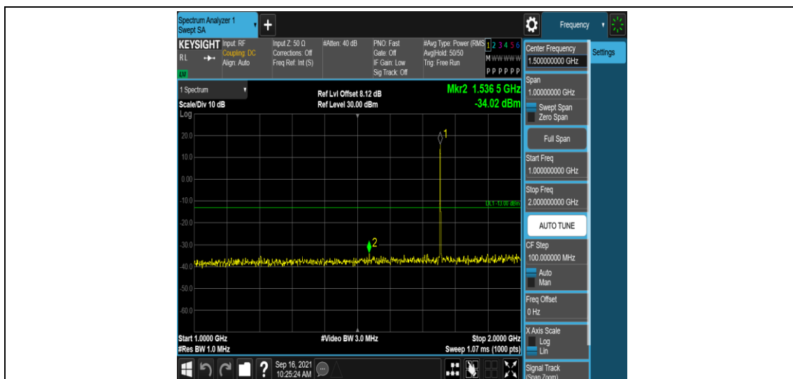
Band4-1.4MHz-16QAM-20393-1RB#0-Range4:1000~2000MHz
