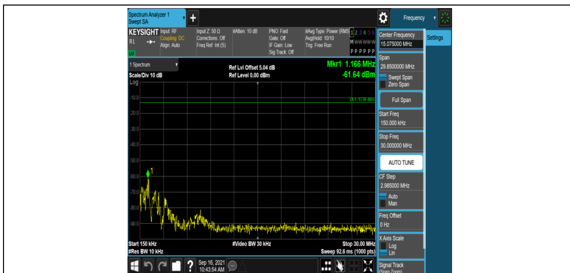
Band4-3MHz-16QAM-19965-1RB#0-Range2:0.15~30MHz
