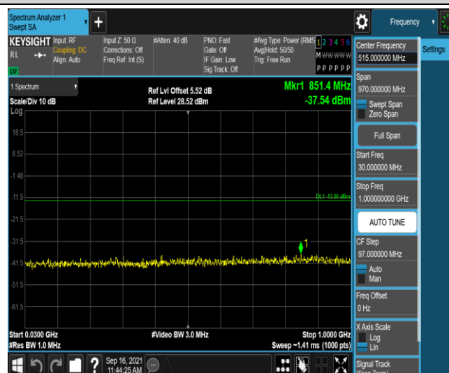
Band4-5MHz-QPSK-20375-1RB#0-Range3:30~1000MHz
