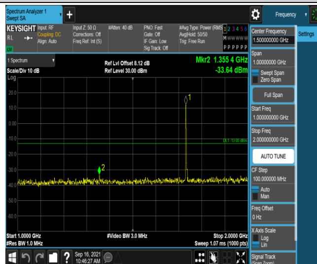
Band4-3MHz-16QAM-20175-1RB#0-Range4:1000~2000MHz
