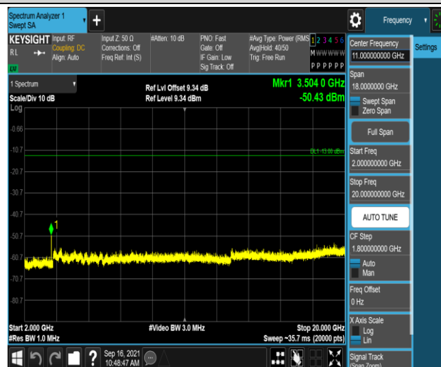
Band4-3MHz-16QAM-20385-1RB#0-Range5:2000~20000MHz
