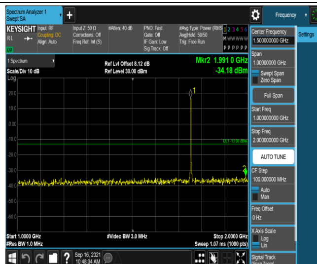
Band4-3MHz-16QAM-20385-1RB#0-Range4:1000~2000MHz
