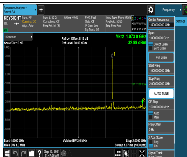
Band4-5MHz-16QAM-20375-1RB#0-Range4:1000~2000MHz
