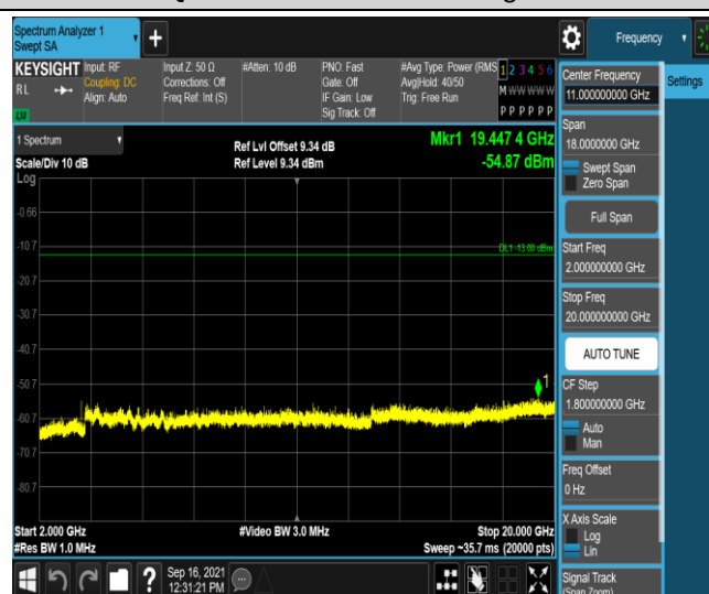
Band4-15MHz-QPSK-20175-1RB#0-Range5:2000~20000MHz
