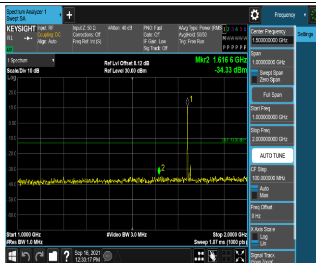
Band4-15MHz-QPSK-20325-1RB#0-Range4:1000~2000MHz
