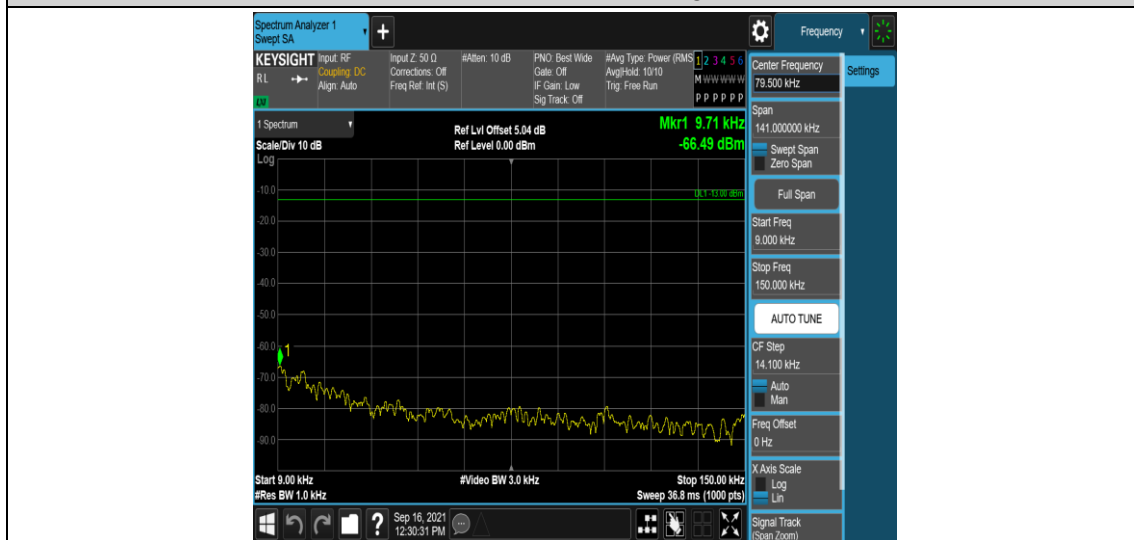
Band4-15MHz-QPSK-20175-1RB#0-Range1:0.009~0.15MHz
