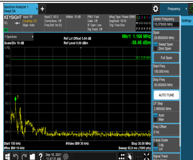
Band4-5MHz-16QAM-20375-1RB#0-Range2:0.15~30MHz
