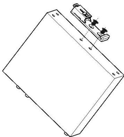
Clip Assembling
