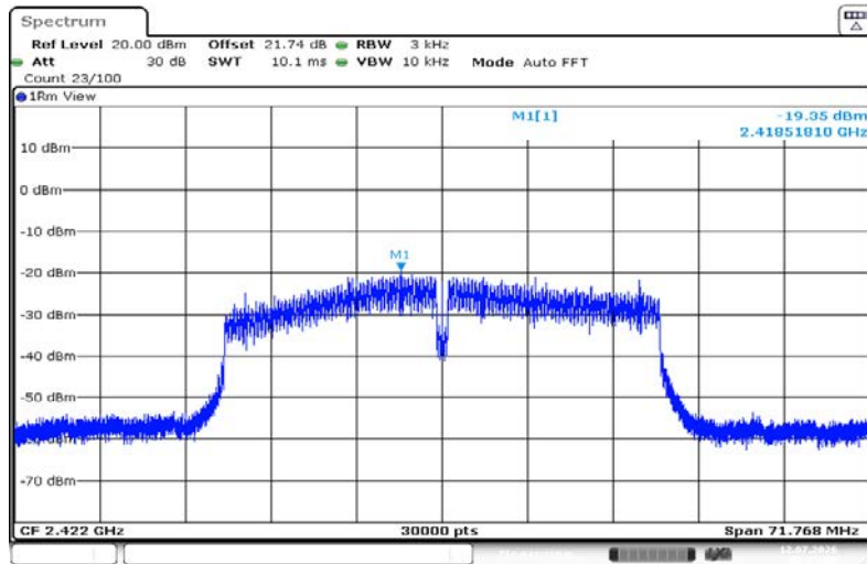
11N40SISO-Ant1-2422-PASS
