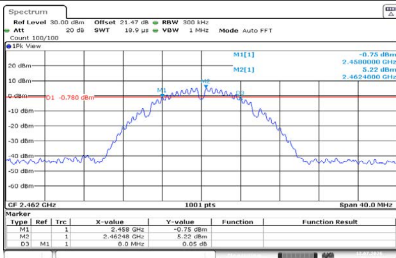
11B-Ant1-2462-PASS
