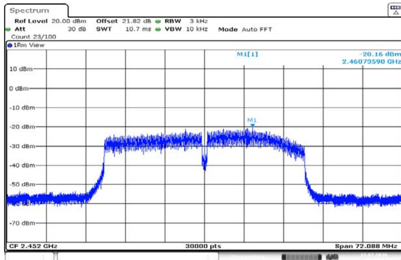
11N40SISO-Ant1-2452-PASS
