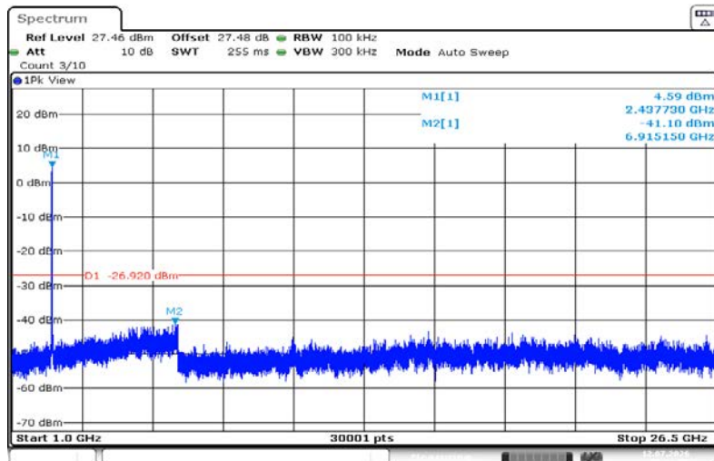
11G-Ant1-2437-1000~26500-PASS
