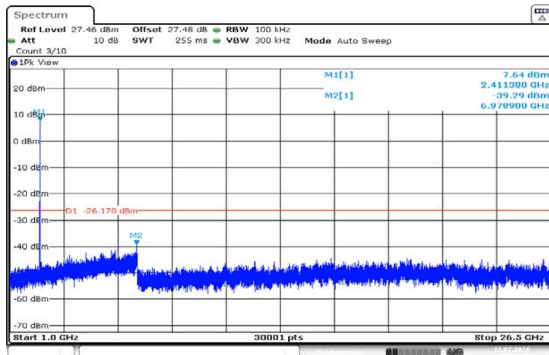
11B-Ant1-2412-1000~26500-PASS
