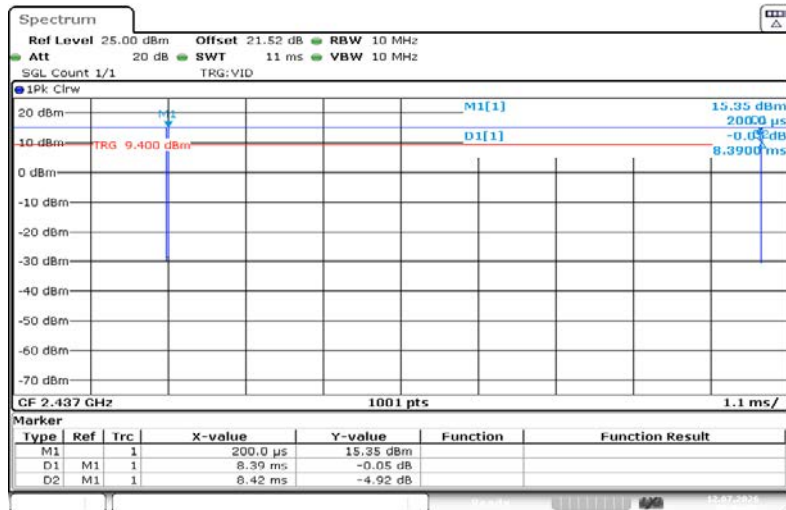
NTNV-11B-Ant1-2437
