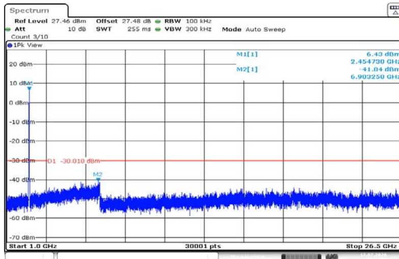
11N40SISO-Ant1-2437-1000~26500-PASS
