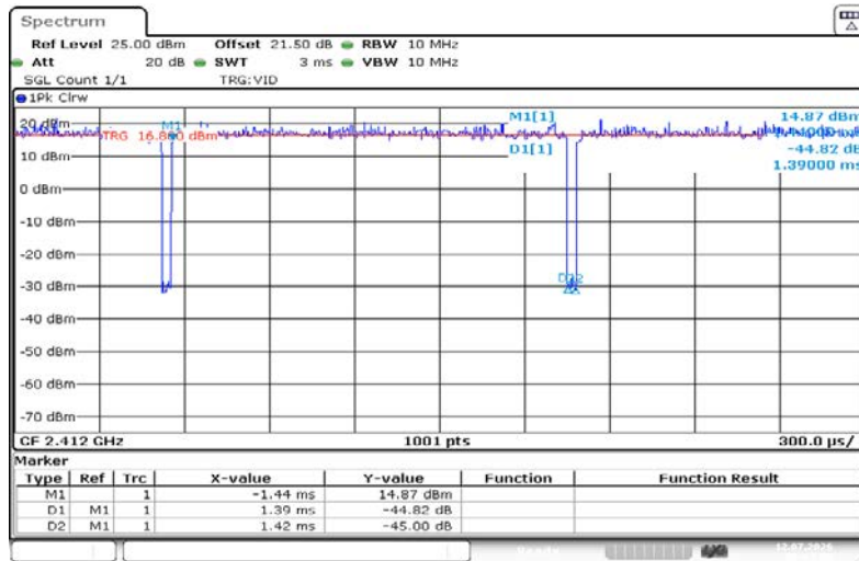
NTNV-11G-Ant1-2412
