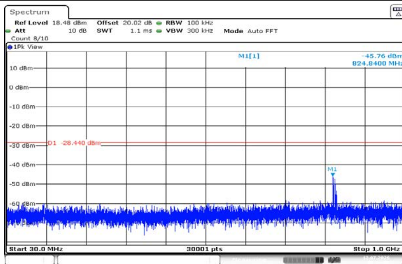
11N40SISO-Ant1-2422-30~1000-PASS
