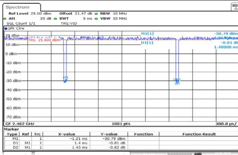
NTNV-11G-Ant1-2462
