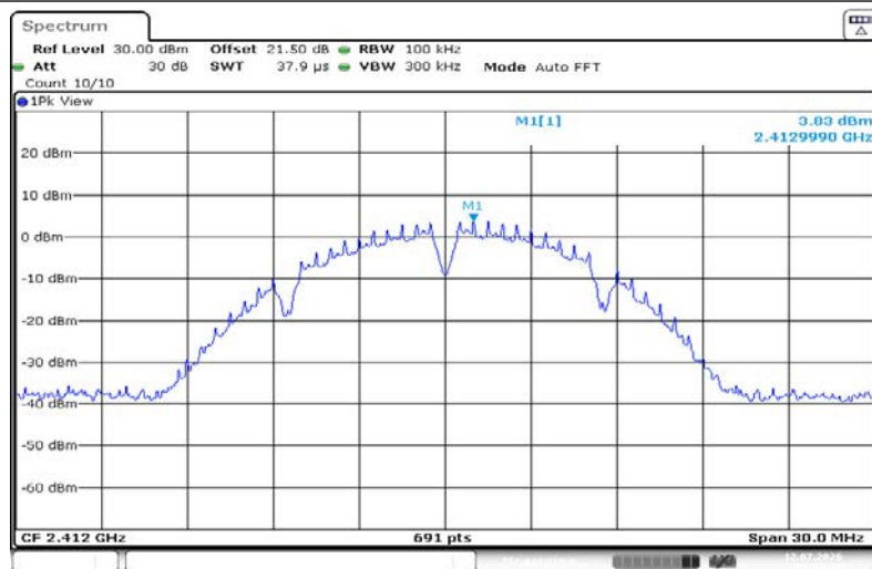
11B-Ant1-2412-0~Reference-PASS
