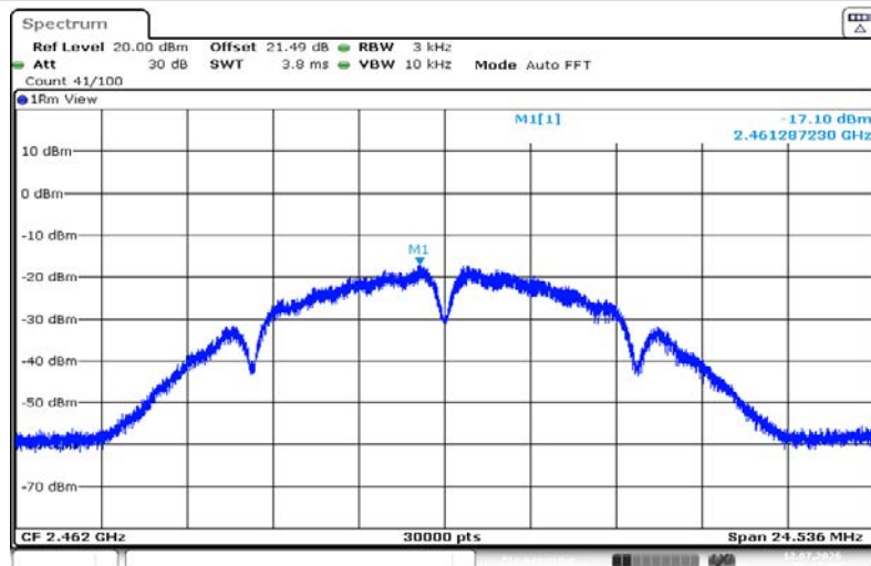
11B-Ant1-2462-PASS
