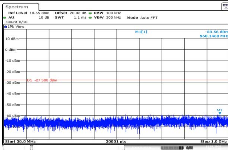
11N20SISO-Ant1-2462-30~1000-PASS
