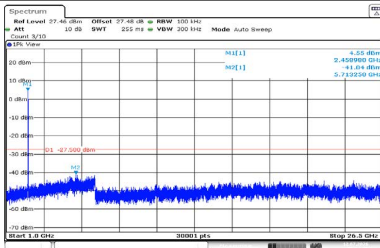
11N20SISO-Ant1-2462-1000~26500-PASS
