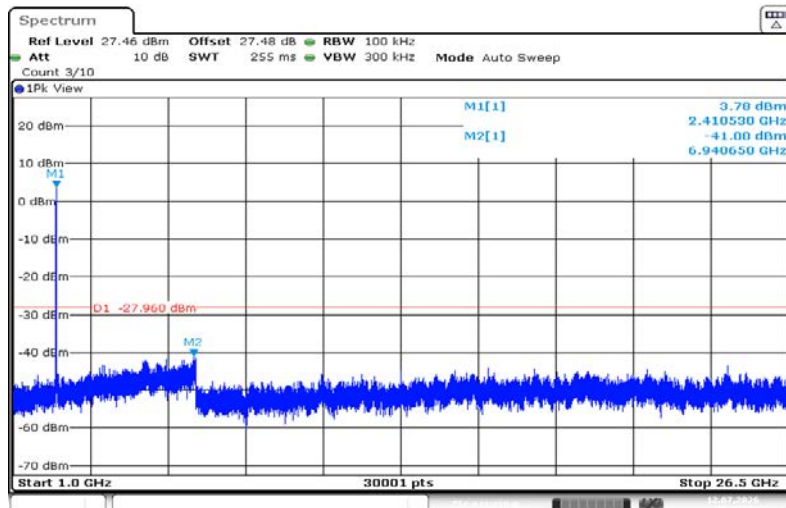
11N20SISO-Ant1-2412-1000~26500-PASS
