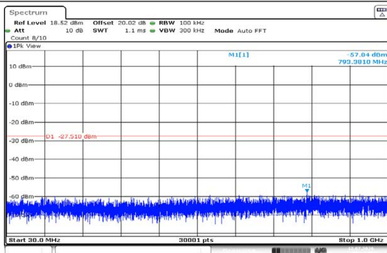
11G-Ant1-2412-0-Reference-PASS
