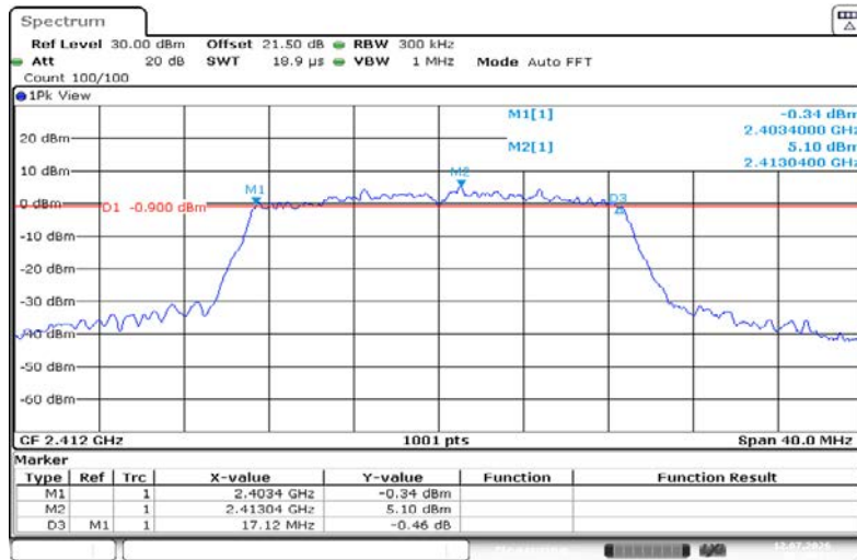
11N20SISO-Ant1-2412-PASS
