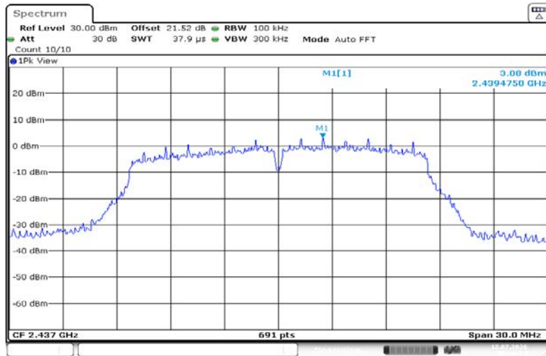
11G-Ant1-2437-0-Reference-PASS
