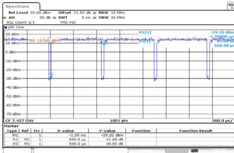
NTVN-11N40SISO-Ant1-2437
