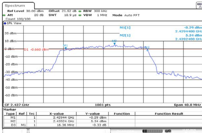
11N20SISO-Ant1-2437-PASS
