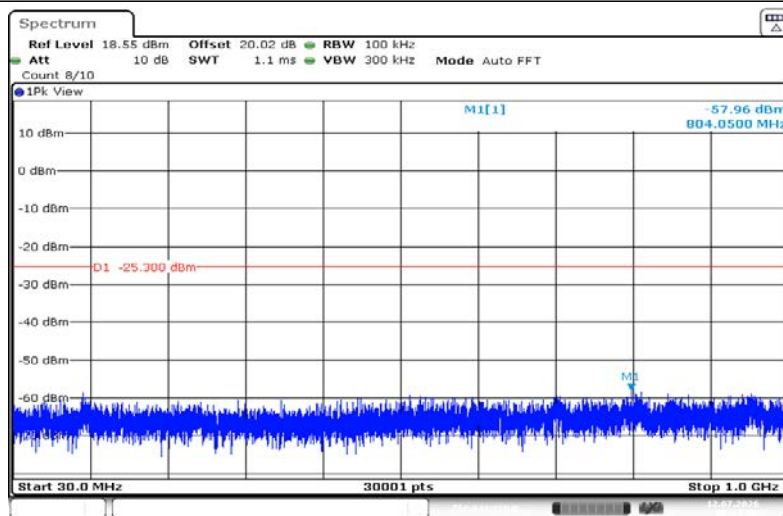
11B-Ant1-2462-30~1000-PASS
