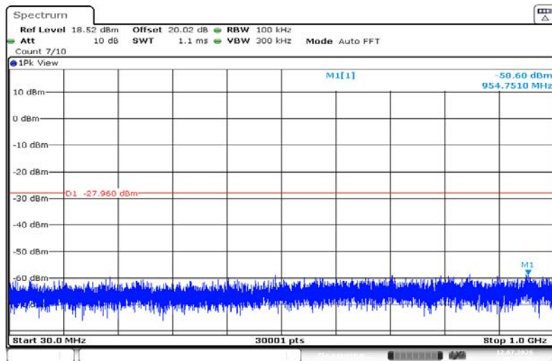
11N20SISO-Ant1-2412-30~1000-PASS
