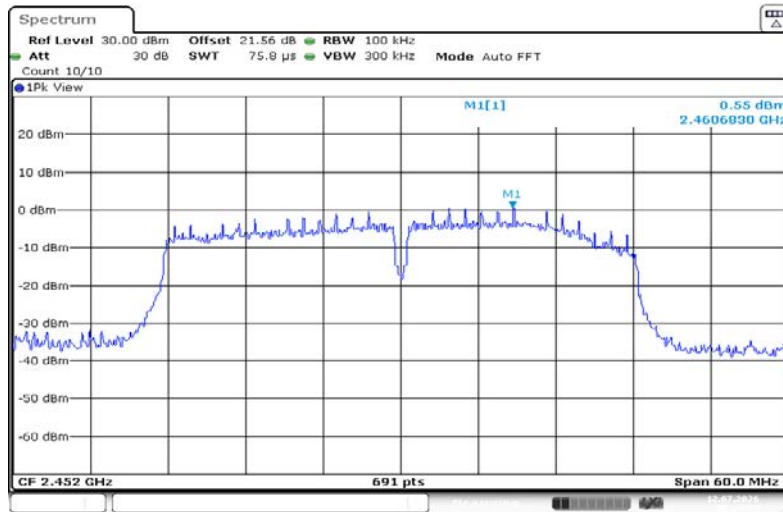
11N40SISO-Ant1-2452-0~Reference-PASS
