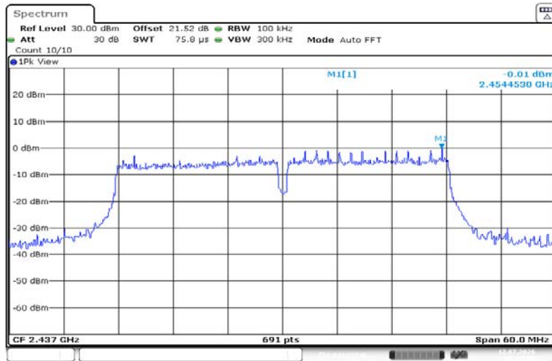
11N40SISO-Ant1-2437-0~Reference-PASS
