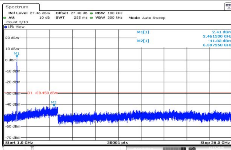
11N40SISO-Ant1-2452-1000~26500-PASS
