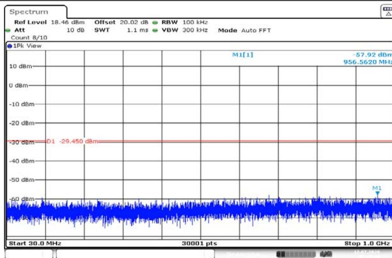
11N40SISO-Ant1-2452-30~1000-PASS
