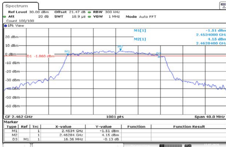
11N20SISO-Ant1-2462-PASS
