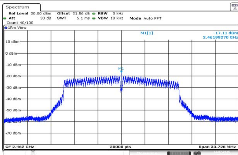
11G-Ant1-2462-PASS
