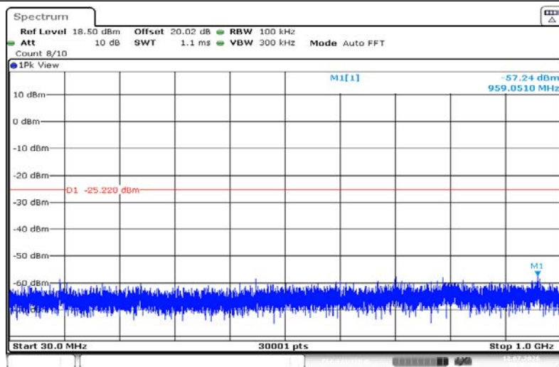
11B-Ant1-2437-30~1000-PASS
