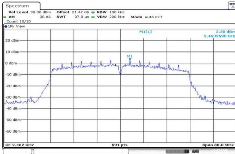
11N20SISO-Ant1-2462-0~Reference-PASS
