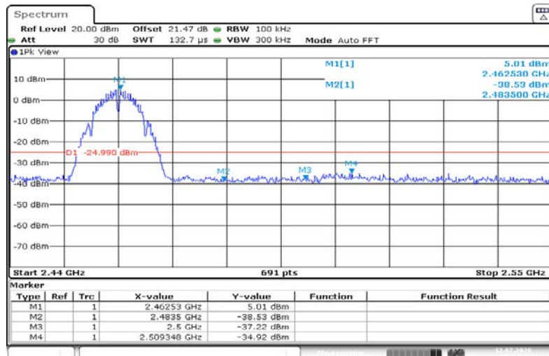
11B-Ant1-2462-PASS
