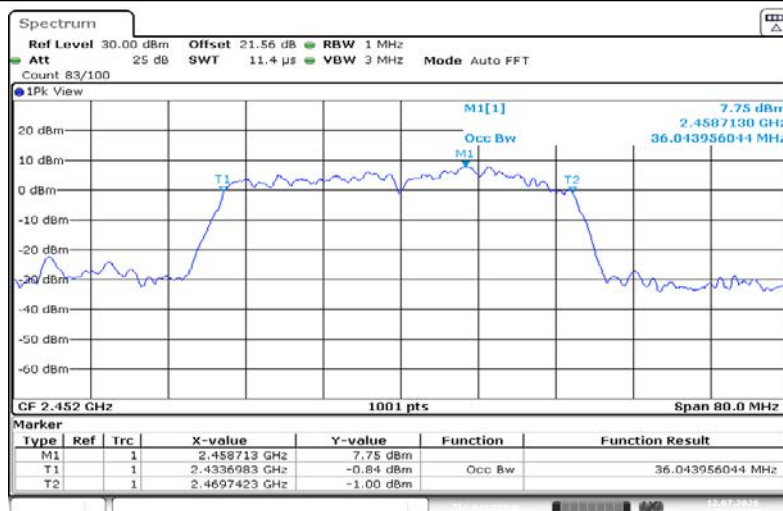
11N40SISO-Ant1-2452
