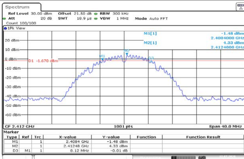
11B-Ant1-2412-PASS
