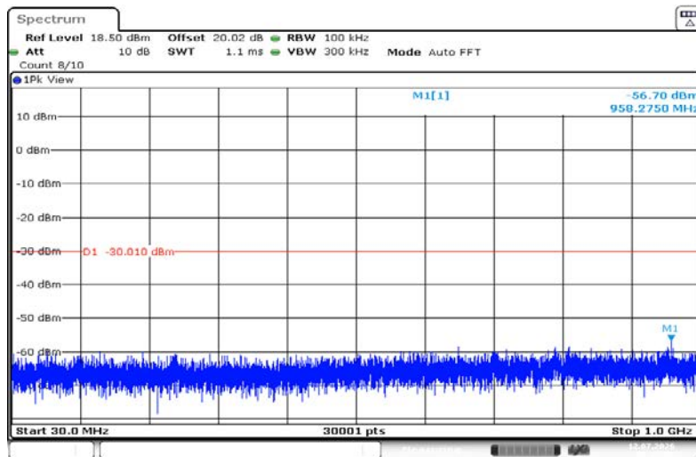
11N40SISO-Ant1-2437-30~1000-PASS
