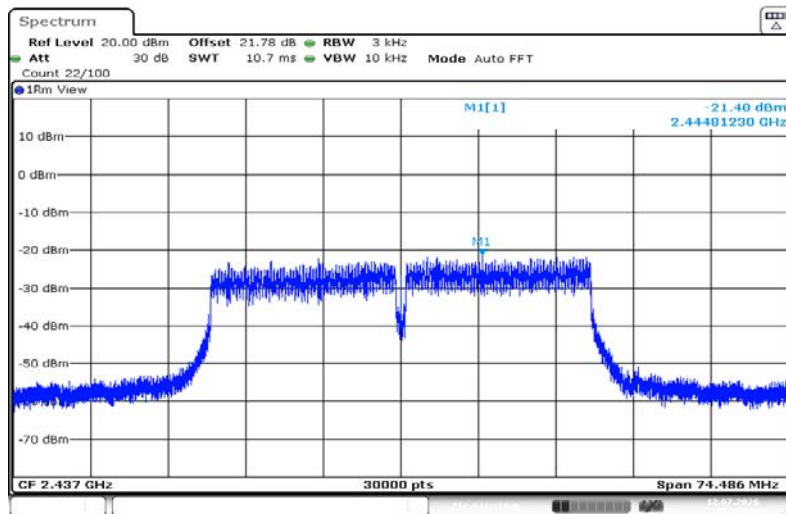
11N40SISO-Ant1-2437-PASS
