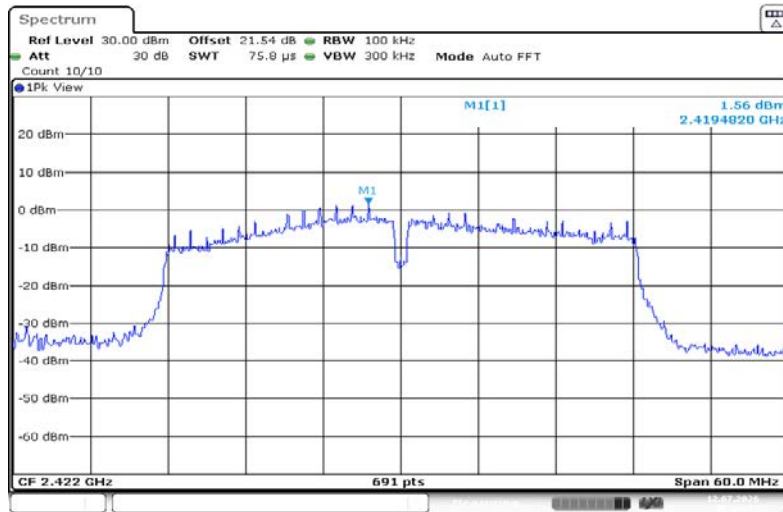
11N40SISO-Ant1-2422-0~Reference-PASS
