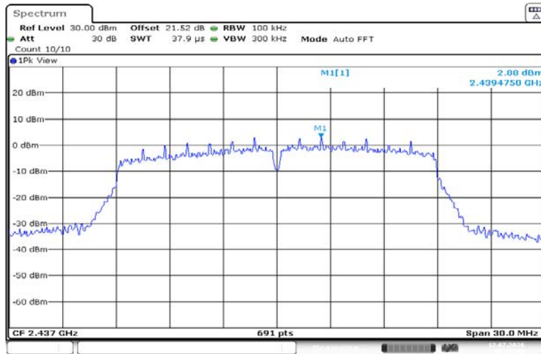
11N20SISO-Ant1-2437-0~Reference-PASS
