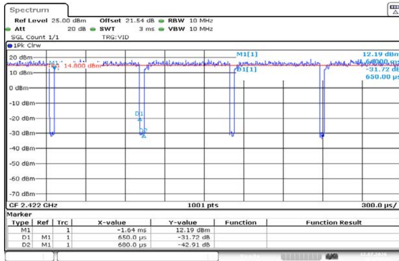
NTVN-11N40SISO-Ant1-2422
