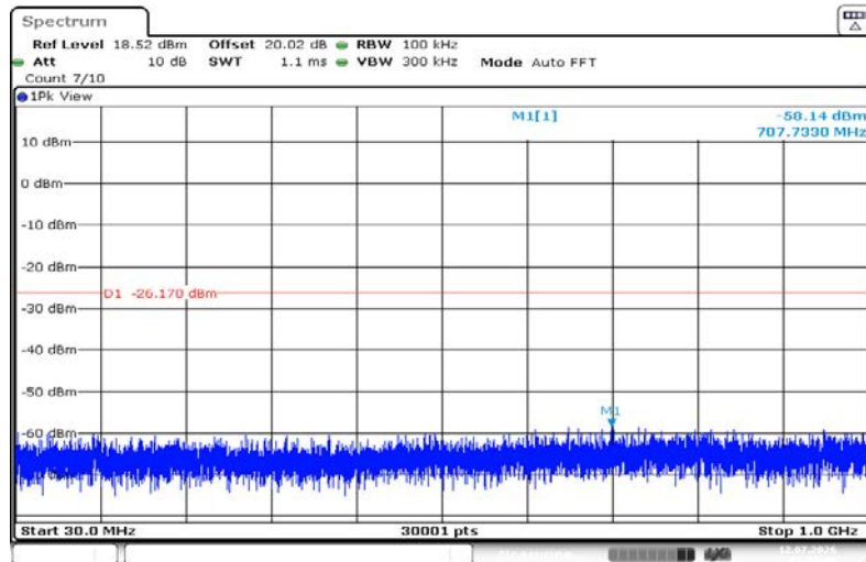
11B-Ant1-2412-30~1000-PASS
