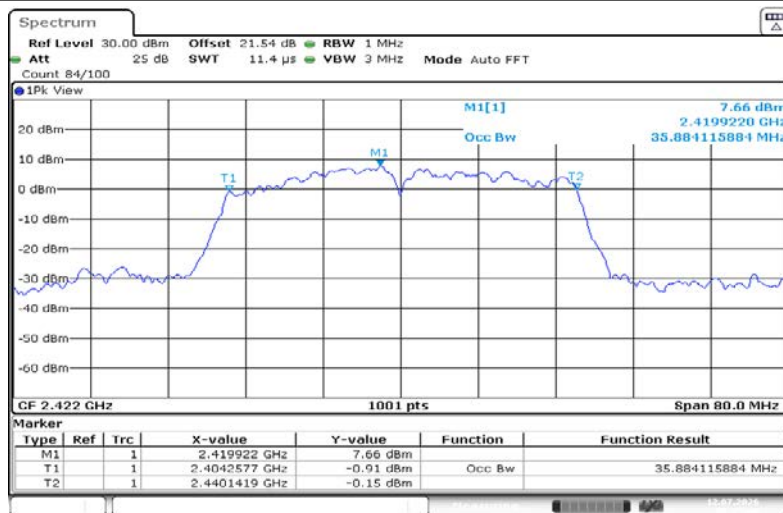
11N40SISO-Ant1-2422
