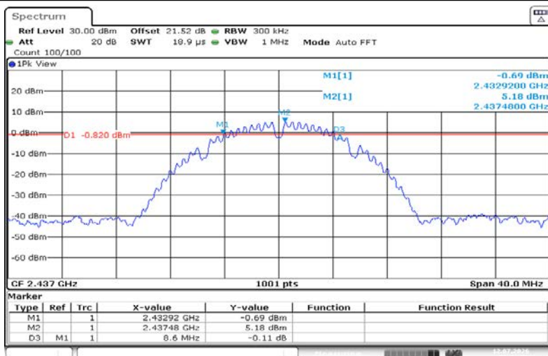
11B-Ant1-2437-PASS
