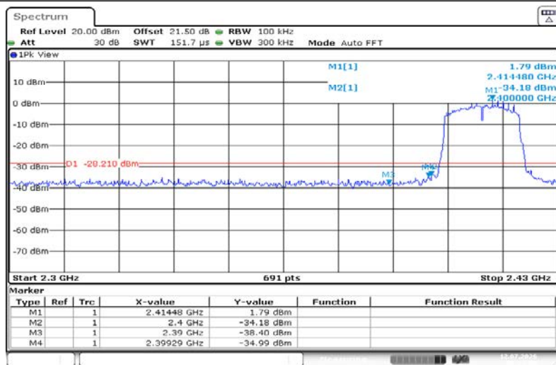
11N20SISO-Ant1-2412-PASS
