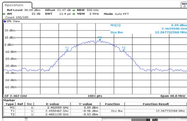
11B-Ant1-2462
