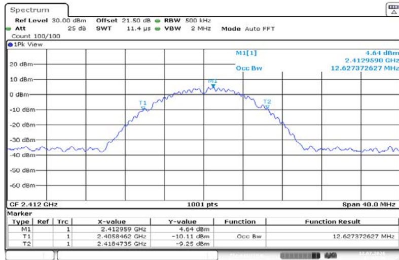
11B-Ant1-2412
