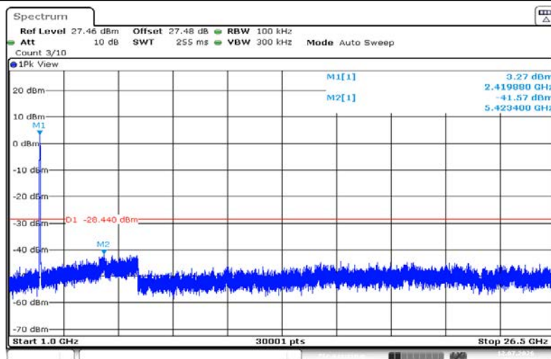
11N40SISO-Ant1-2422-1000~26500-PASS
