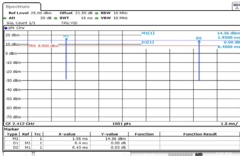
NTNV-11B-Ant1-2412
