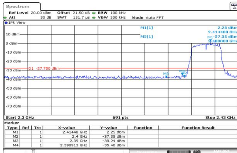
11G-Ant1-2412-PASS
