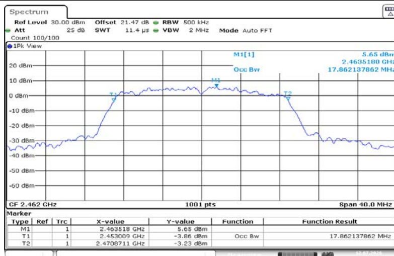
11N20SISO-Ant1-2462
