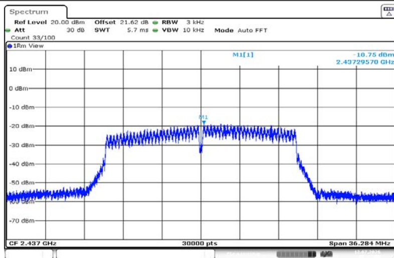
11N20SISO-Ant1-2437-PASS
