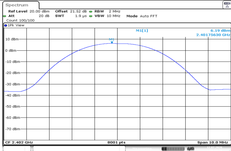
BLE_1M_Ant1_2440
