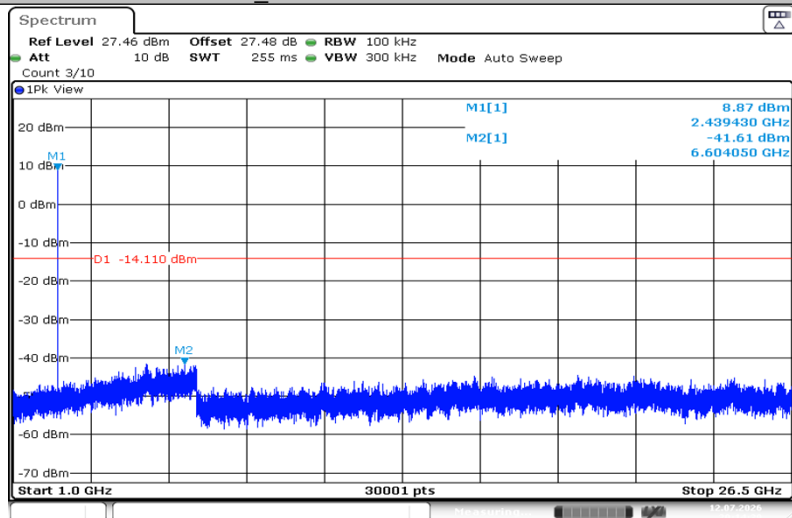
BLE_1M-Ant1-2440-1000~26500-PASS
