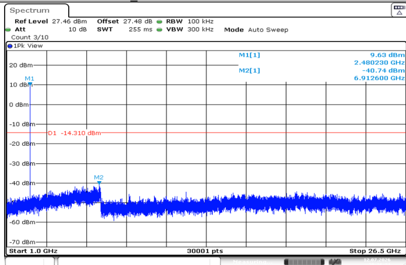
BLE_1M-Ant1-2480-1000~26500-PASS
