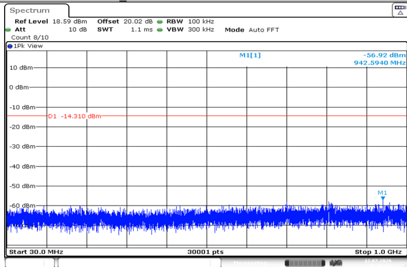
BLE_1M-Ant1-2480-30~1000-PASS
