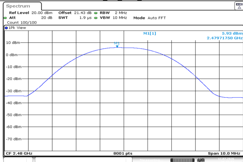
BLE_1M_Ant1_2480
