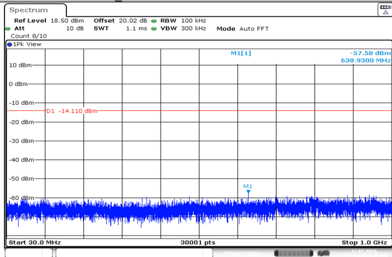
BLE_1M-Ant1-2440-30~1000-PASS
