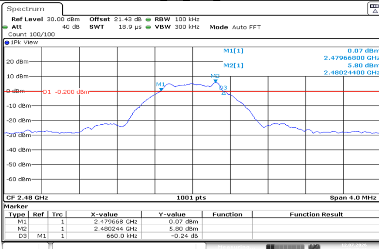
BLE_1M_Ant1_2480
