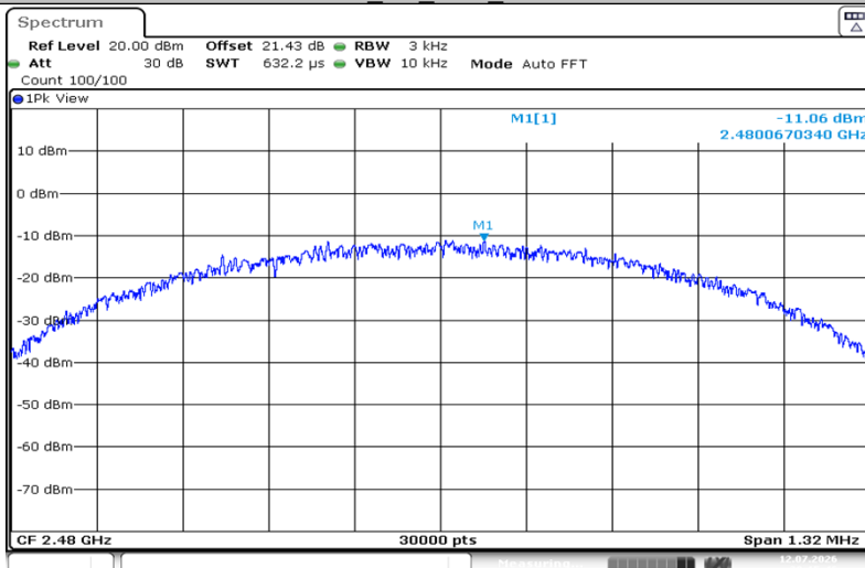
BLE_1M_Ant1_2480
