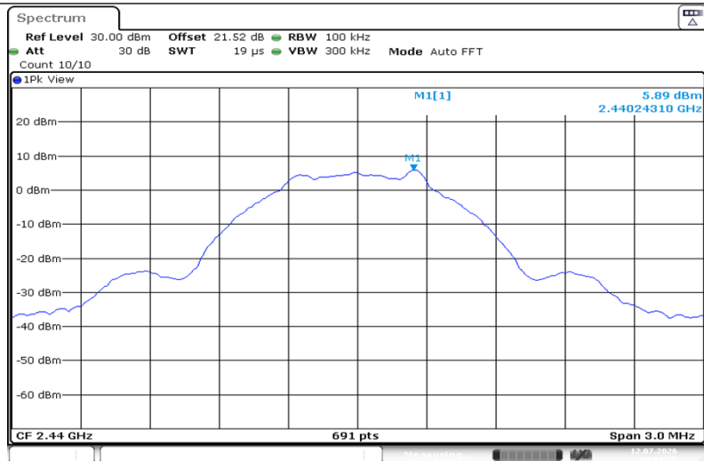
BLE_1M-Ant1-2440-0~Reference-PASS
