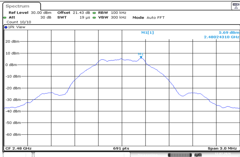
BLE_1M-Ant1-2480-0~Reference-PASS
