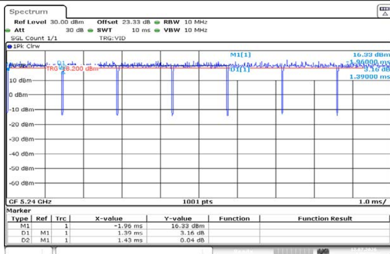
NTNV-11A-Ant1-5240
