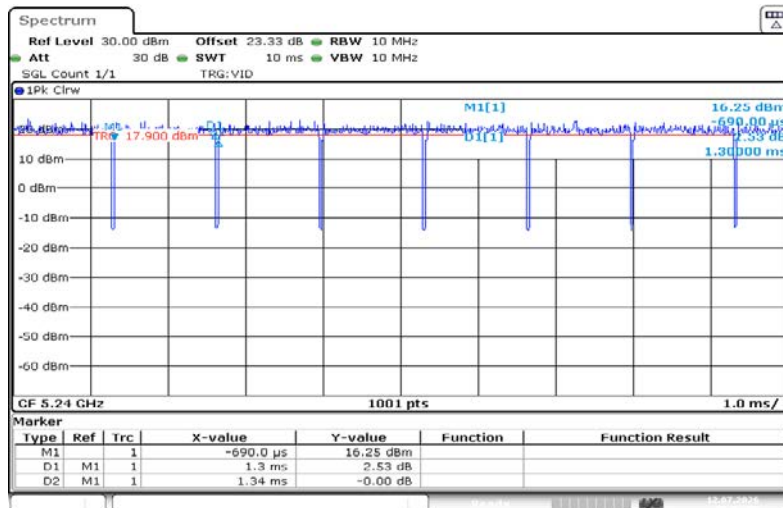
NTNV-11N20SISO-Ant1-5240
