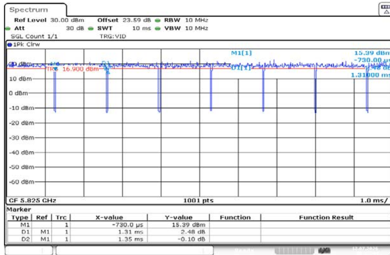
NTNV-11AC20SISO-Ant1-5825
