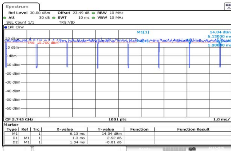
NTNV-11N20SISO-Ant1-5745
