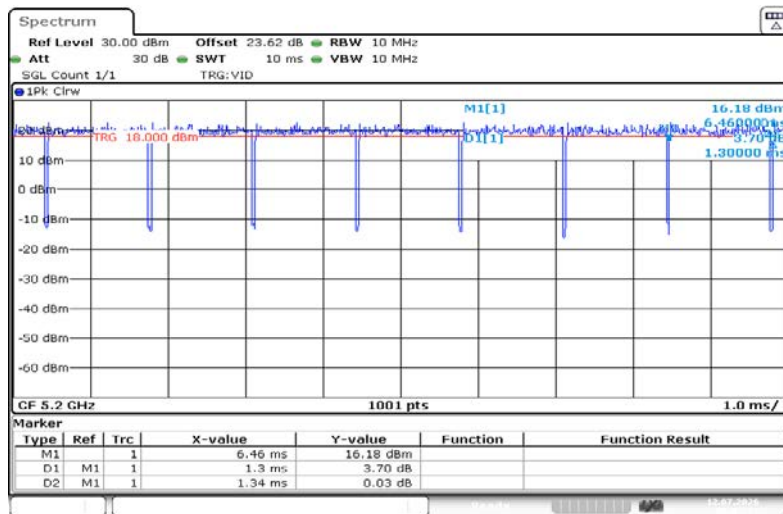
NTNV-11N20SISO-Ant1-5200
