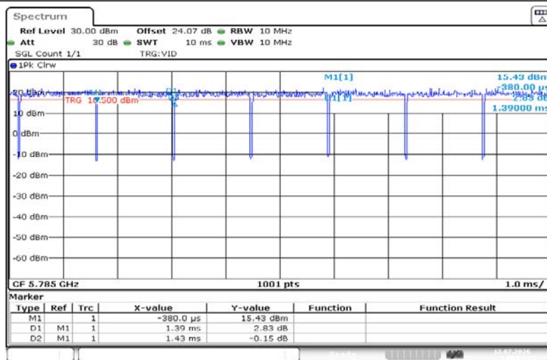
NTNV-11A-Ant1-5785
