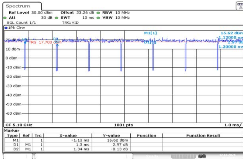
NTNV-11N20SISO-Ant1-5180
