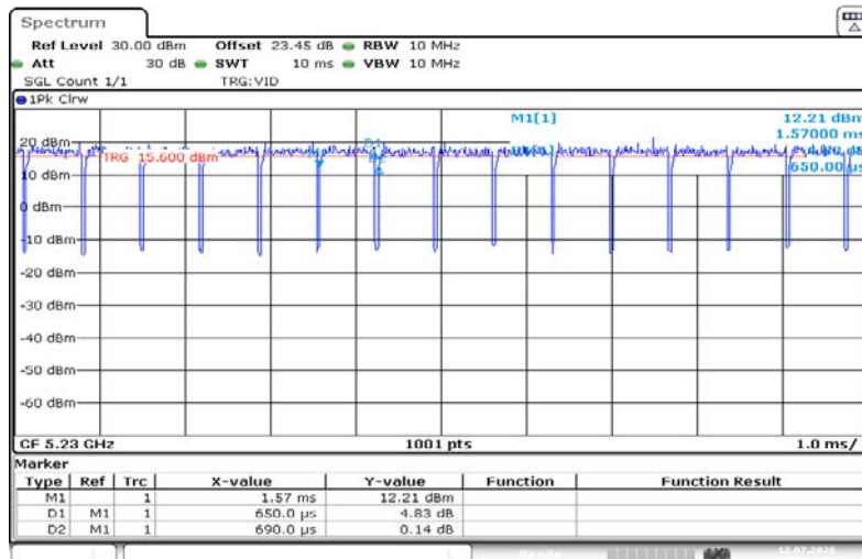
NTNV-11AC40SISO-Ant1-5230
