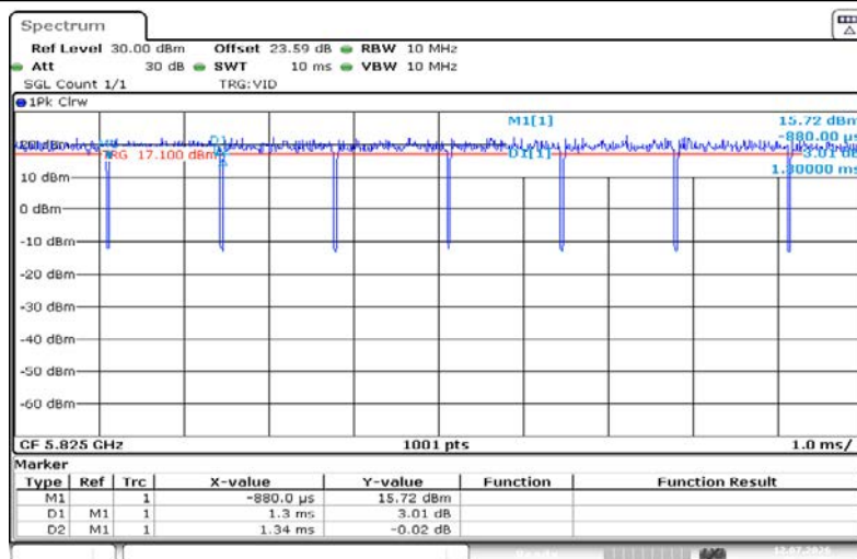
NTNV-11N20SISO-Ant1-5825
