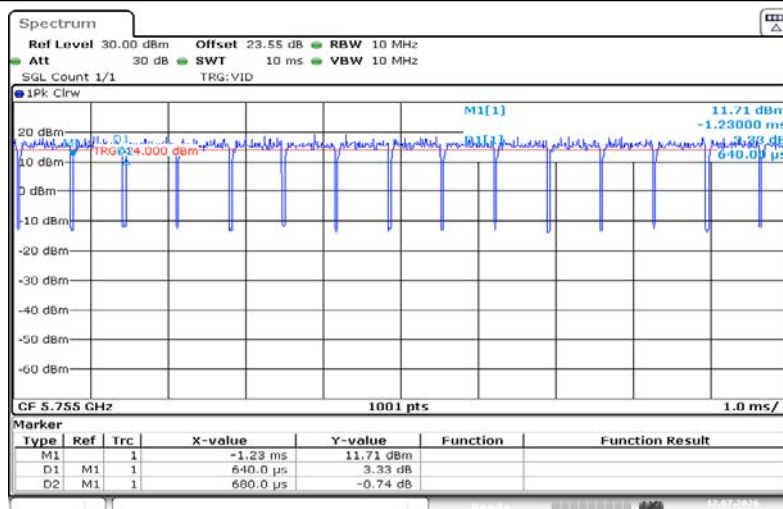
NTNV-11N40SISO-Ant1-5755
