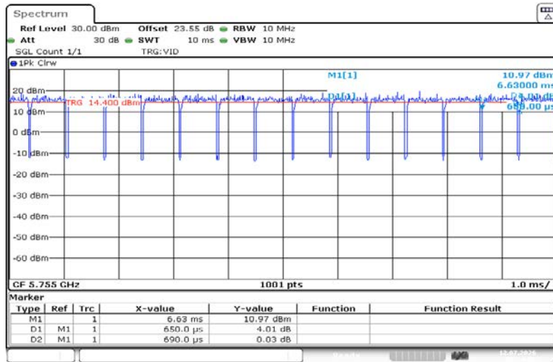
NTNV-11AC40SISO-Ant1-5755
