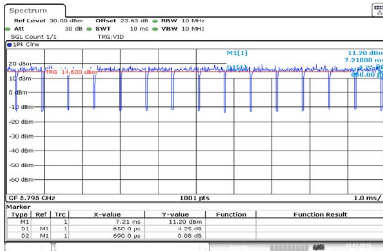
NTNV-11AC40SISO-Ant1-5795
