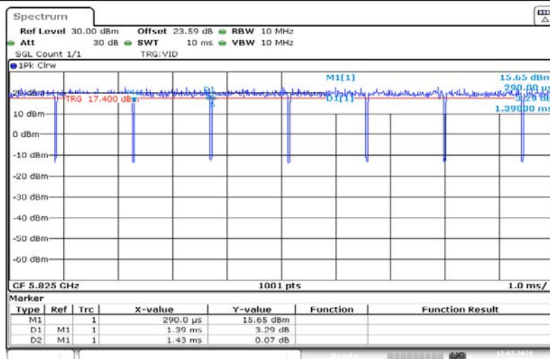
NTNV-11A-Ant1-5825
