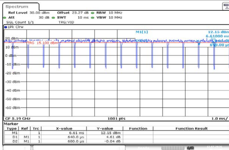
NTNV-11N40SISO-Ant1-5190
