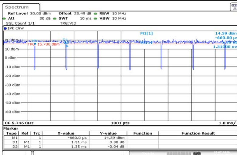
NTNV-11AC20SISO-Ant1-5745
