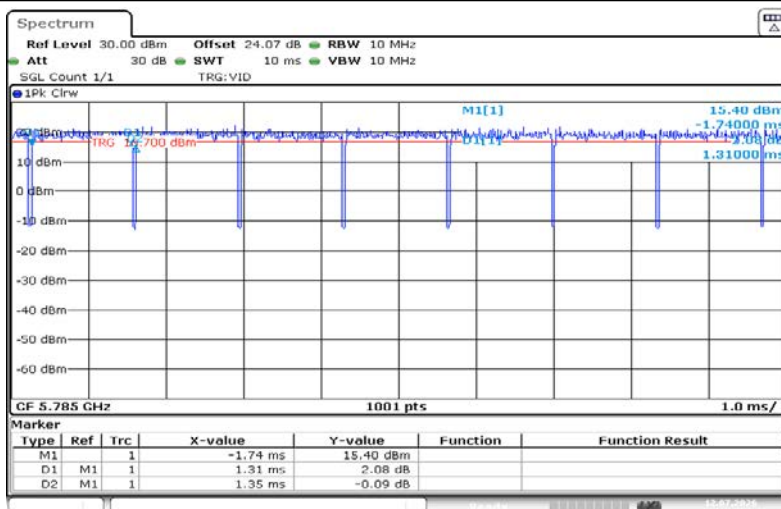
NTNV-11AC20SISO-Ant1-5785
