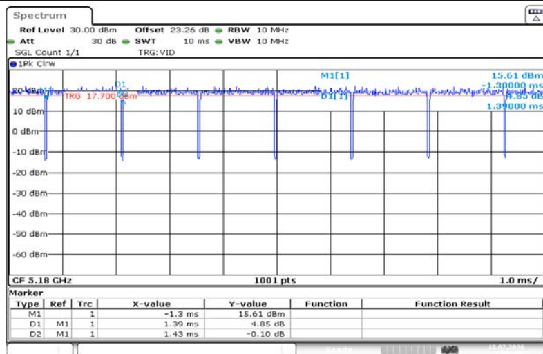
NTNV-11A-Ant1-5180
