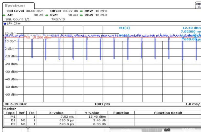
NTNV-11AC40SISO-Ant1-5190
