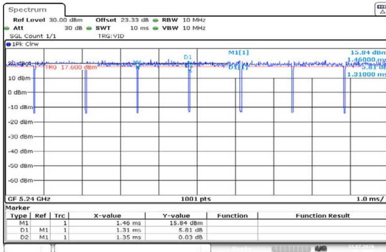
NTNV-11AC20SISO-Ant1-5240
