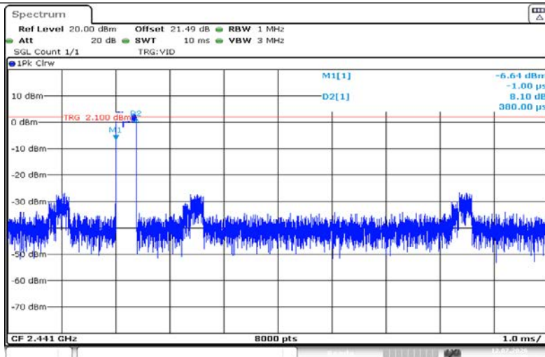
3DH1-Ant1-Hop-PASS
