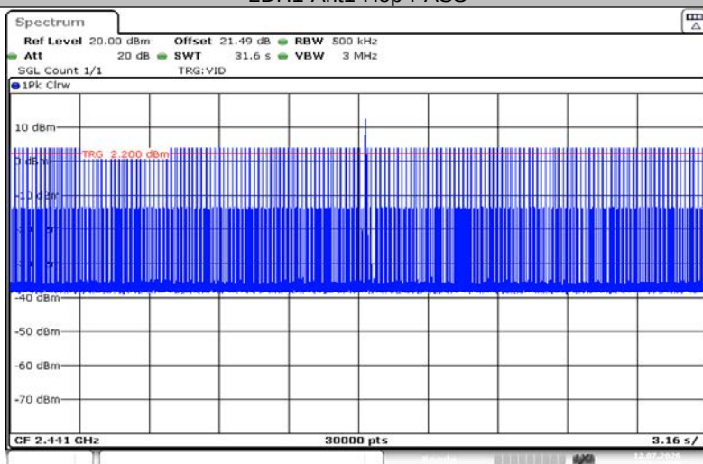
2DH1-Ant1-Hop-PASS
