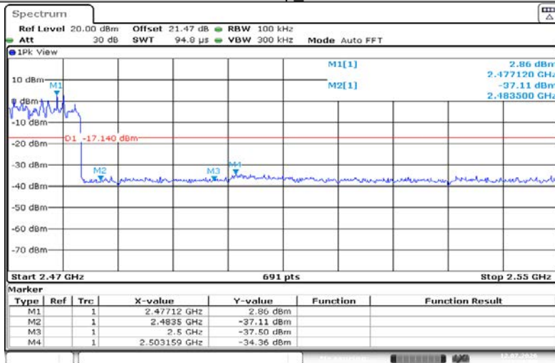
3DH5-Ant1-Hop_2480-PASS
