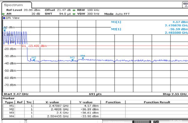
DH5-Ant1-Hop_2480-PASS
