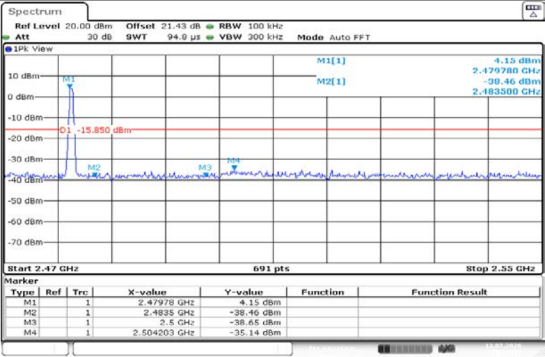
DH5-Ant1-2480-PASS
