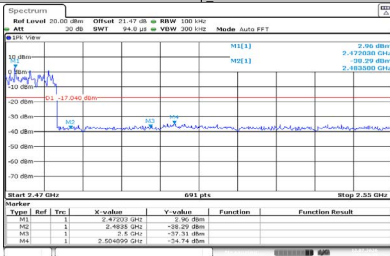
2DH5-Ant1-Hop_2480-PASS
