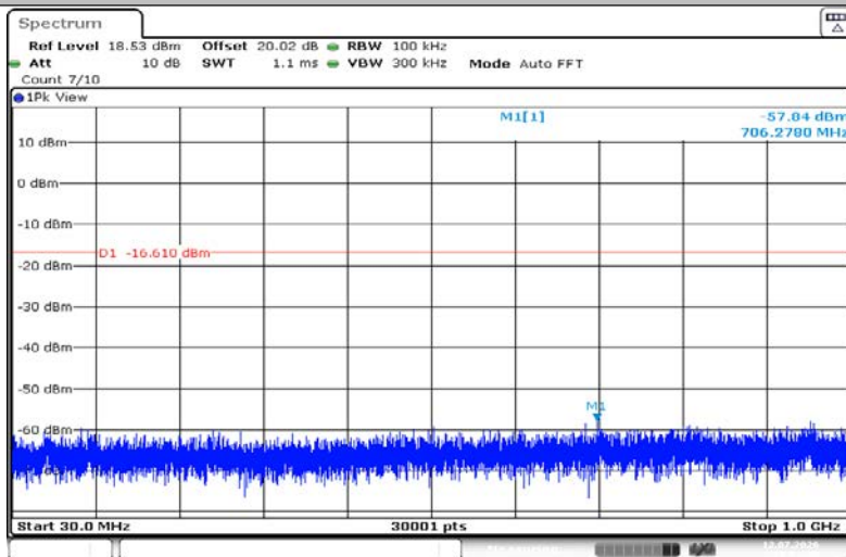
3DH5-Ant1-2441-30~1000-PASS
