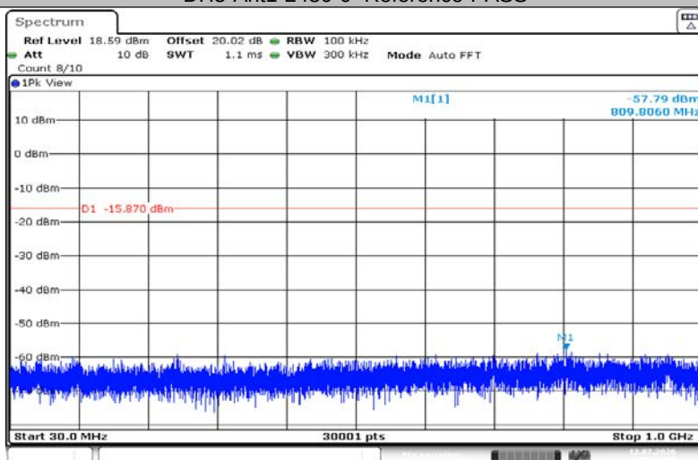
DH5-Ant1-2480-30~1000-PASS
