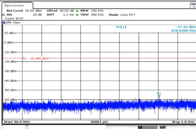
2DH5-Ant1-2480-30~1000-PASS
