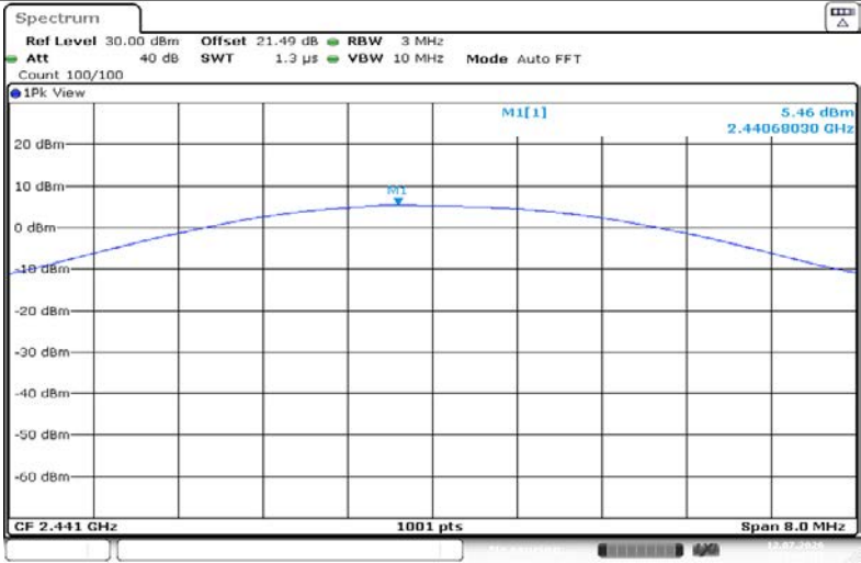
DH5-Ant1-2441-PASS
