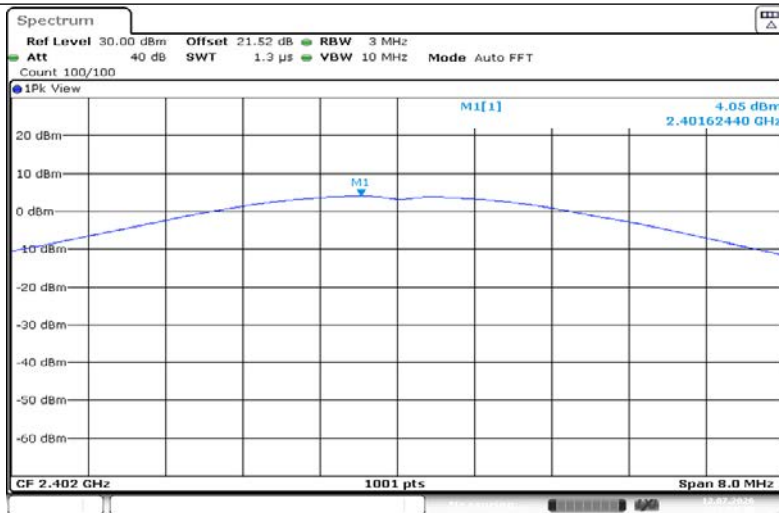
2DH5-Ant1-2402-PASS
