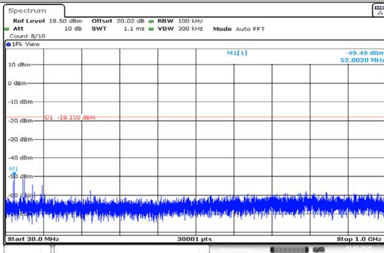
3DH5-Ant1-2402-30~1000-PASS
