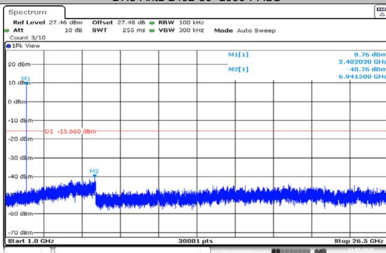
DH5-Ant1-2402-1000~26500-PASS
