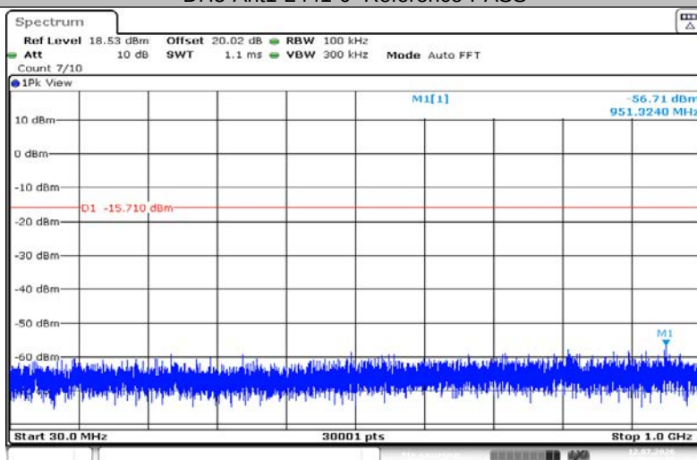
DH5-Ant1-2441-30~1000-PASS
