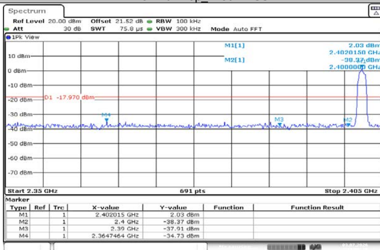
3DH5-Ant1-2402-PASS
