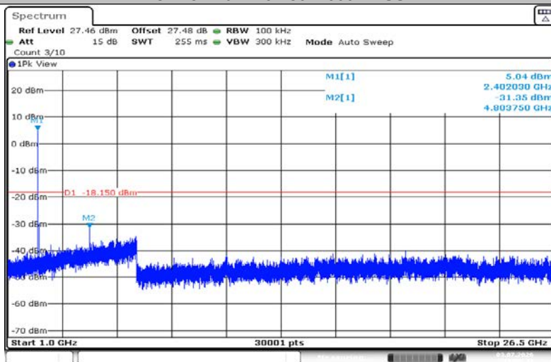
3DH5-Ant1-2402-1000~26500-PASS
