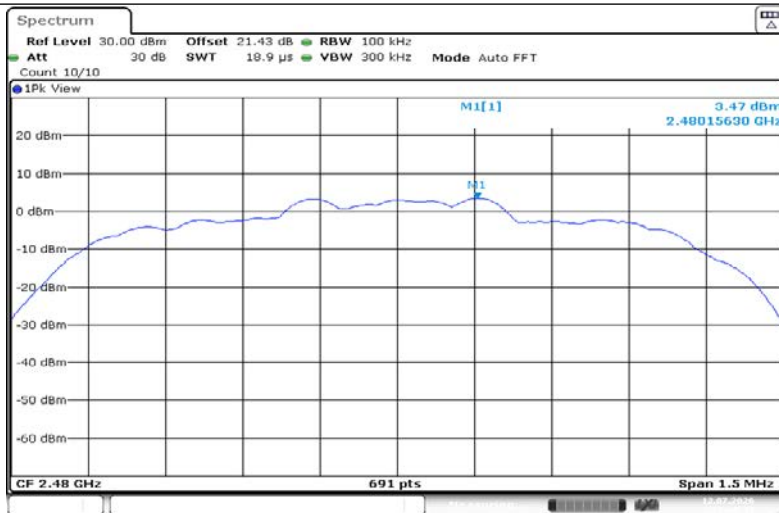
3DH5-Ant1-2480-0~Reference-PASS
