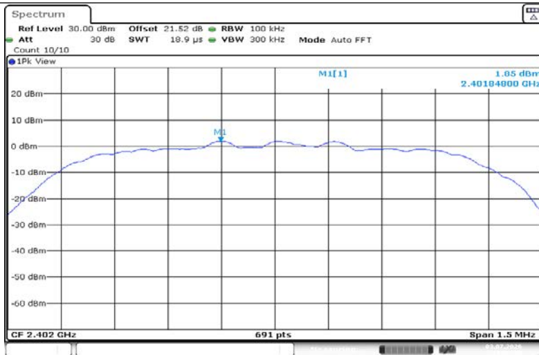
3DH5-Ant1-2402-0~Reference-PASS
