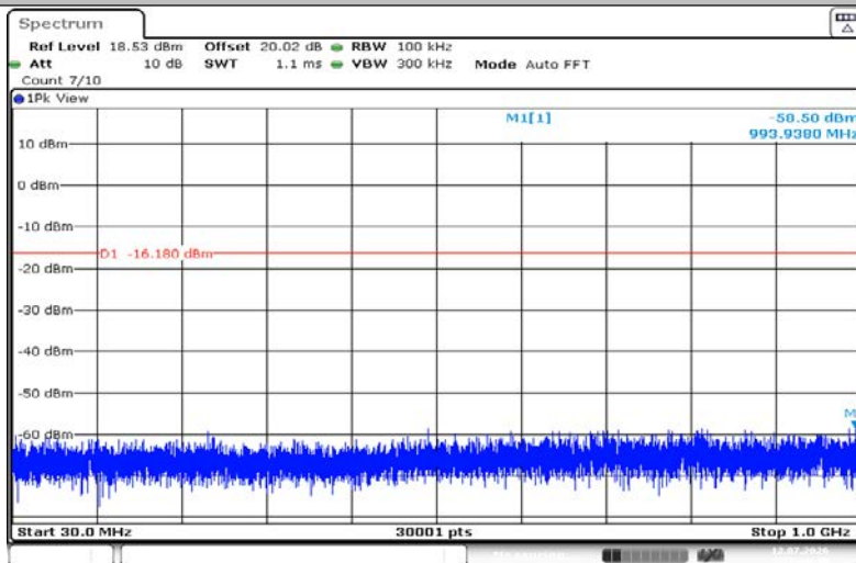
2DH5-Ant1-2441-30~1000-PASS
