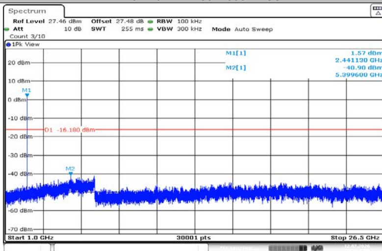
2DH5-Ant1-2441-1000~26500-PASS
