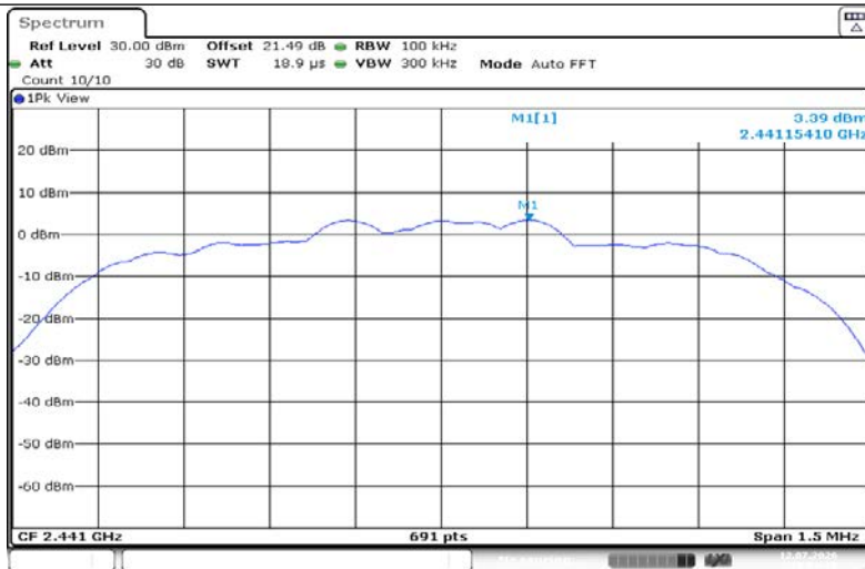
3DH5-Ant1-2441-0~Reference-PASS
