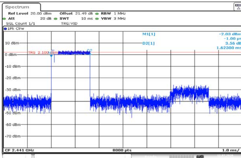
3DH3-Ant1-Hop-PASS
