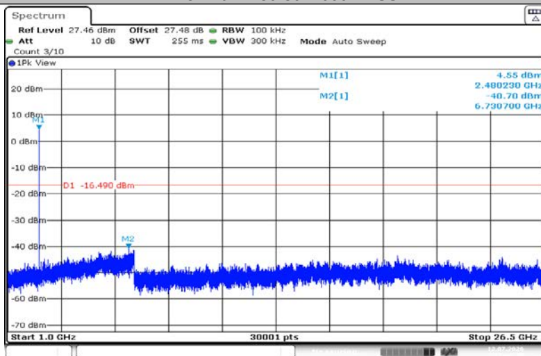
2DH5-Ant1-2480-1000~26500-PASS
