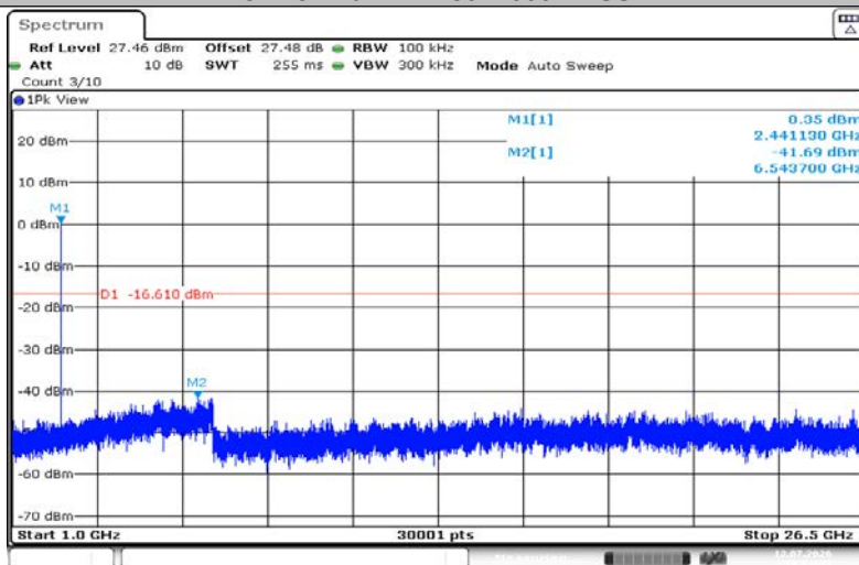
3DH5-Ant1-2441-1000~26500-PASS
