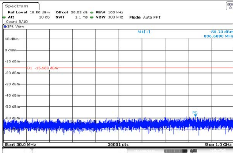
DH5-Ant1-2402-30~1000-PASS
