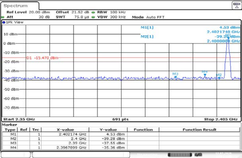
DH5-Ant1-2402-PASS
