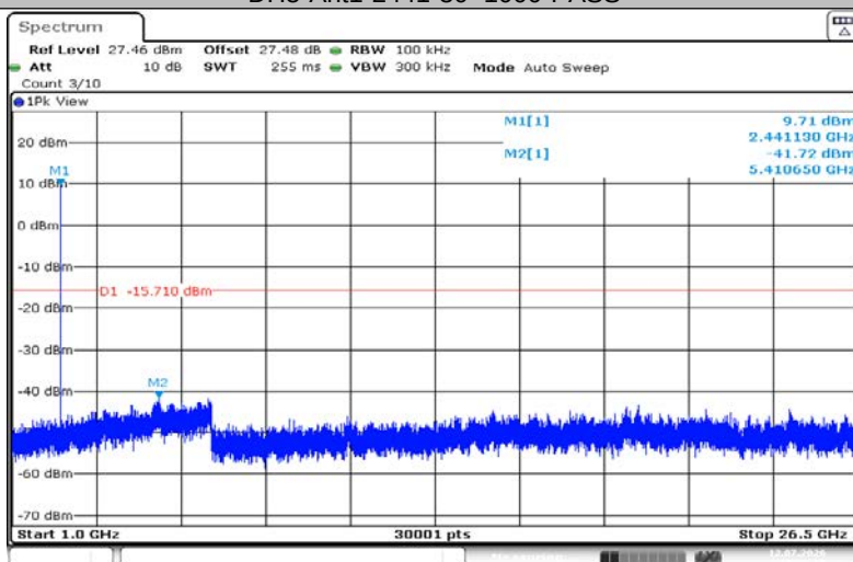
DH5-Ant1-2441-1000~26500-PASS
