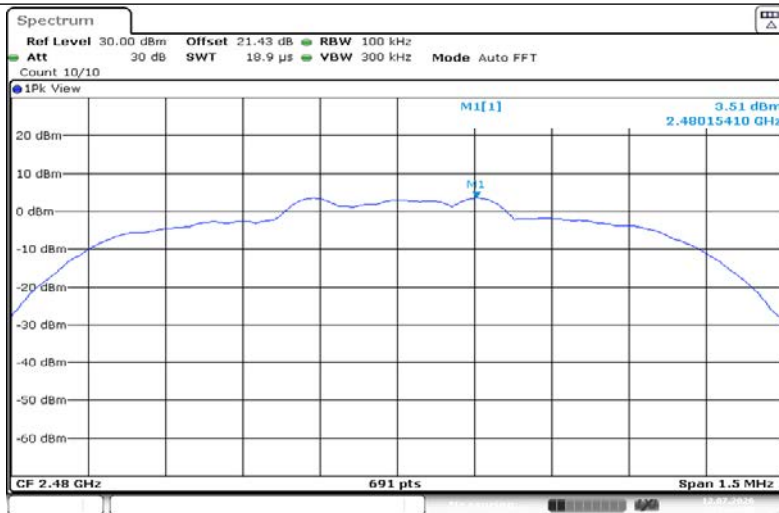
2DH5-Ant1-2480-0~Reference-PASS
