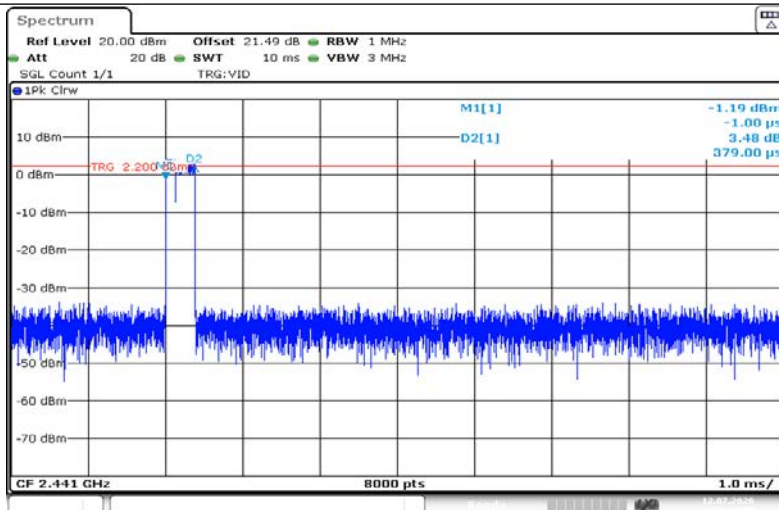
2DH1-Ant1-Hop-PASS
