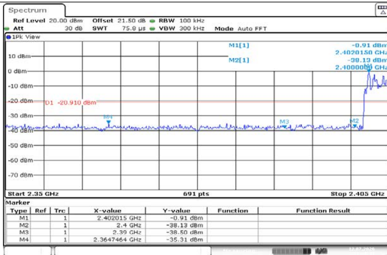
2DH5-Ant1-Hop_2402-PASS
