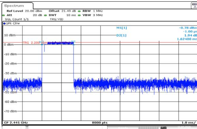
2DH3-Ant1-Hop-PASS
