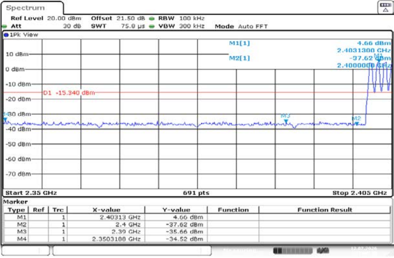
DH5-Ant1-Hop_2402-PASS
