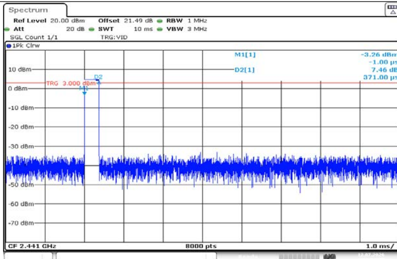
DH1-Ant1-Hop-PASS
