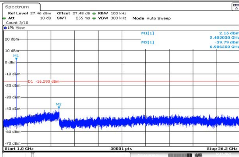
2DH5-Ant1-2402-1000~26500-PASS
