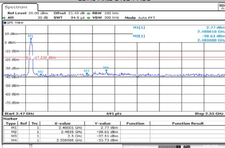
2DH5-Ant1-2480-PASS
