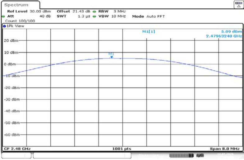
DH5-Ant1-2480-PASS
