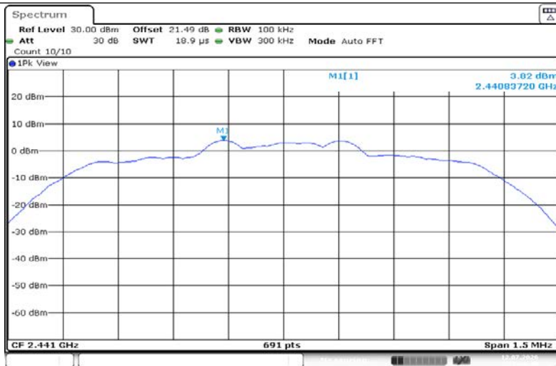
2DH5-Ant1-2441-0~Reference-PASS
