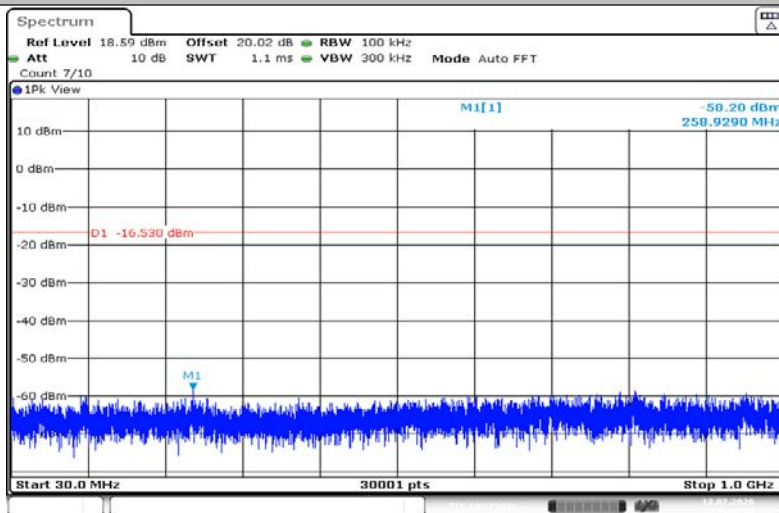
3DH5-Ant1-2480-30~1000-PASS
