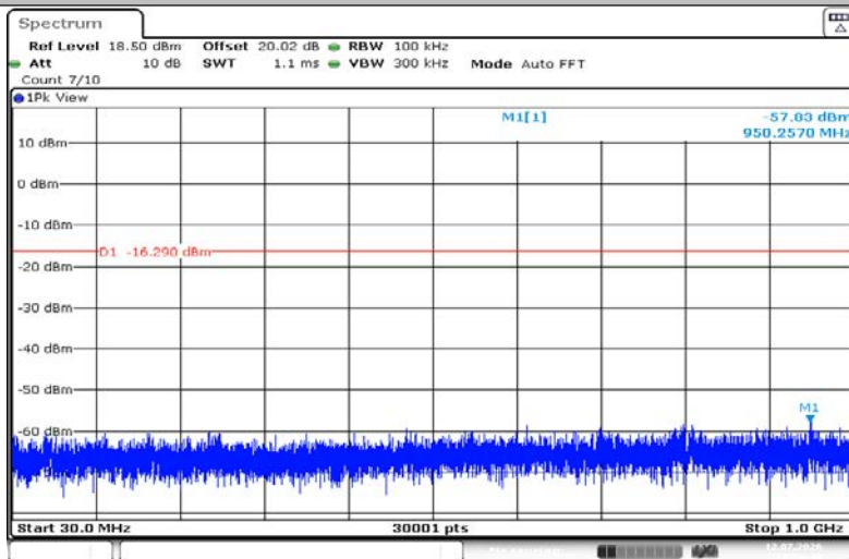
2DH5-Ant1-2402-30~1000-PASS
