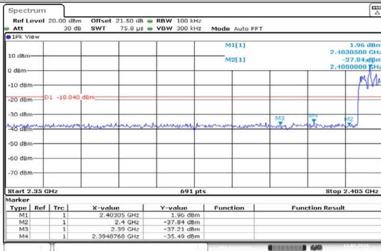
3DH5-Ant1-Hop_2402-PASS
