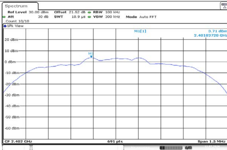
2DH5-Ant1-2402-0~Reference-PASS
