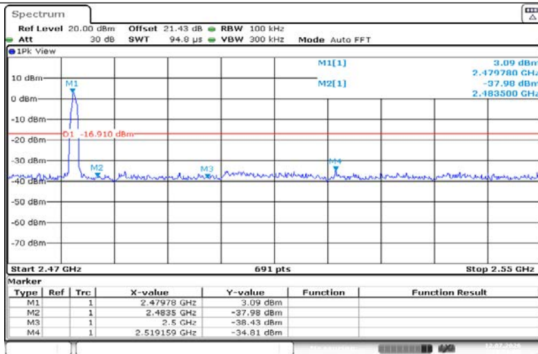
3DH5-Ant1-2480-PASS
