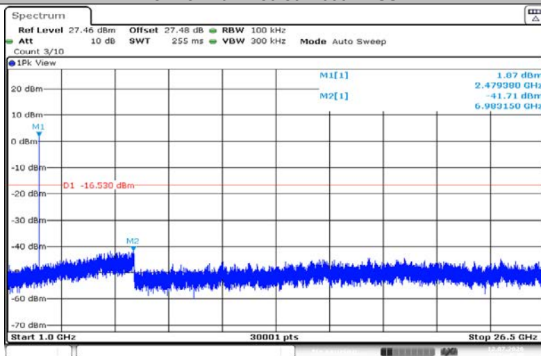
3DH5-Ant1-2480-1000~26500-PASS
