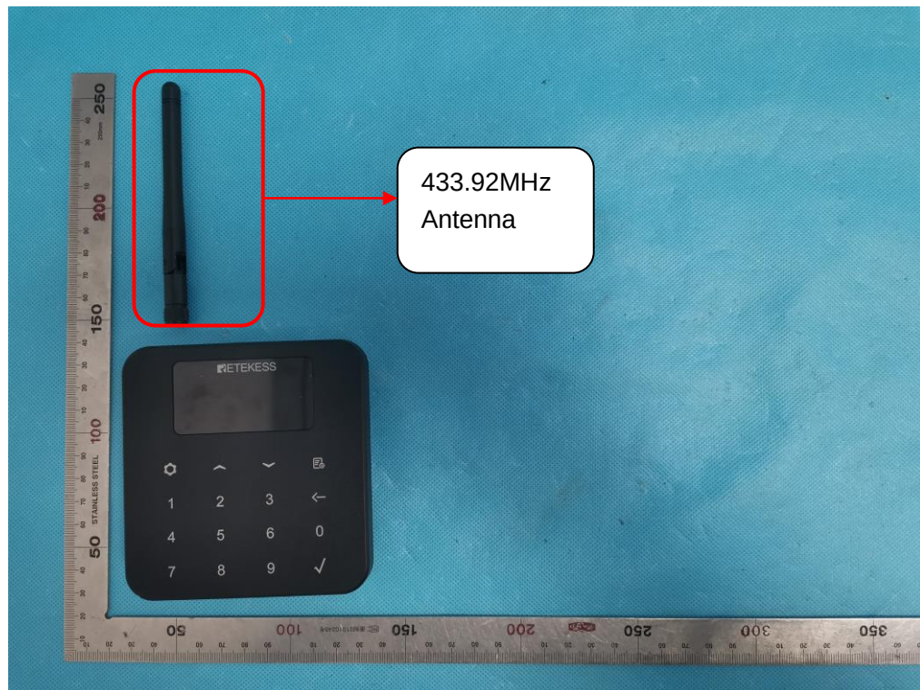
Antenna of EUT
