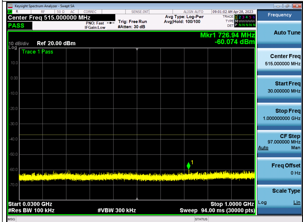
Test_Graph_802.11ax80_ANT1_5210_MCS9_Frequency Band 1
