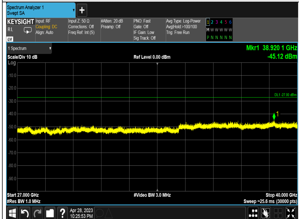
Test_Graph_802.11a_ANT2_5240_6Mbps_Frequency Band 5
