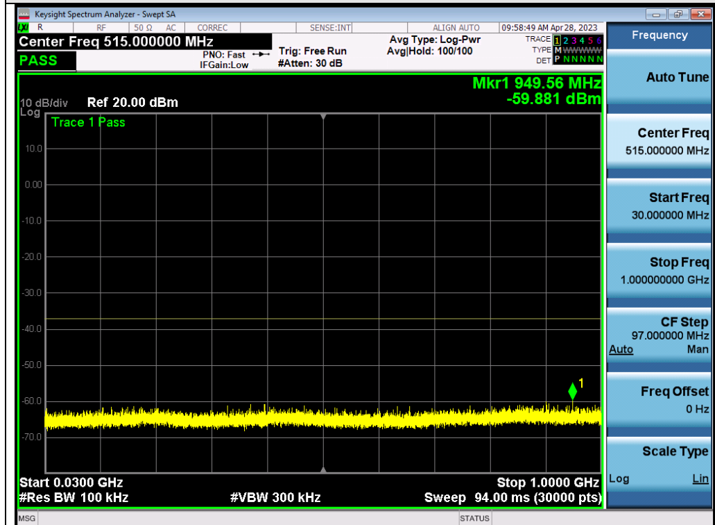
Test_Graph_802.11ax80_ANT2_5210_MCS9_Frequency Band 1
