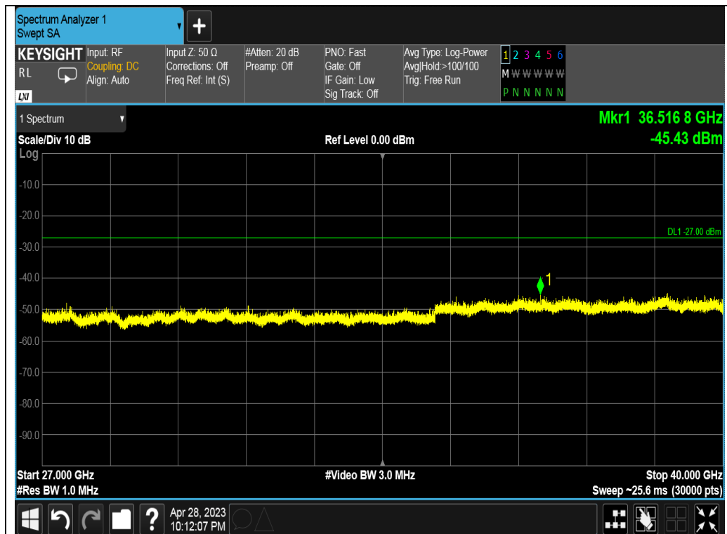
Test_Graph_802.11ac80_ANT1_5775_MCS9_Frequency Band5
