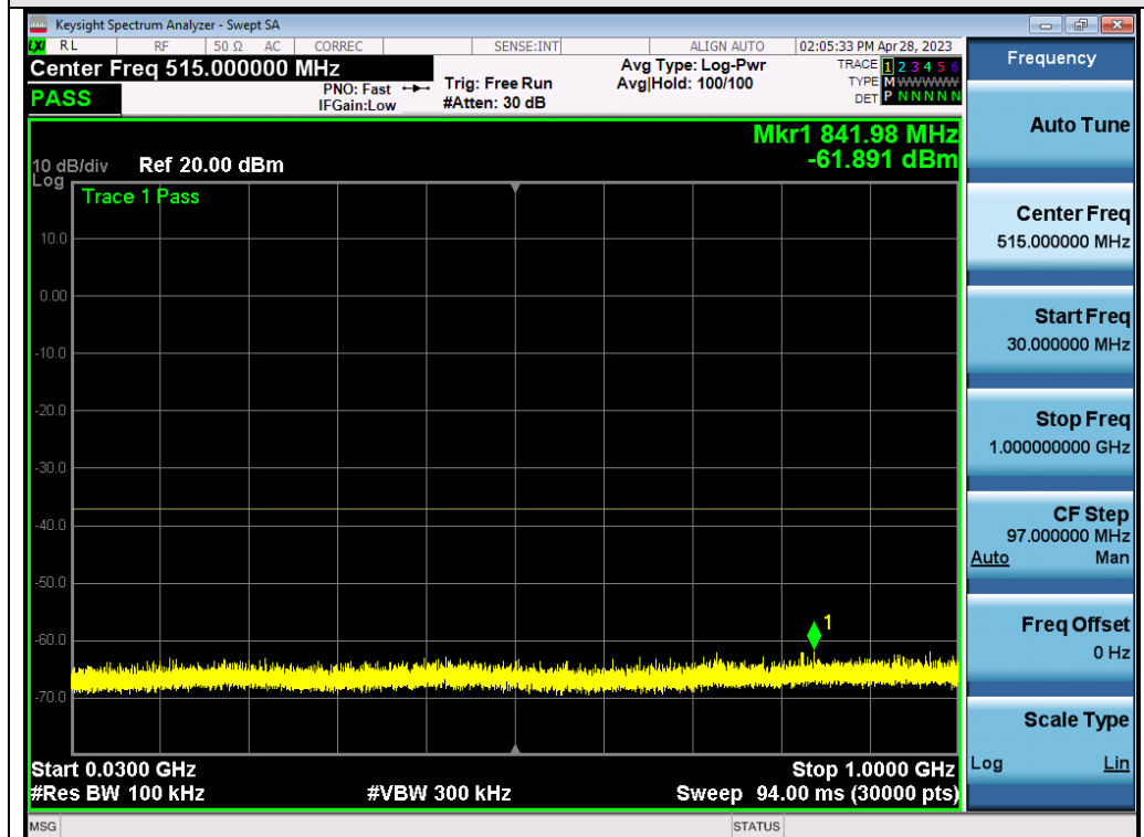
Test_Graph_802.11ax80_ANT1_5775_MCS9_Frequency Band1
