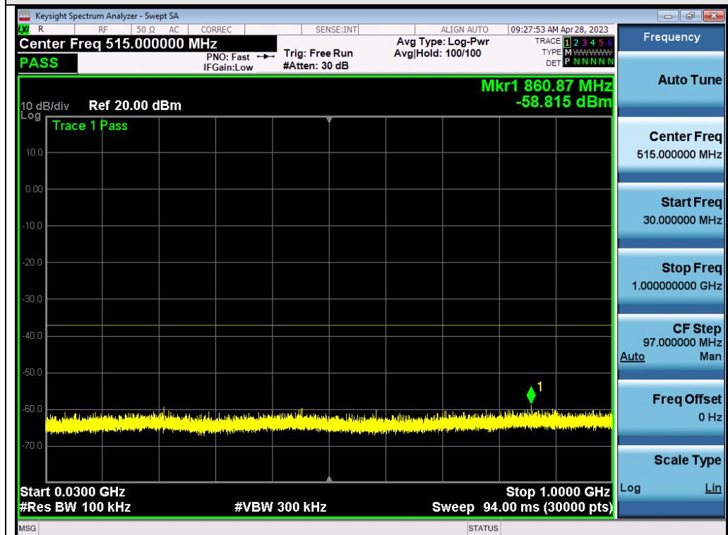
Test_Graph_802.11n40_ANT2_5230_MCS0_Frequency Band 1
