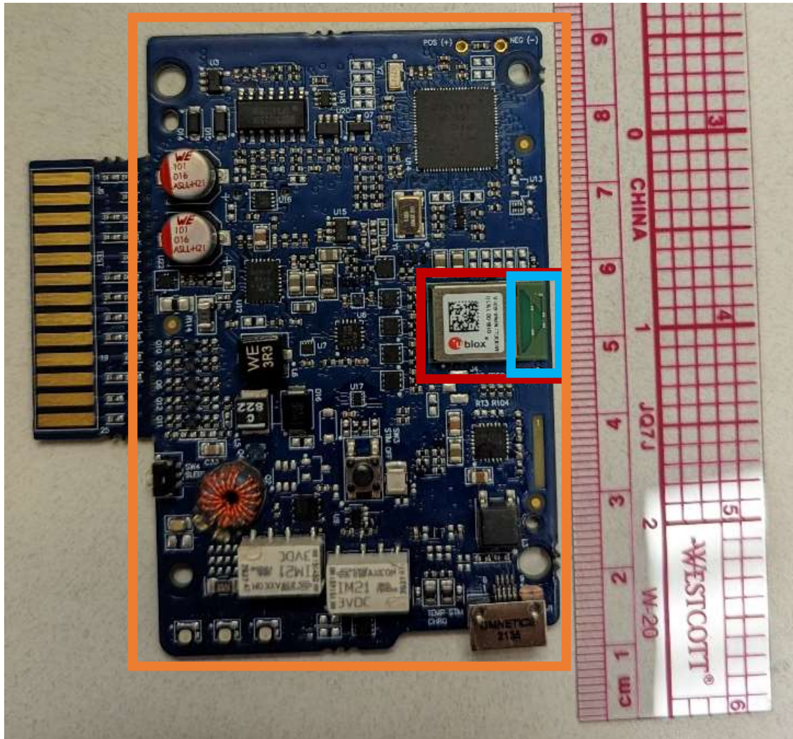
NINA-B3x6 with internal antenna on Charger host board – top view
