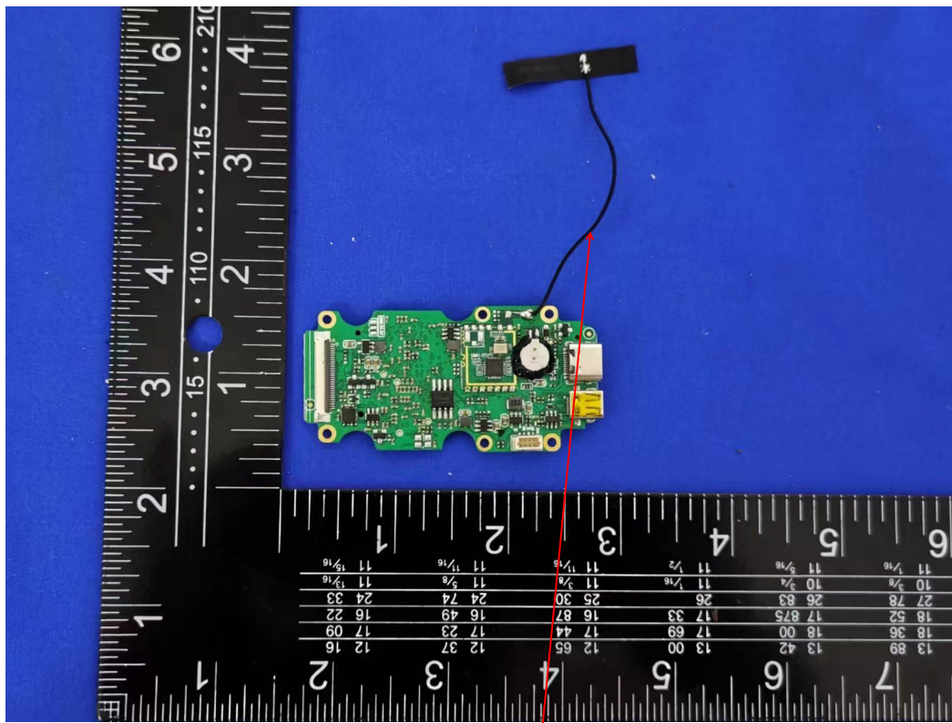
FPC antenna
