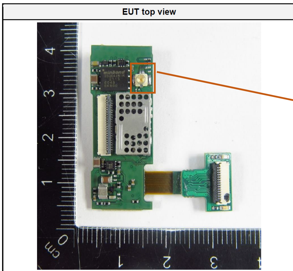
EUT Antenna connector for conducted testing
