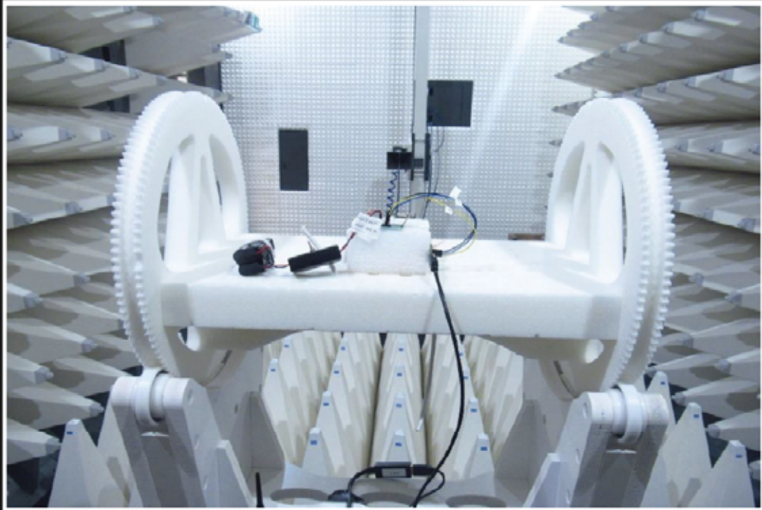
EUT Test Setup (back)
