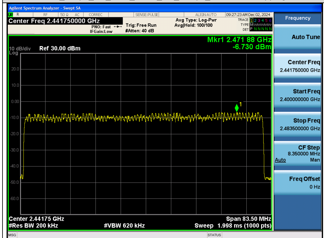
Test_Graph_EDR_HOP_ANT1_NA_3Mbps_Number of Hopping
