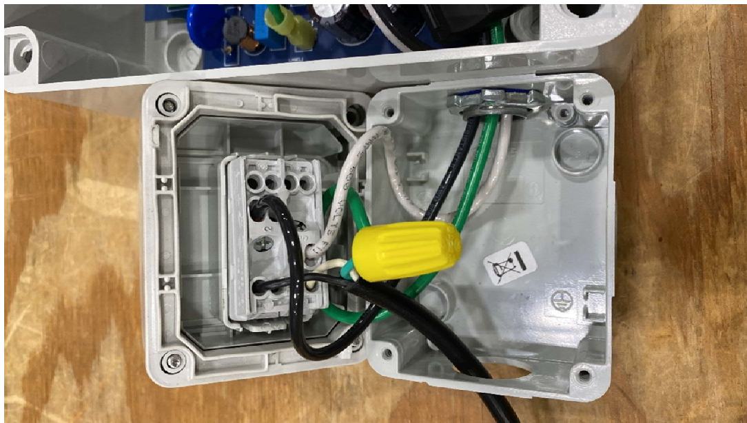
HIFIS Internal layout (AC Input Enclosure)
