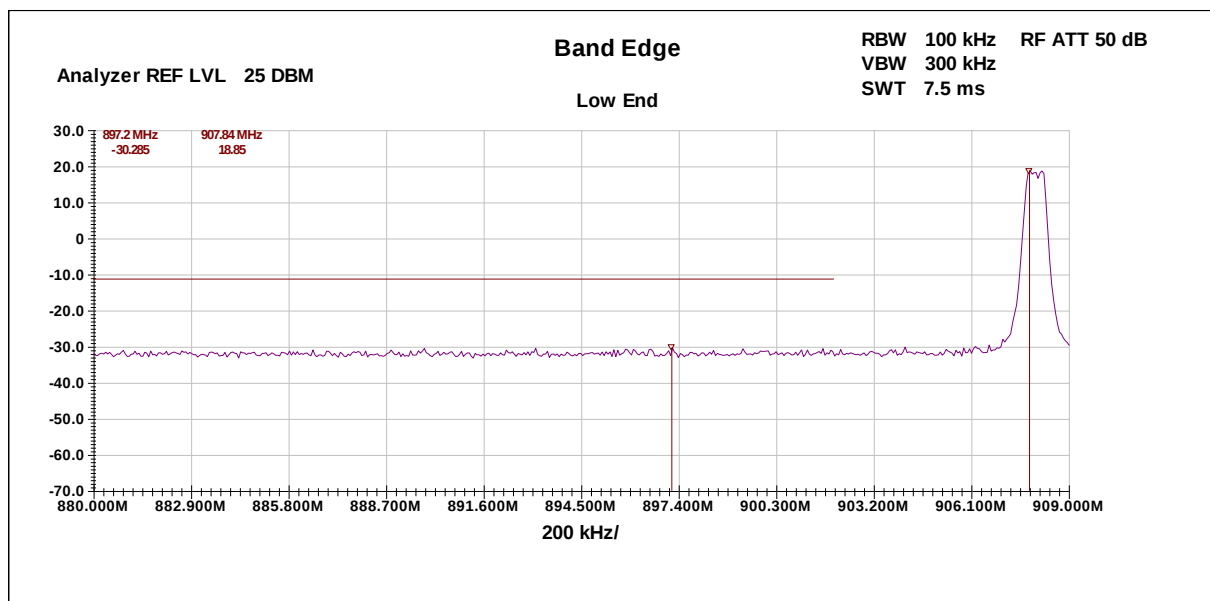
Figure 16-2 - Band Edge Lower Channel
