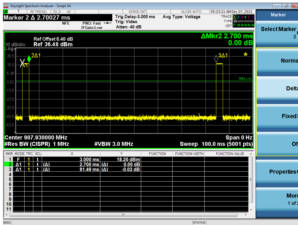
Figure 10-4 - Duty Cycle, Low Channel
