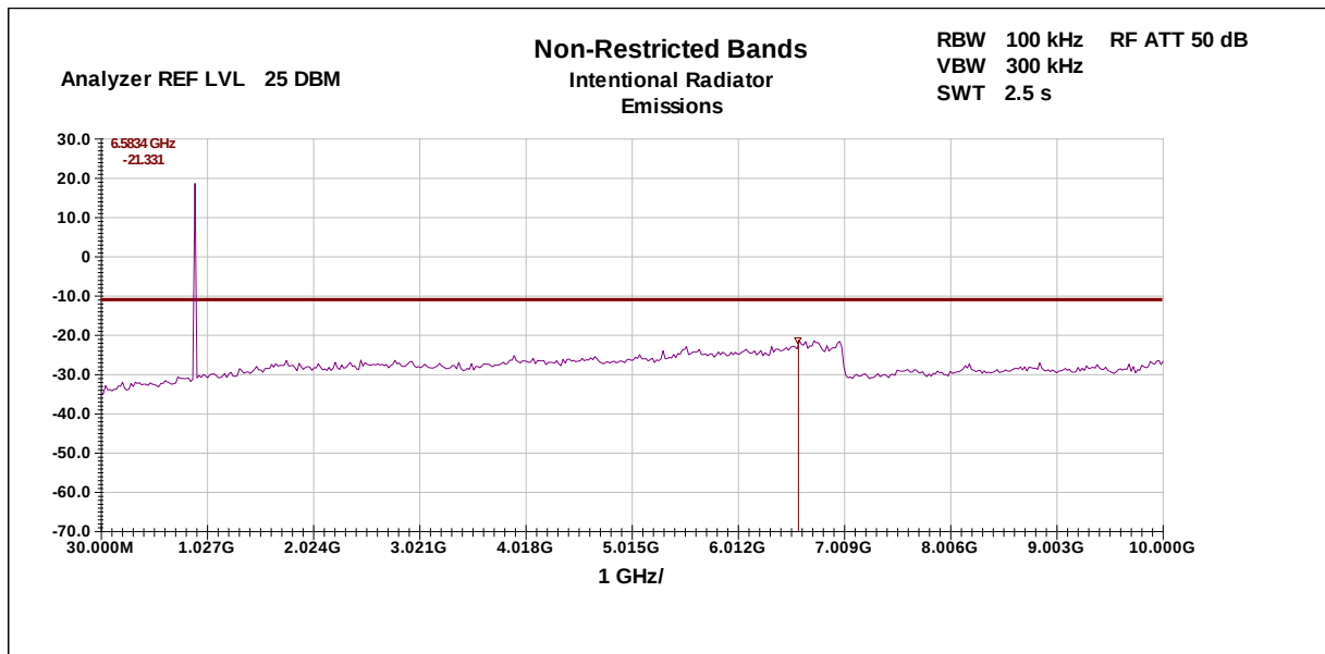
Figure 17-4 - 100kHz Spurious Emissions, High Channel
