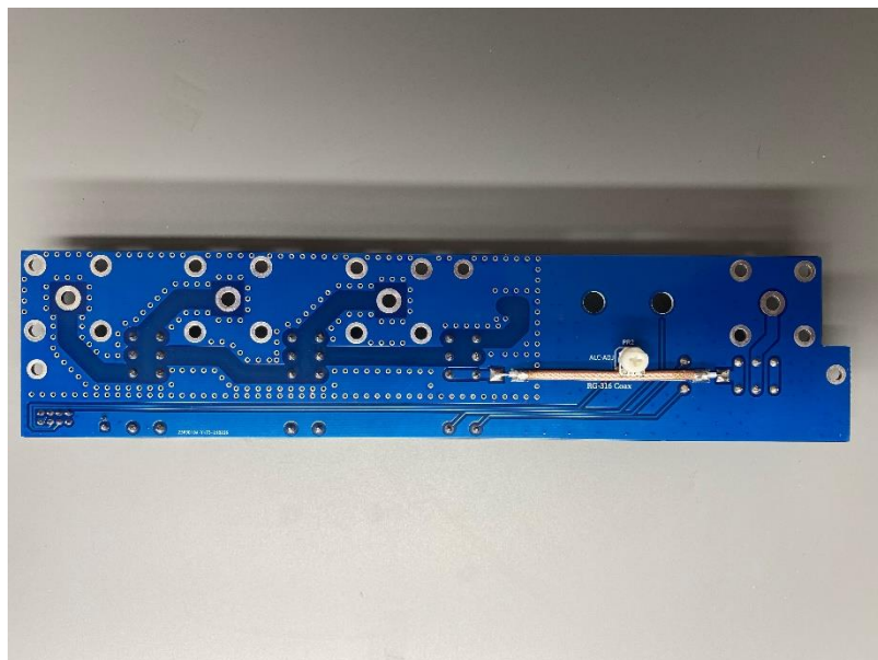
Antenna Switch Rear View
