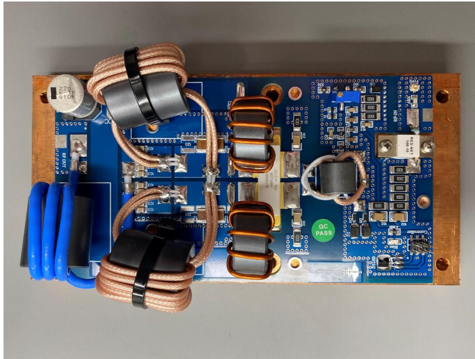
Power Unit Rear View
