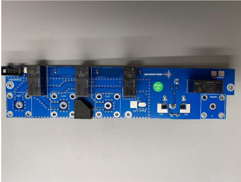
Antenna Switch Front View
