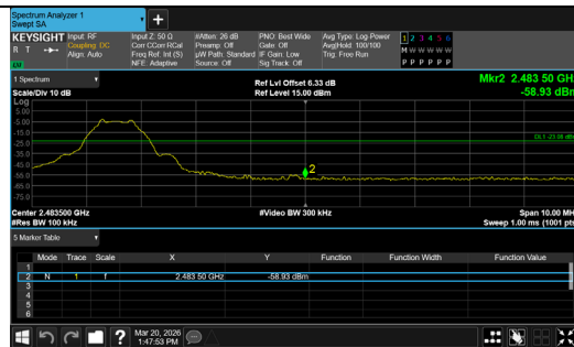
Out Of Band Emission BLE 1M_Channel 39
