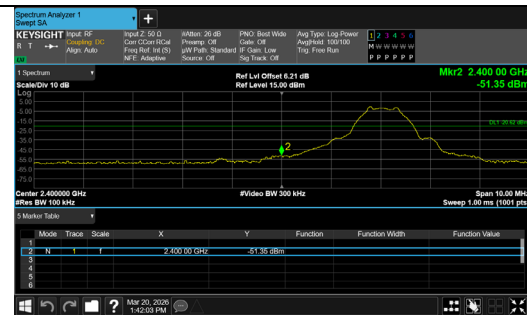
Out Of Band Emission BLE 1M_Channel 0
