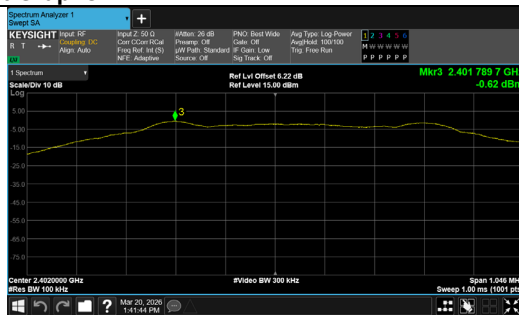
In-Band Reference Level BLE 1M_Channel 0
