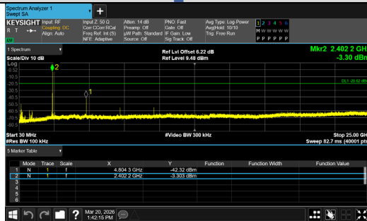
30.0 MHz - 25000.0 MHz BLE 1M_Channel 0
