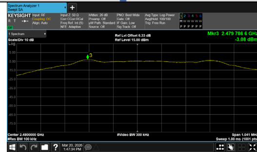
In-Band Reference Level BLE 1M_Channel 39
