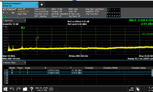
30.0 MHz - 25000.0 MHz BLE 1M_Channel 19
