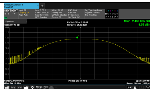
Peak Output Power BLE 1M_Channel 19
