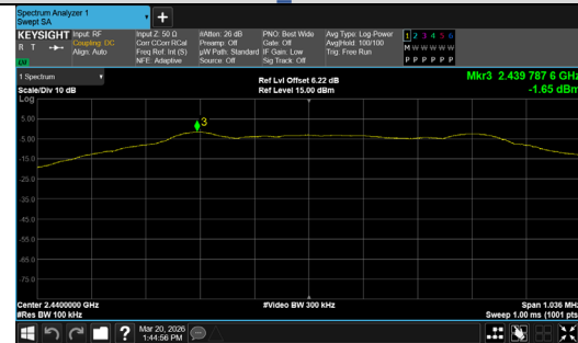
In-Band Reference Level BLE 1M_Channel 19
