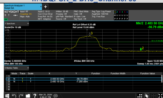
Out Of Band Emission \pi/4 DQPSK_2-DH5_Channel 78
