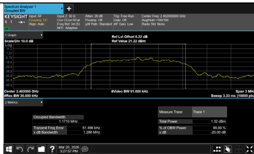
8DPSK_3-DH5_Channel 0
