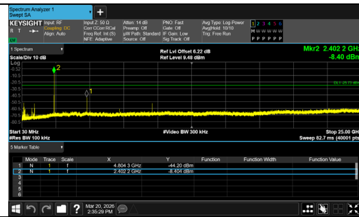
30.0 MHz - 25000.0 MHz \pi/4 DQPSK_2-DH5_Channel 0
