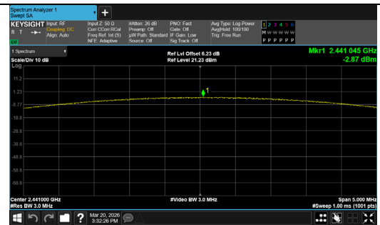
Peak Output Power 8DPSK_Channel 39
