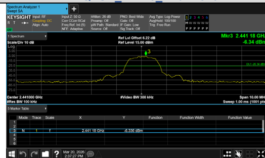
Out Of Band Emission \pi/4 DQPSK_2-DH5_Channel 39
