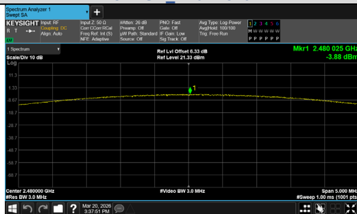
Peak Output Power 8DPSK_Channel 78
