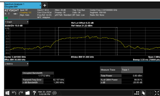
8DPSK_3-DH5_Channel 39
