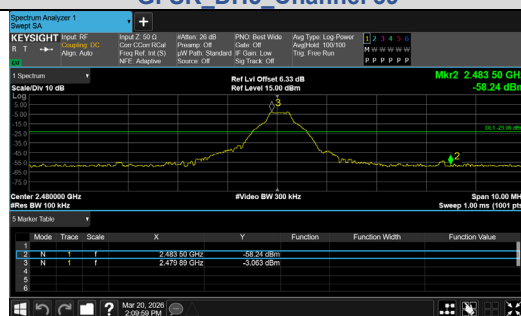
Out Of Band Emission GFSK_DH5_Channel 78
