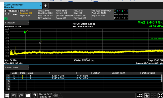
30.0 MHz - 25000.0 MHz \pi/4 DQPSK_2-DH5_Channel 39
