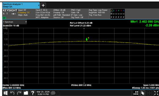
Peak Output Power 8DPSK_Channel 0
