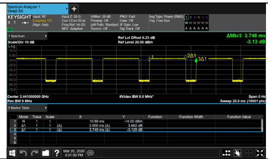
8DPSK(3-DH5)_Channel 39
