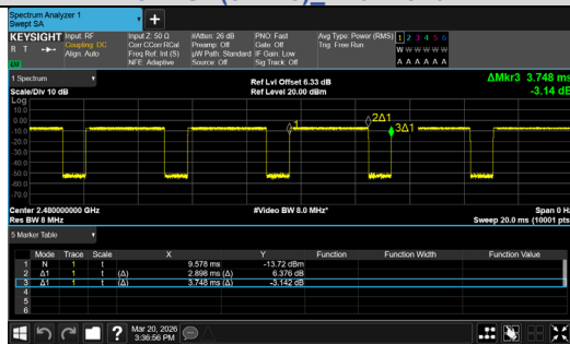
8DPSK(3-DH5)_Channel 78
