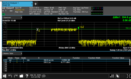
Pulse Width \pi/4 DQPSK_2-DH1
