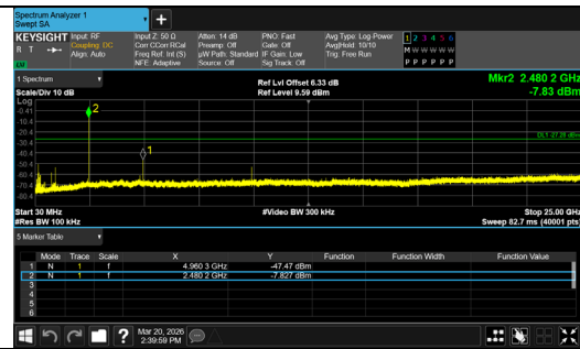
30.0 MHz - 25000.0 MHz \pi/4 DQPSK_2-DH5_Channel 78
