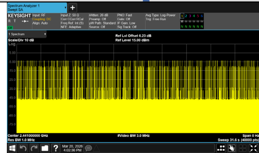
Number of Pulses in 31.6 seconds \pi/4 DQPSK_2-DH3
