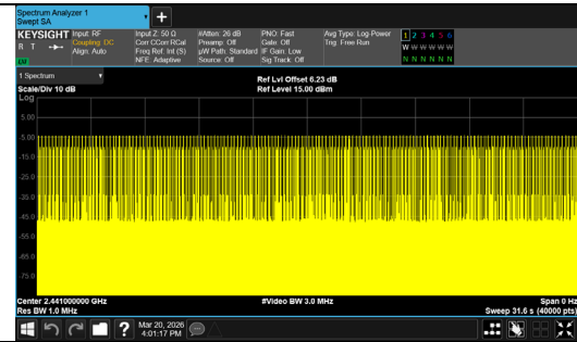
Number of Pulses in 31.6 seconds \pi/4 DQPSK_2-DH1
