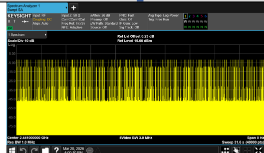
Number of Pulses in 31.6 seconds GFSK_DH3
