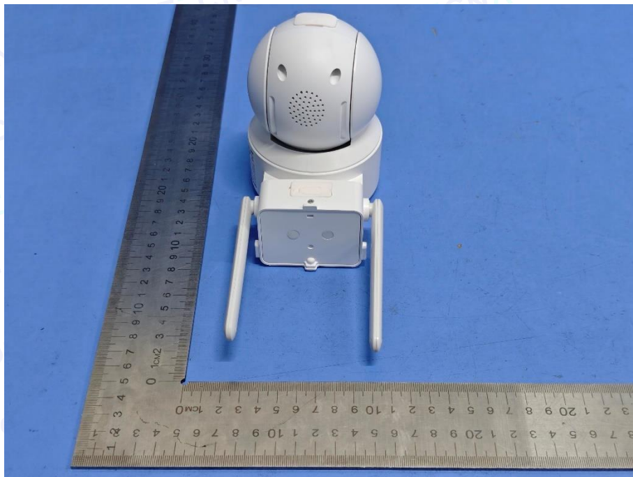
Photo 6 Appearance of EUT (GW30)
