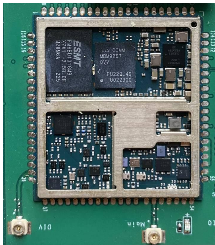
Photo 8: Internal View for LTE Module
