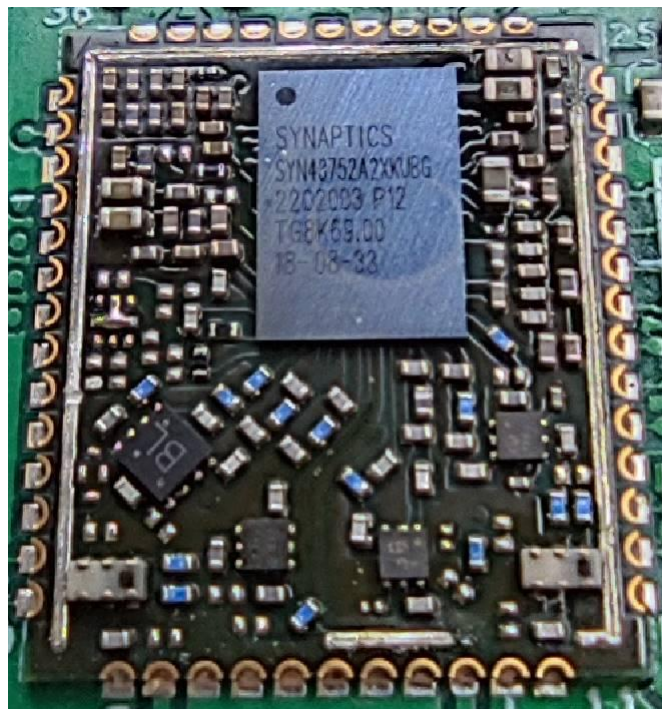
Photo 6: Internal View for WiFi&BT Module
