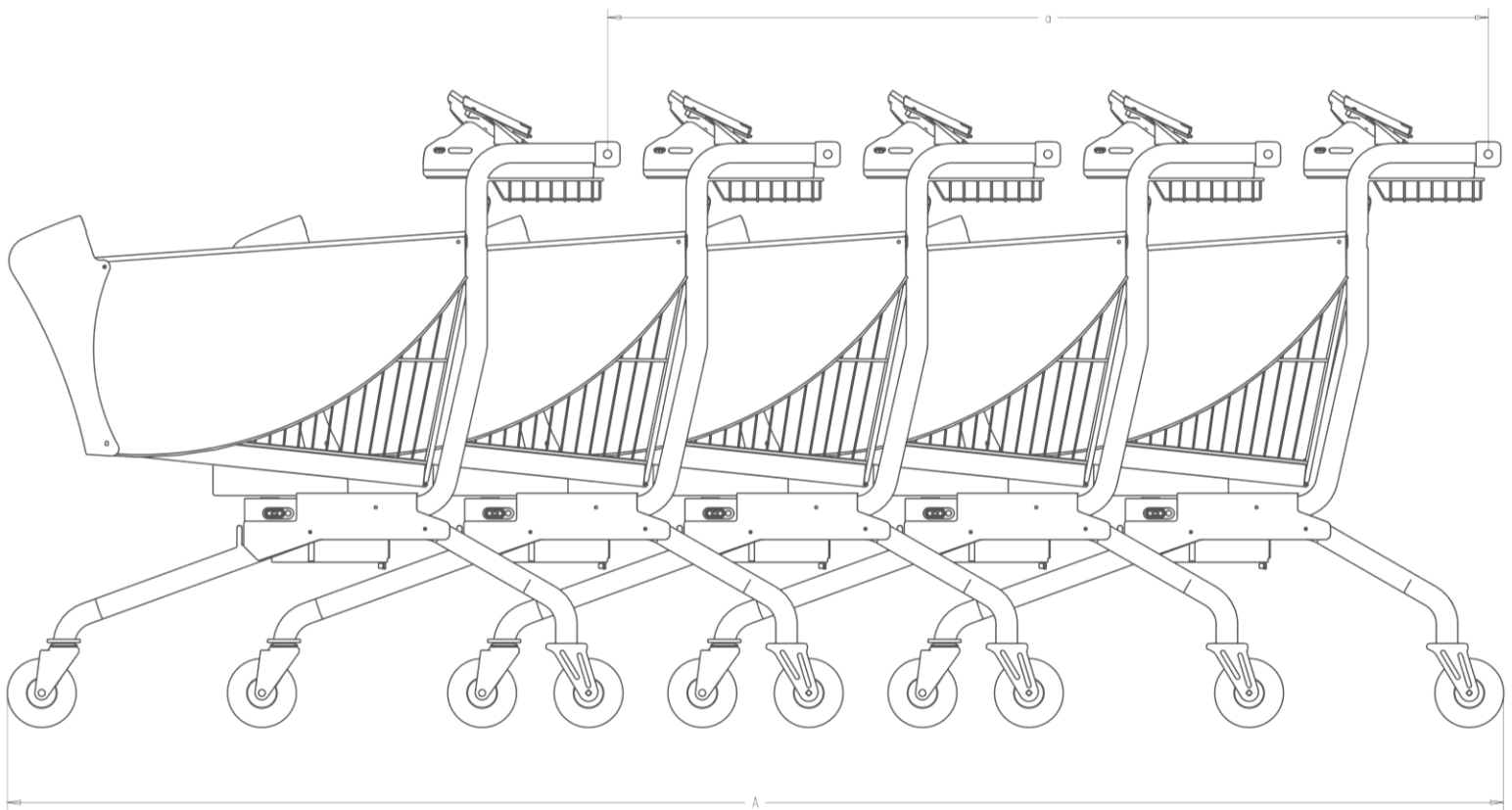
Five cart stacking dimensions
