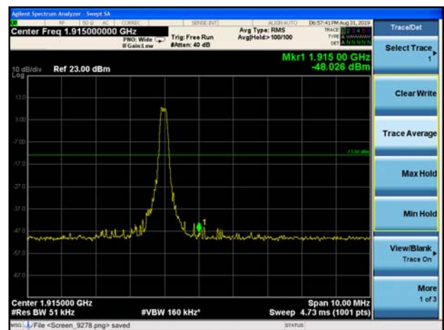
LTE Band 25 15MHz 16QAM 1RB CH-High
