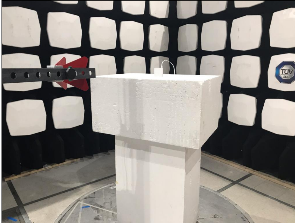
Figure 6: Equipment Under Test – Radiated Emissions – Z-orientation
