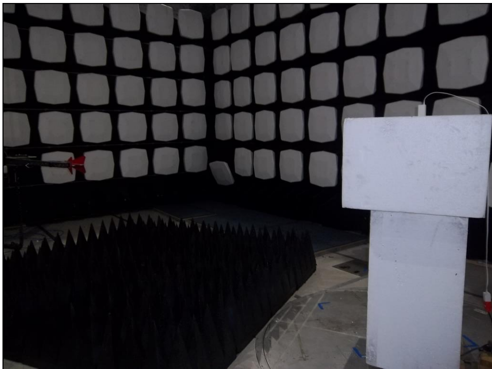
Figure 12: Equipment Under Test – Radiated Emissions >1GHz
