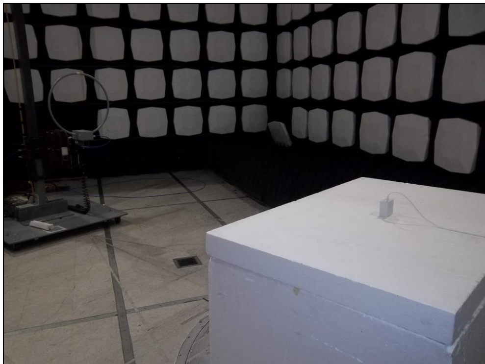
Figure 8: Equipment Under Test – Radiated Emissions <30MHz
