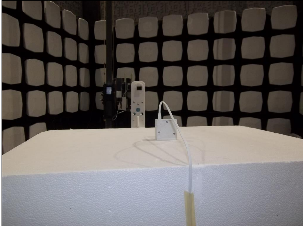
Figure 14: Equipment Under Test – Radiated Emissions >18GHz
