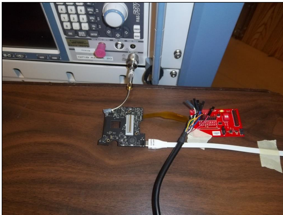
Figure 3: Equipment Under Test – Antenna Port Conducted Measurements
