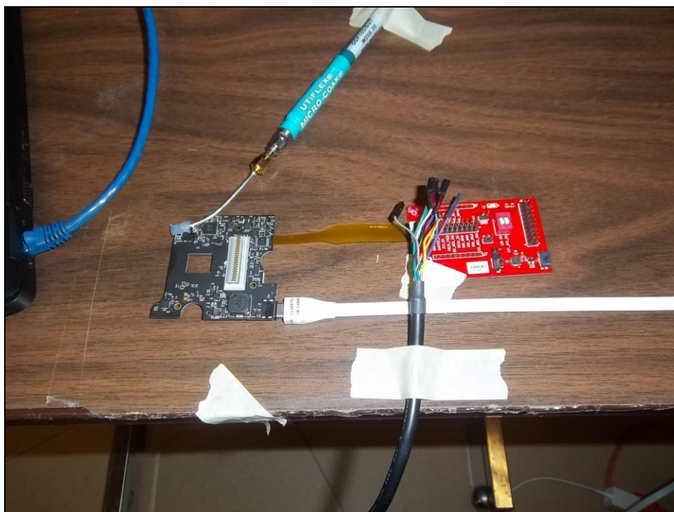
Figure 2: Equipment Under Test – Antenna Port Conducted Measurements
