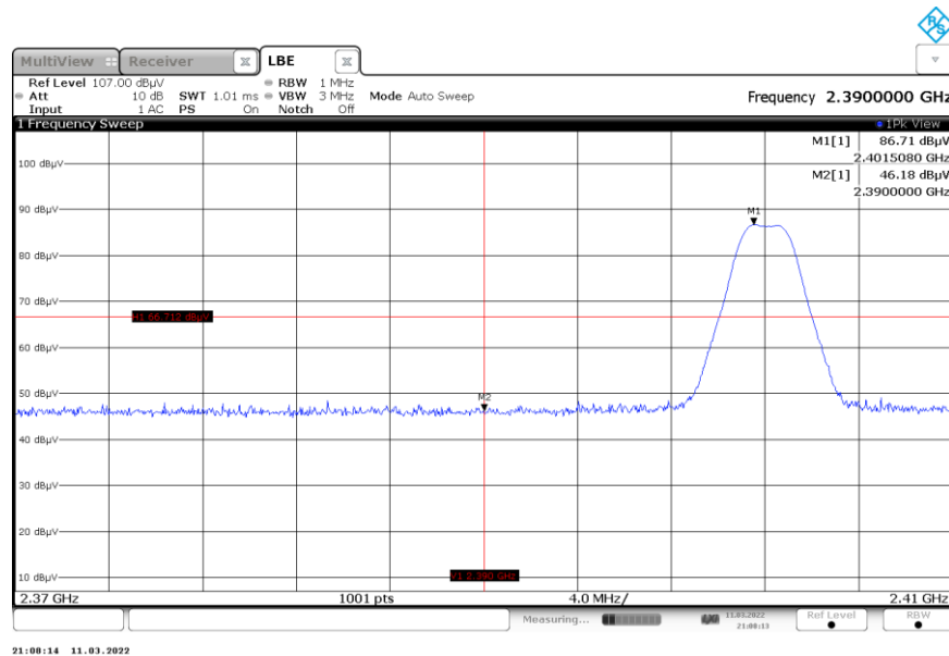
Figure 1: Reference plot Radiated Lower Band-edge – LCH
