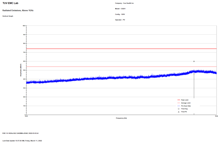
Figure 12: Reference plot for Radiated Spurious Emissions – 10 GHz – 18 GHz – V polarity
