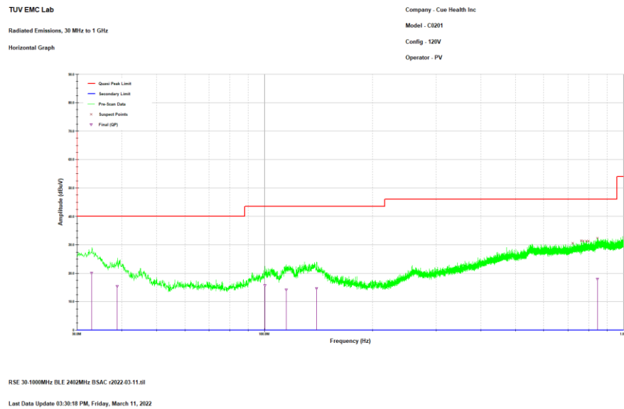
Figure 5: Reference plot for Radiated Spurious Emissions – 30 MHz – 1 GHz – H Polarity
