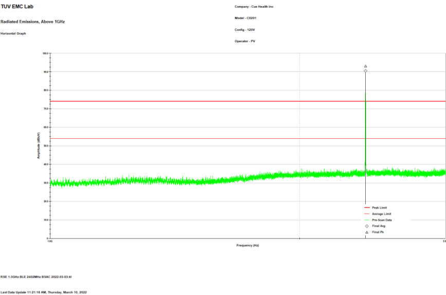
Figure 7: Reference plot for Radiated Spurious Emissions – 1 GHz – 3 GHz – H Polarity
