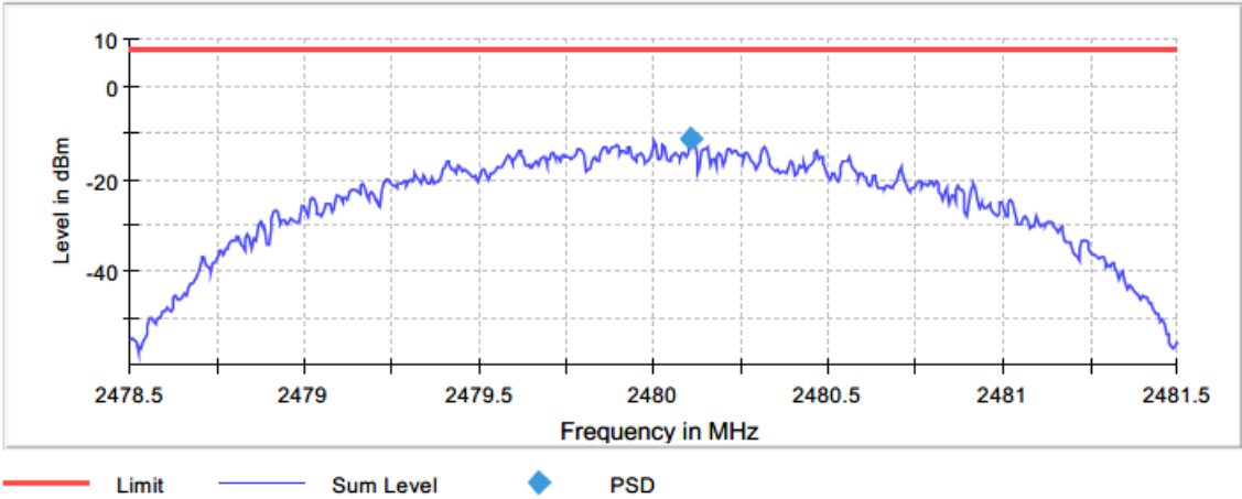
Figure 2.5.6-3: PSD – HCH
