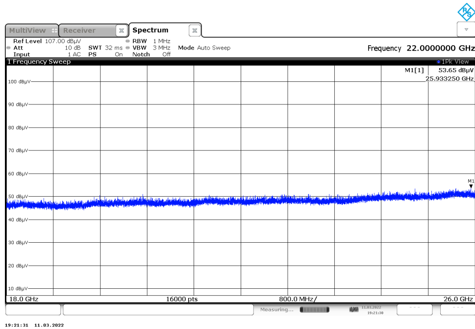
Figure 13: Reference plot for Radiated Spurious Emissions – 18 GHz – 26 GHz
