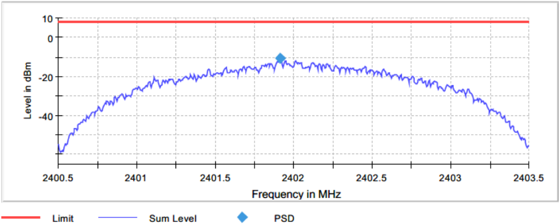
Figure 2.5.6-1: PSD – LCH
