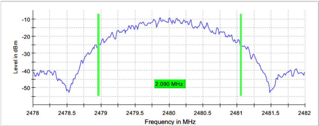
Figure 2.4.6-6: 99% BW - HCH
