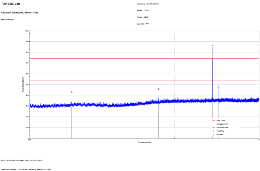
Figure 8: Reference plot for Radiated Spurious Emissions – 1 GHz – 3 GHz – V Polarity
