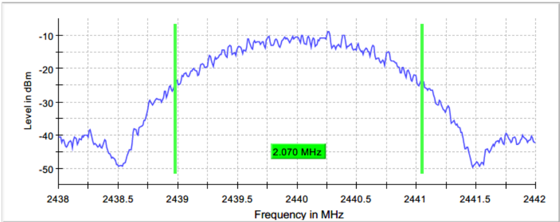
Figure 2.4.6-5: 99% BW - MCH
