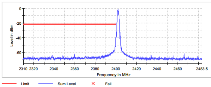
Figure 2.6.6-1: Lower Band-edge
