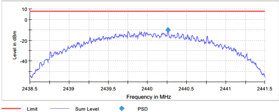
Figure 2.5.6-2: PSD – MCH
