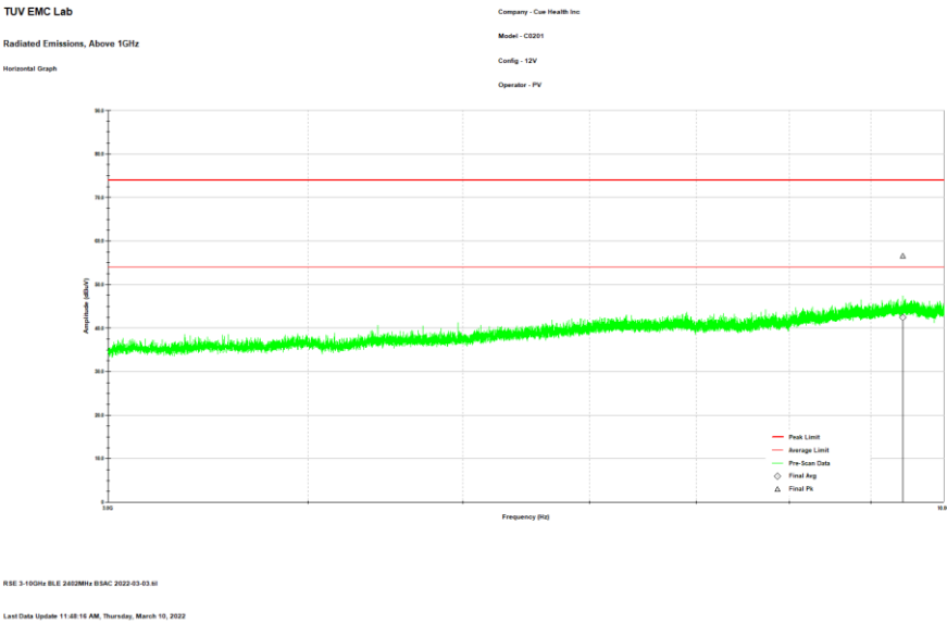
Figure 9: Reference plot for Radiated Spurious Emissions – 3 GHz – 10 GHz – H Polarity
