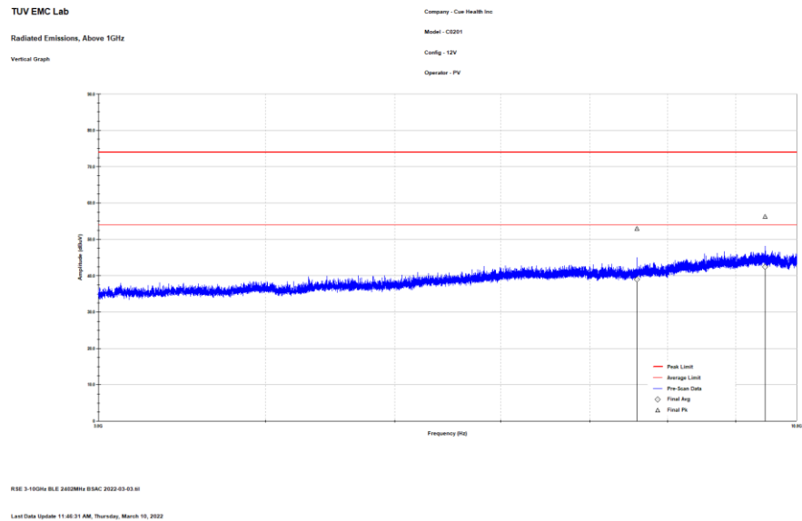
Figure 10: Reference plot for Radiated Spurious Emissions – 3 GHz – 10 GHz – V Polarity
