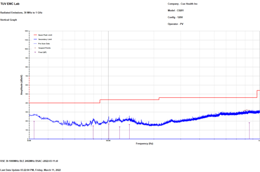
Figure 6: Reference plot for Radiated Spurious Emissions – 30 MHz – 1 GHz – V Polarity
