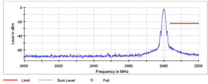
Figure 2.6.6-2: Upper Band-edge
