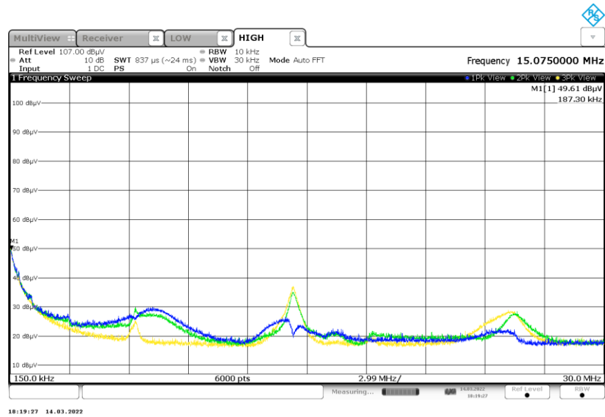
Figure 4: Reference plot for Radiated Spurious Emissions– 150 kHz – 30MHz Note: Emissions above the noise floor are ambient not associated with the EUT.
