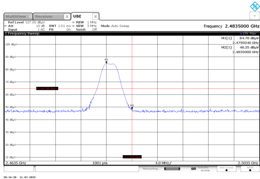
Figure 2: Reference plot Radiated Upper Band-edge – HCH
