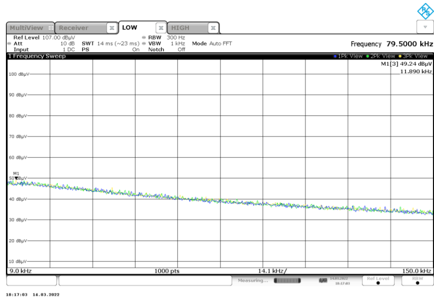
Figure 3: Reference plot for Radiated Spurious Emissions – 9 kHz – 150 kHz
