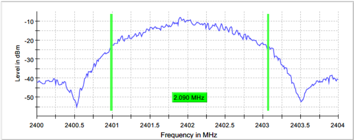
Figure 2.4.6-4: 99% BW - LCH
