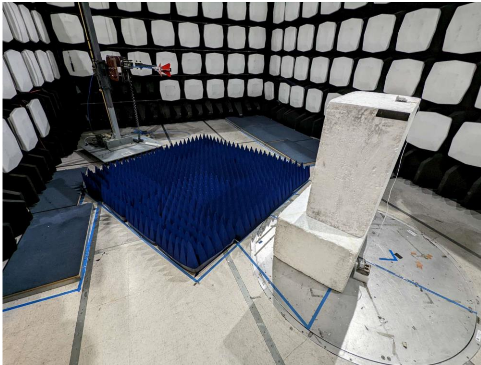
Figure A-3: Test Setup – Radiated Emissions >1GHz
