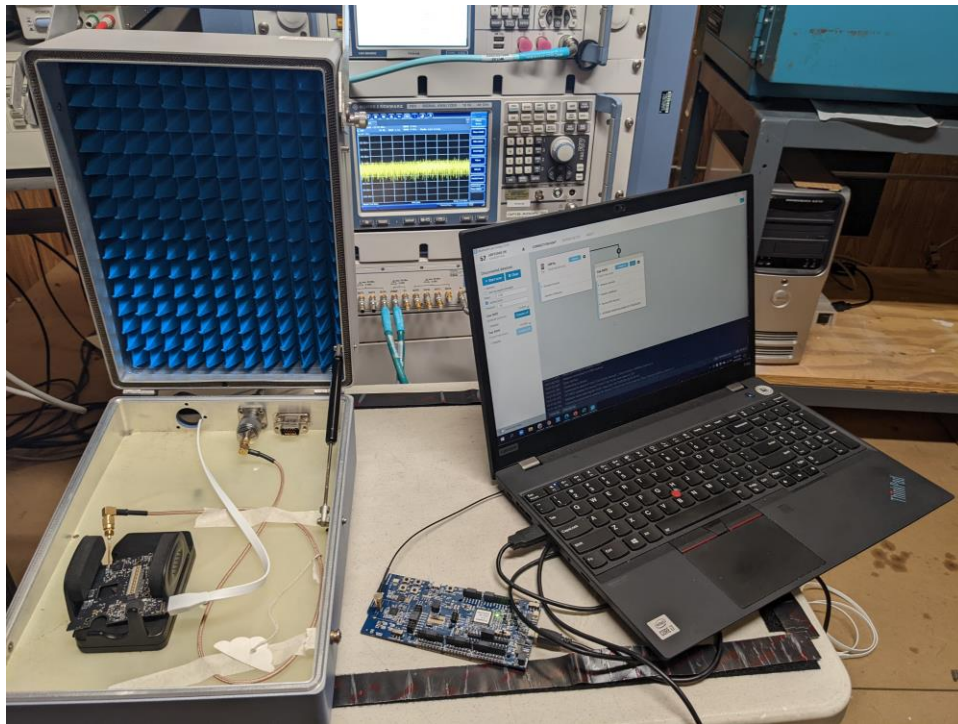
Figure A-7: Test Setup – Receiver Blocking
