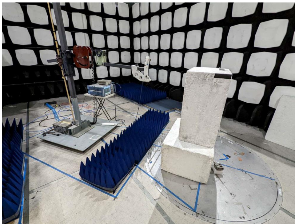
Figure A-5: Test Setup – Radiated Emissions >18GHz
