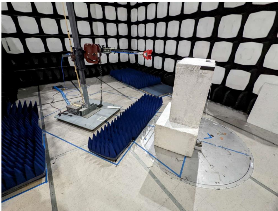
Figure A-4: Test Setup – Radiated Emissions >10GHz
