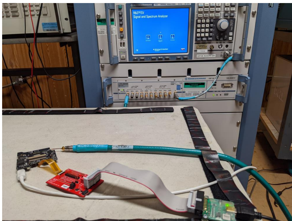
Figure A-6: Test Setup – Conducted measurement
