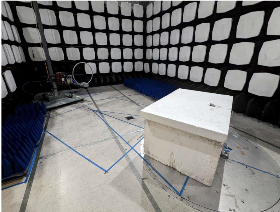
Figure A-1: Test Setup – Radiated Emissions <30MHz
