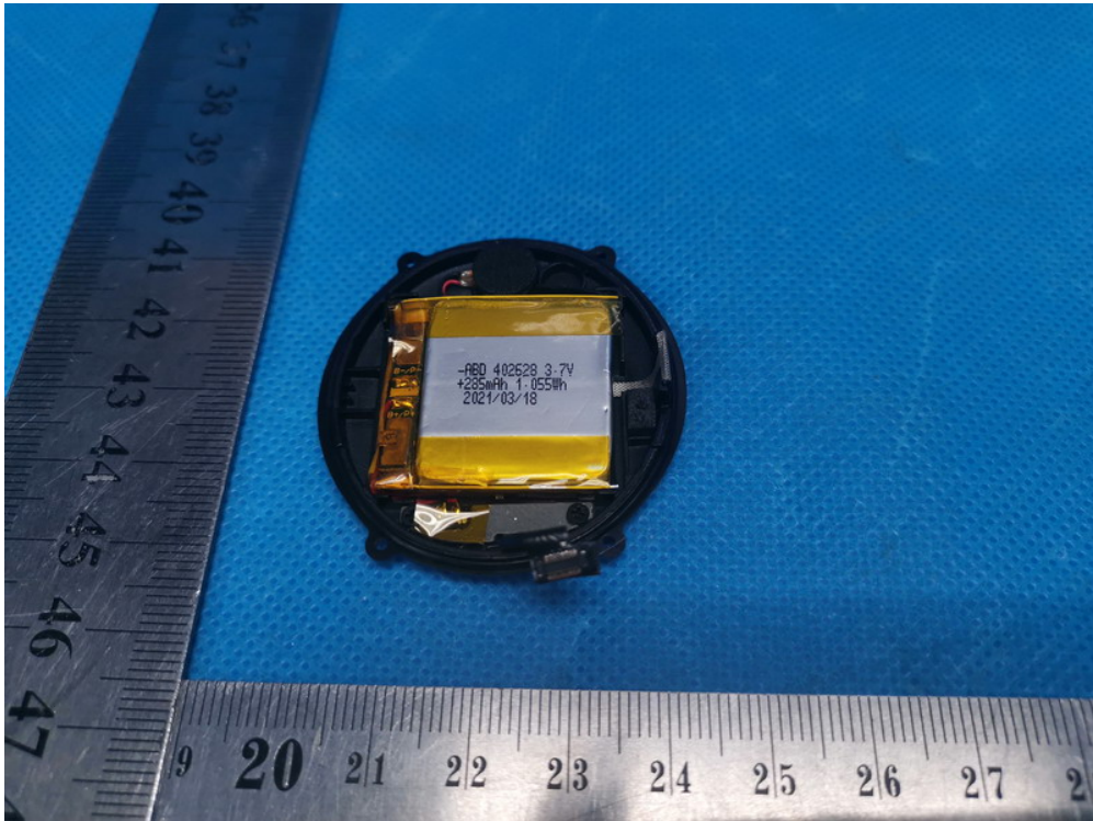
Battery View
