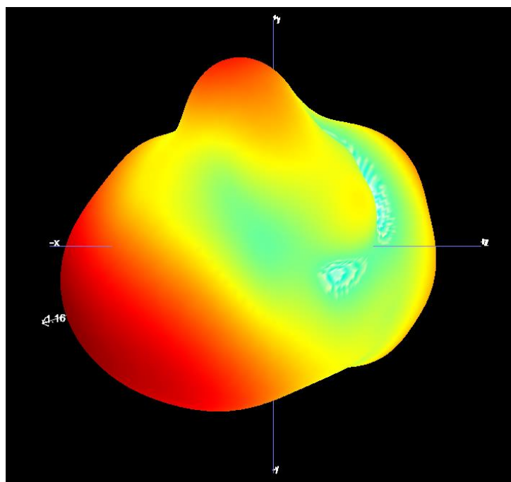
B1.3 3D Pattern for 2483MHz
