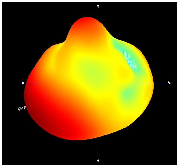
B1.2 3D Pattern for 2442MHz
