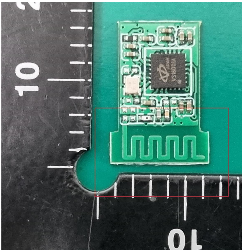
Antenna (Close-up and Location)
