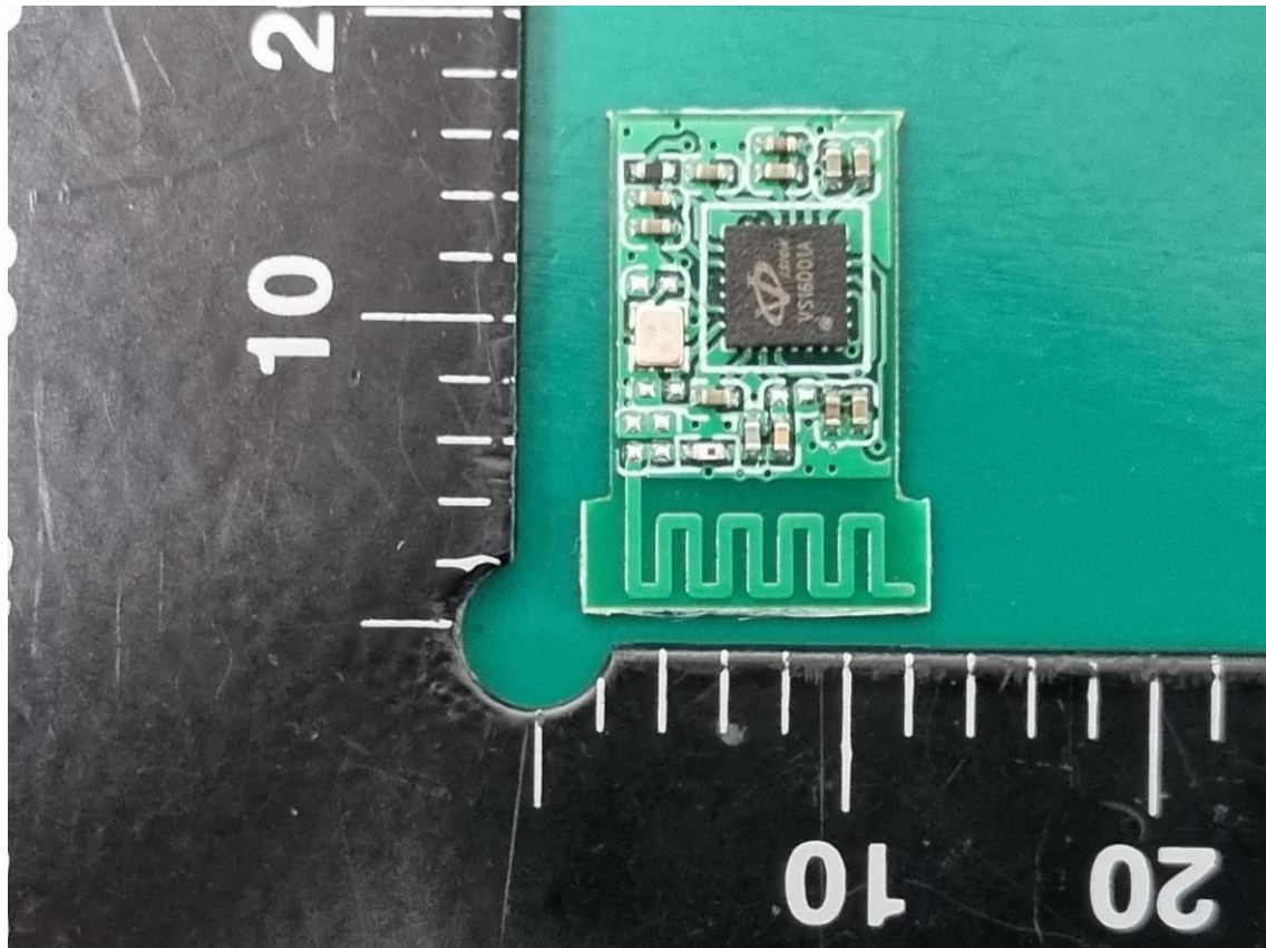
Main Board (dongle, rear)
