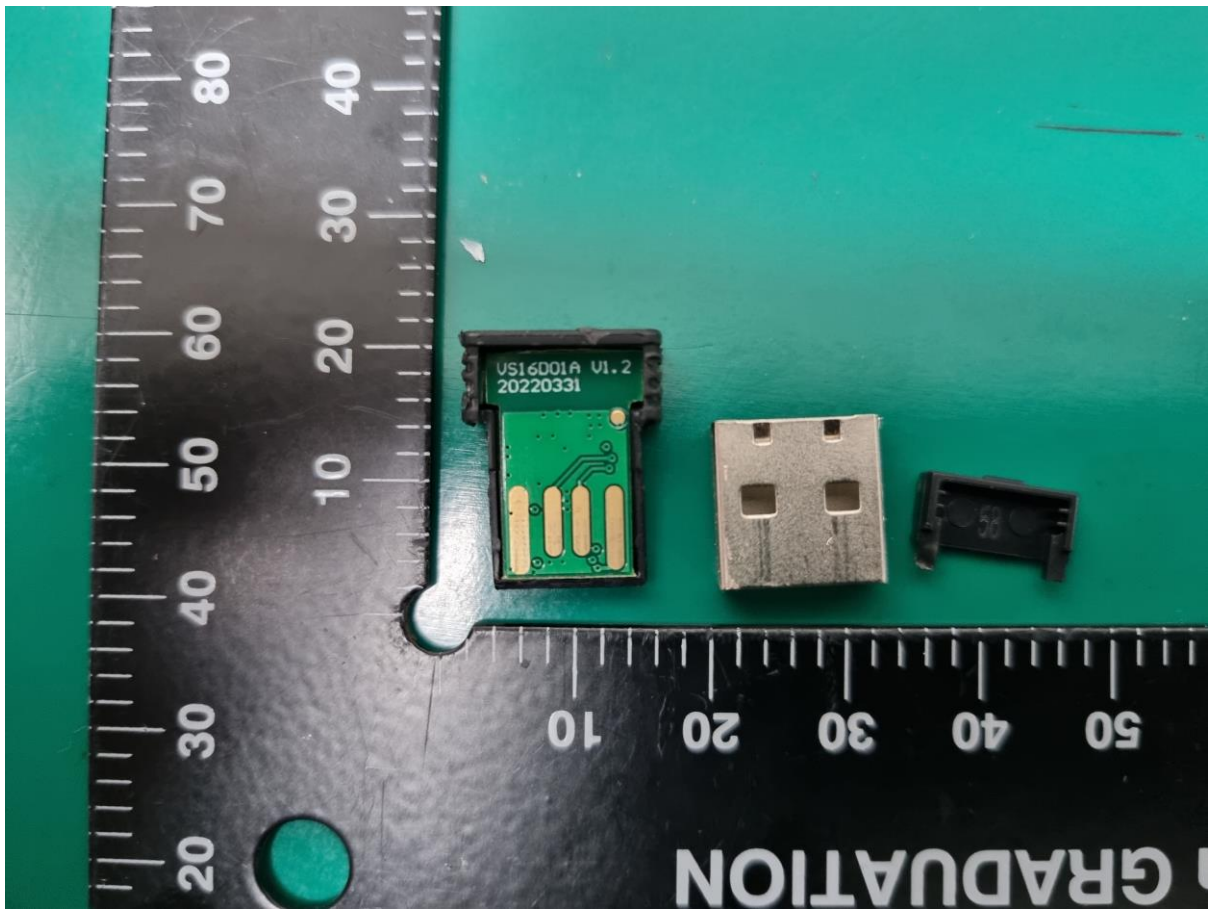
Internal of sample (dongle)
