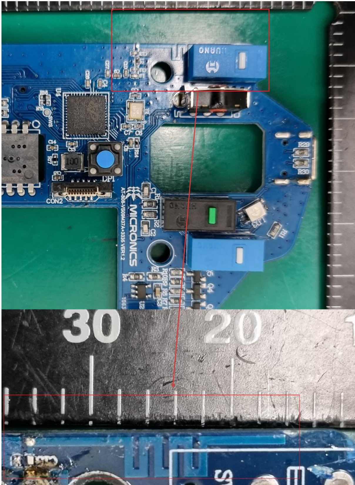
Antenna (close-up and location)
