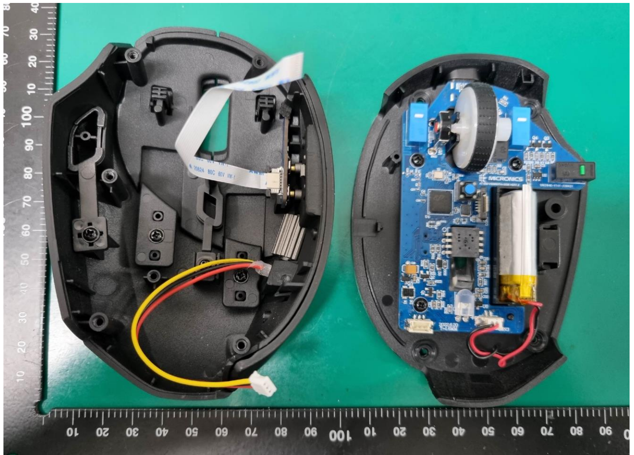
Internal of sample (mouse)
