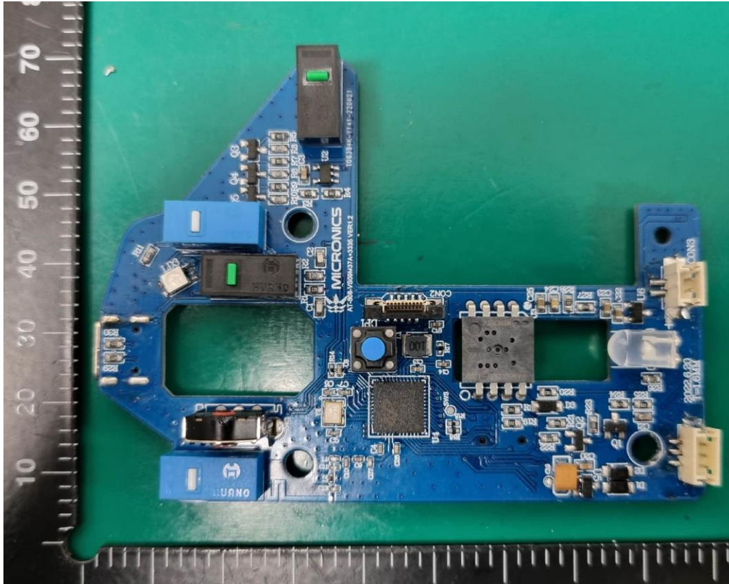
Main Board (mouse, rear)
