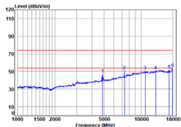
BLE_1M_TX_CH_19_Vertical
