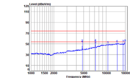
BLE_1M_TX_CH_00_Horizontal
