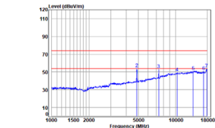
BLE_1M_TX_CH_19_Horizontal
