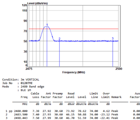
BLE_1M_TX_CH_39_Vertical-Peak
