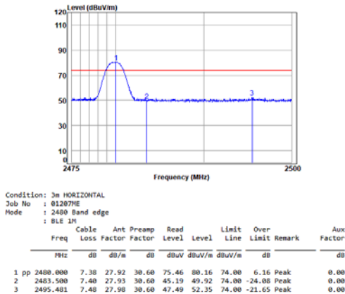
BLE_1M_TX_CH_39_Horizontal-Peak
