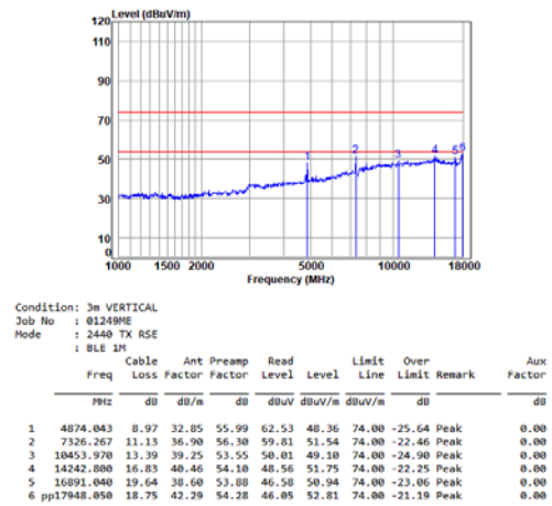
BLE_1M_TX_CH_19_Vertical
