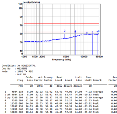
BLE_1M_TX_CH_00_Horizontal
