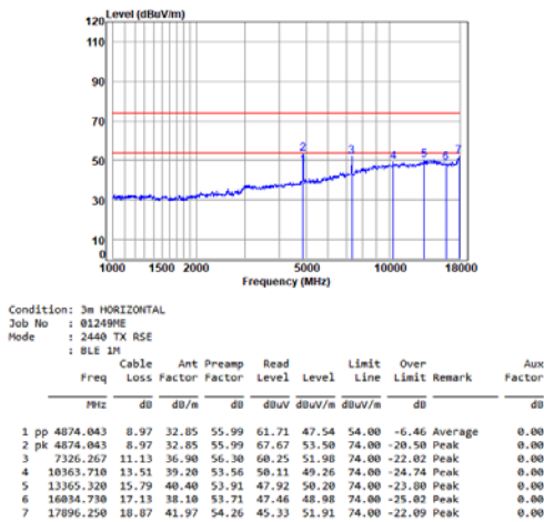
BLE_1M_TX_CH_19_Horizontal
