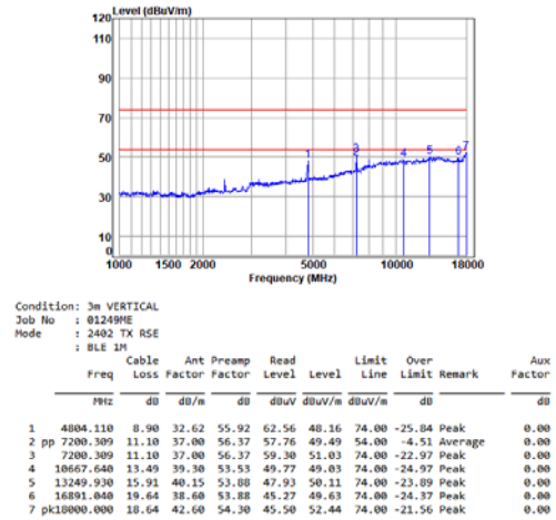
BLE_1M_TX_CH_00_Vertical
