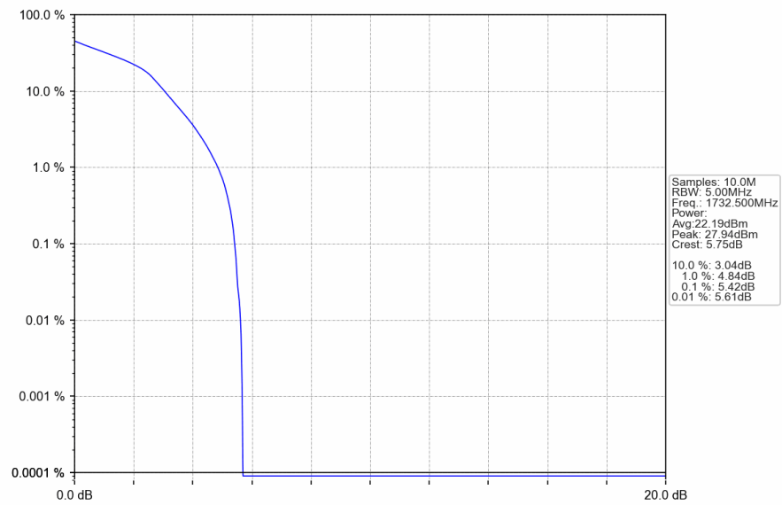
Band4_1.4MHz_16QAM_MCH_1732.5MHz_RB_6_0_NTNV
