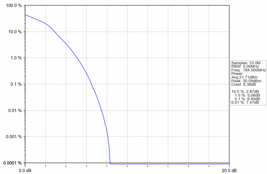
Band13_5MHz_16QAM_HCH_784.5MHz_RB_25_0_NTNV
