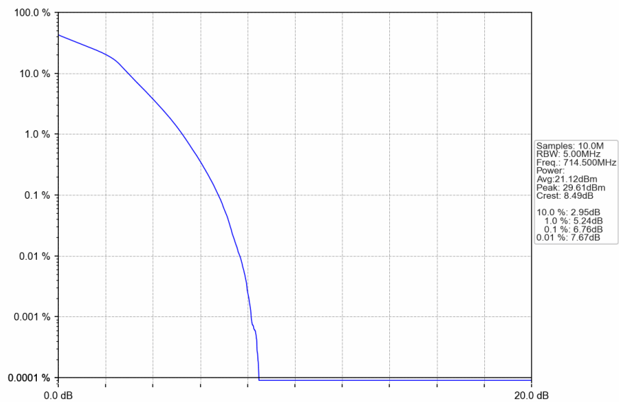
Band12_3MHz_16QAM_HCH_714.5MHz_RB_15_0_NTNV
