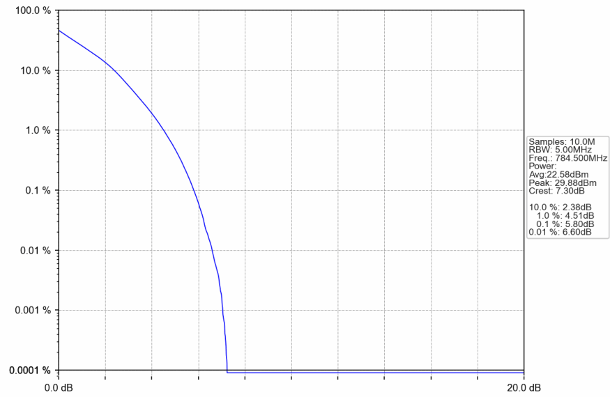
Band13_5MHz_QPSK_HCH_784.5MHz_RB_25_0_NTNV
