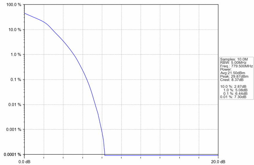
Band13_5MHz_16QAM_LCH_779.5MHz_RB_25_0_NTNV
