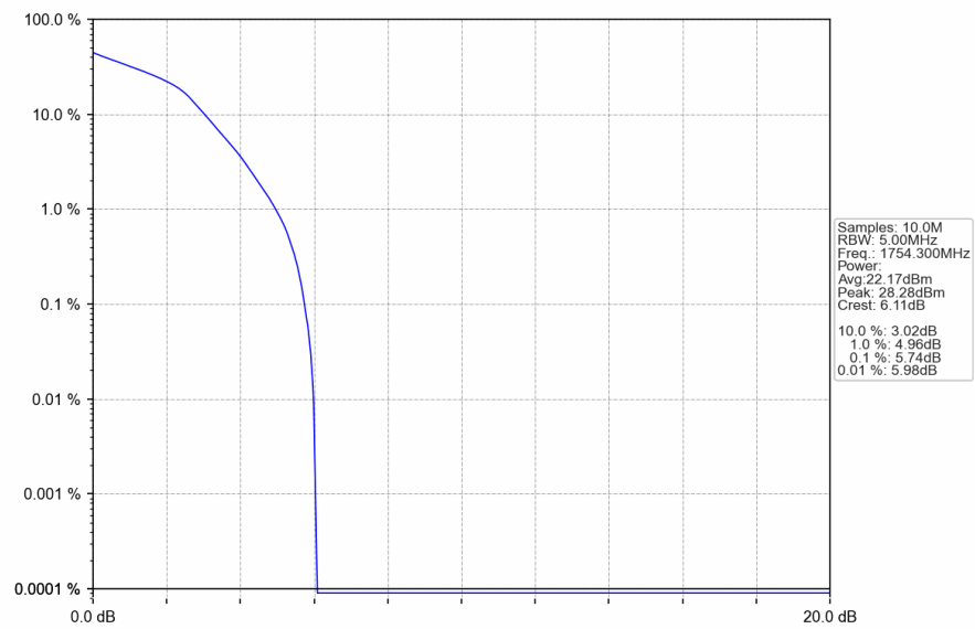
Band4_1.4MHz_16QAM_HCH_1754.3MHz_RB_6_0_NTNV
