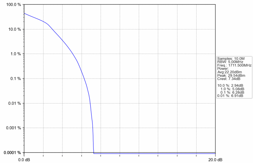
Band4_3MHz_16QAM_LCH_1711.5MHz_RB_15_0_NTNV
