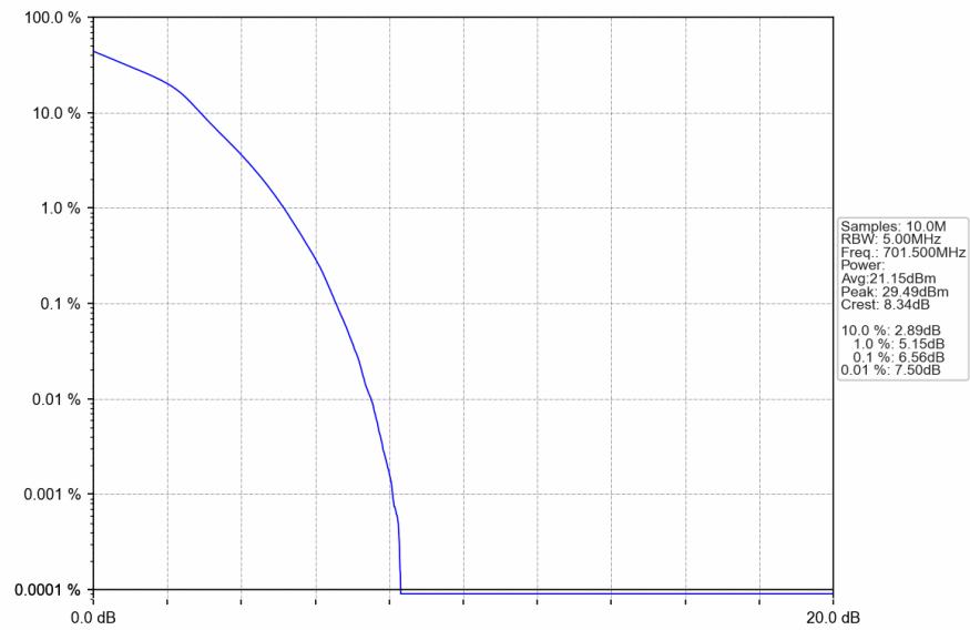
Band12_5MHz_16QAM_LCH_701.5MHz_RB_25_0_NTNV
