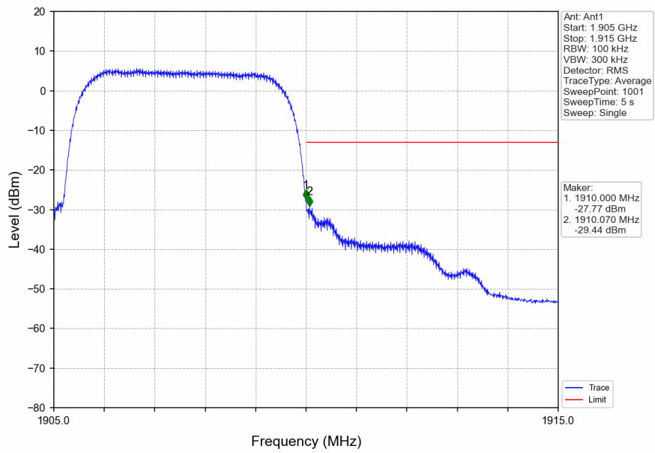
Band2_HSDPA_HCH_1907.6MHz_Subtest 1_NTNV
