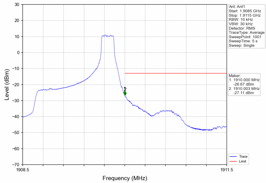
Band2_1.4MHz_16QAM_HCH_1909.3MHz_RB_6_0_NTNV
