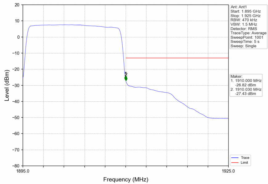
Band2_15MHz_16QAM_HCH_1902.5MHz_RB_75_0_NTNV
