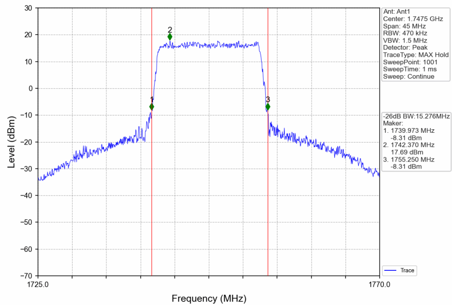
Band4_15MHz_16QAM_HCH_1747.5MHz_RB_75_0_NTNV
