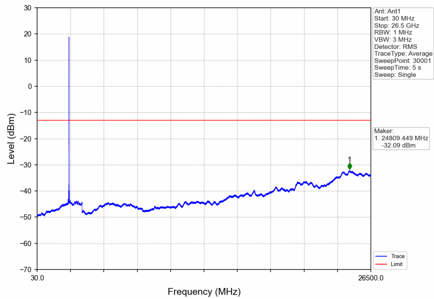
Band7_15MHz_16QAM_HCH_2562.5MHz_RB_1_0_NTNV
