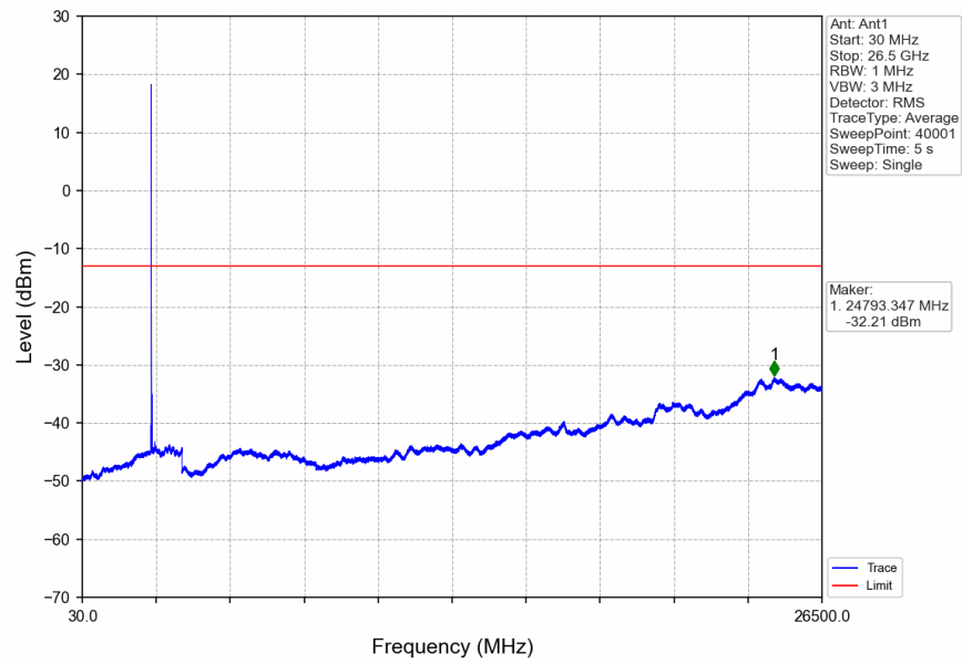
Band7_10MHz_16QAM_LCH_2505MHz_RB_50_0_NTNV
