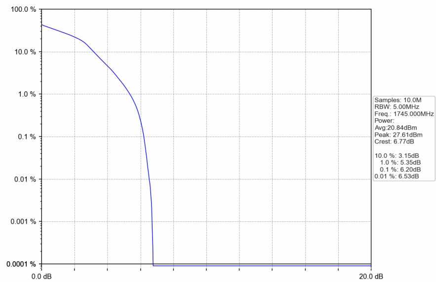
Band66_1.4MHz_16QAM_MCH_1745MHz_RB_6_0_NTNV
