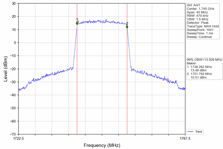
Band66_15MHz_QPSK_MCH_1745MHz_RB_75_0_NTNV
