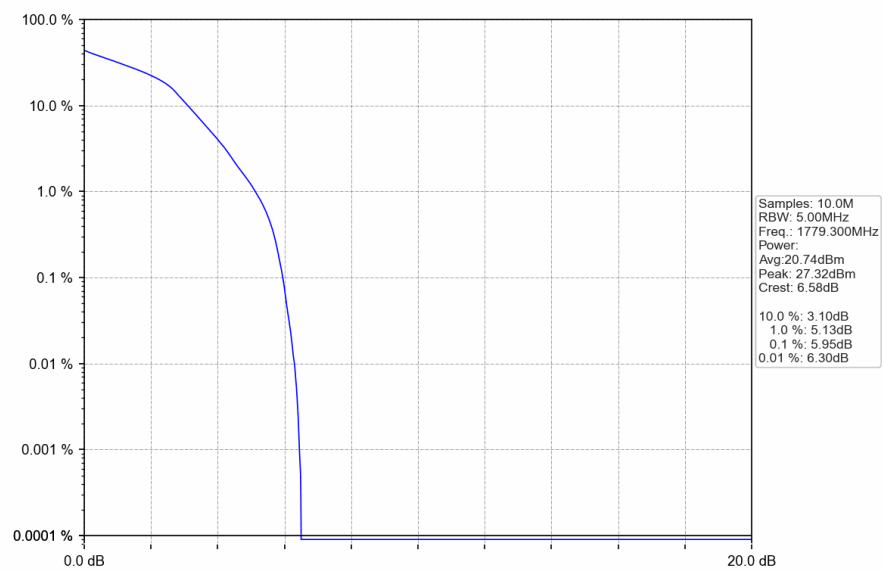
Band66_1.4MHz_16QAM_HCH_1779.3MHz_RB_6_0_NTNV
