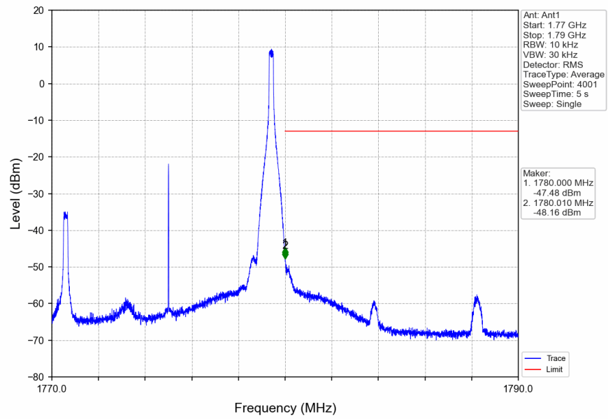
Band66_10MHz_16QAM_HCH_1775MHz_RB_50_0_NTNV
