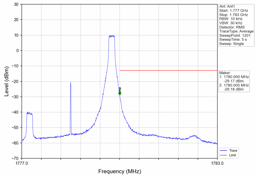
Band66_3MHz_16QAM_HCH_1778.5MHz_RB_15_0_NTNV
