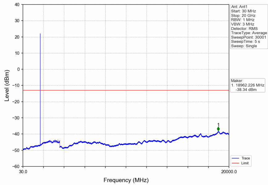
Band66_1.4MHz_16QAM_LCH_1710.7MHz_RB_6_0_NTNV
