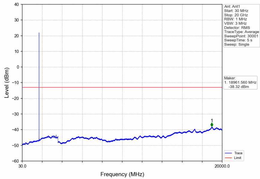
Band66_3MHz_16QAM_LCH_1711.5MHz_RB_15_0_NTNV
