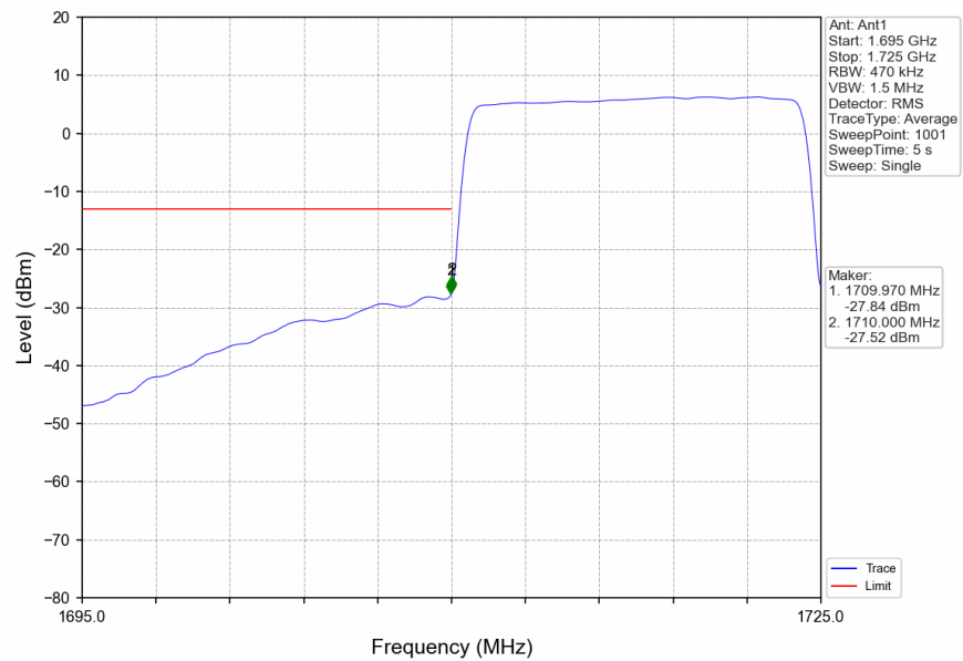
Band66_15MHz_16QAM_LCH_1717.5MHz_RB_75_0_NTNV
