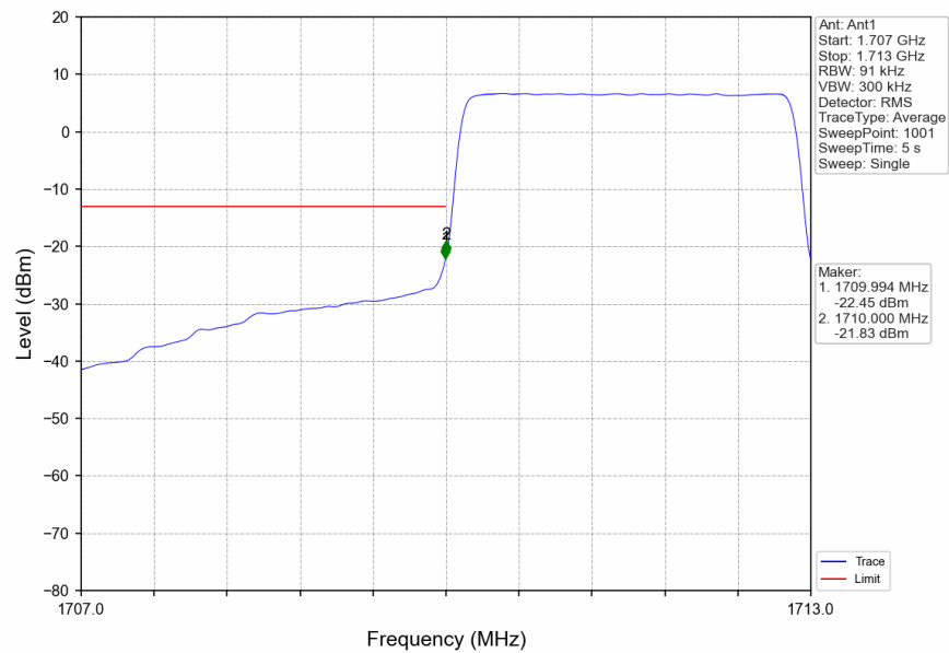
Band66_3MHz_16QAM_LCH_1711.5MHz_RB_15_0_NTNV
