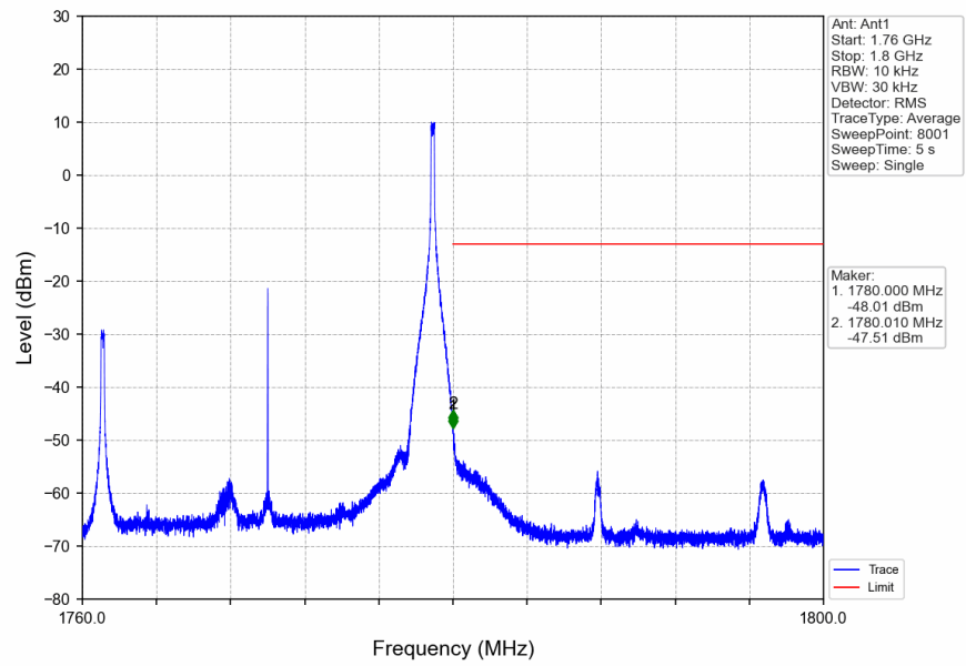
Band66_20MHz_16QAM_HCH_1770MHz_RB_100_0_NTNV
