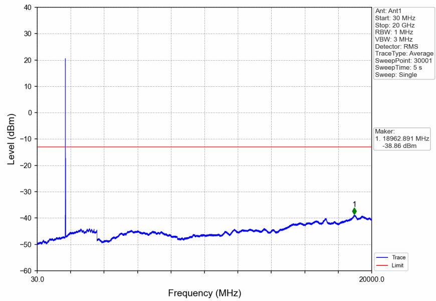
Band66_15MHz_16QAM_LCH_1717.5MHz_RB_75_0_NTNV
