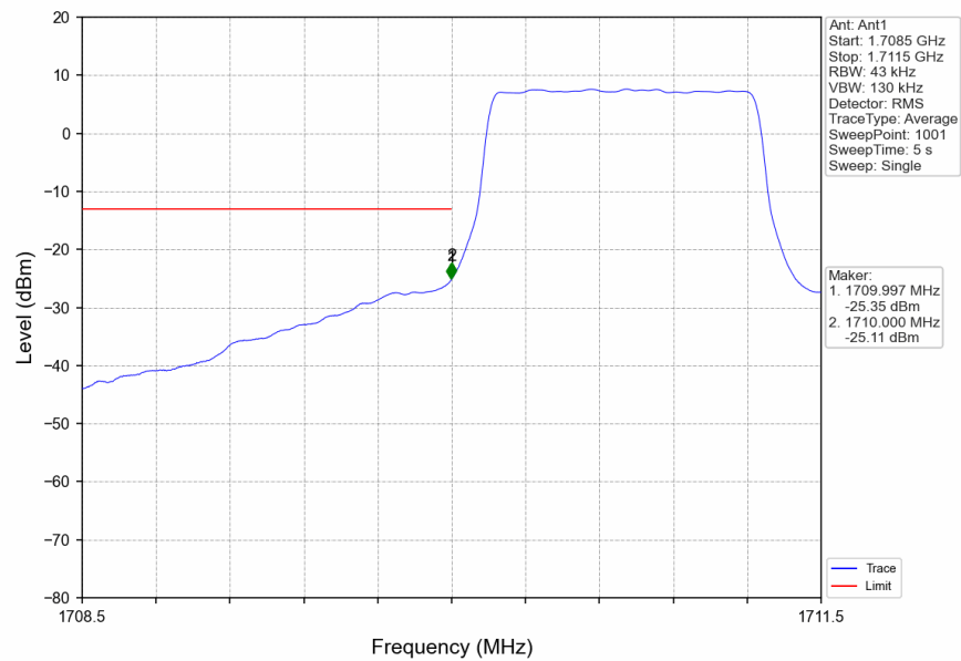
Band66_1.4MHz_16QAM_LCH_1710.7MHz_RB_6_0_NTNV
