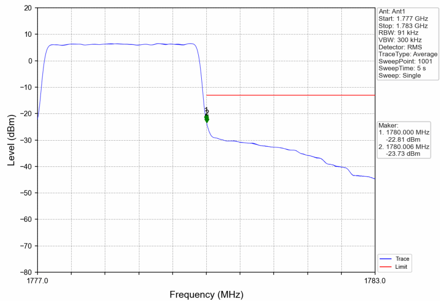
Band66_3MHz_16QAM_HCH_1778.5MHz_RB_15_0_NTNV
