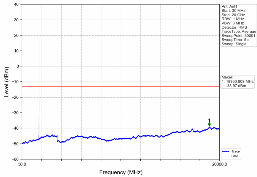
Band66_5MHz_16QAM_HCH_1777.5MHz_RB_1_0_NTNV
