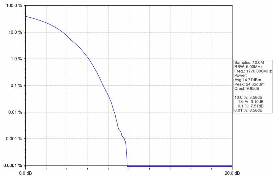
Band66_20MHz_16QAM_HCH_1770MHz_RB_100_0_NTNV
