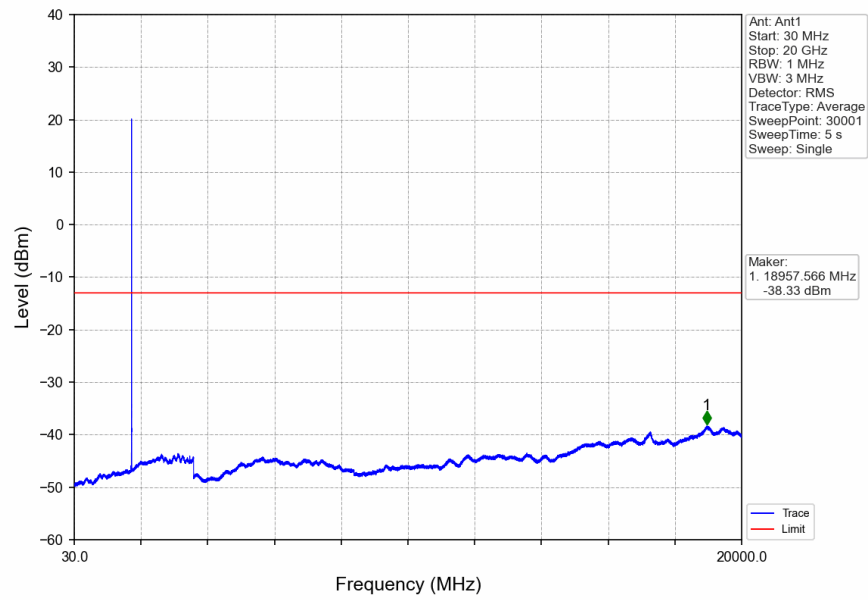
Band66_3MHz_16QAM_HCH_1778.5MHz_RB_1_0_NTNV
