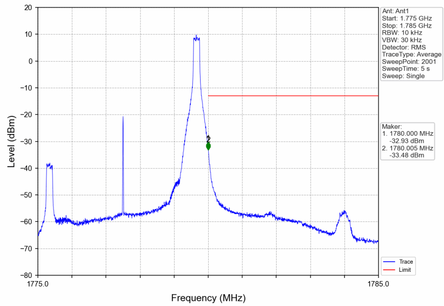
Band66_5MHz_16QAM_HCH_1777.5MHz_RB_25_0_NTNV
