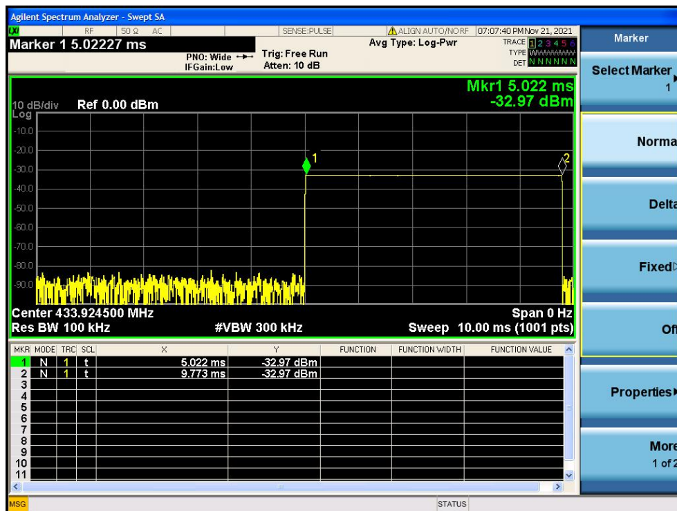
Pulse 1
