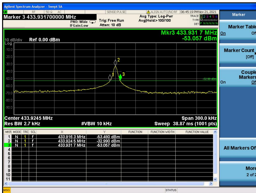
Test plots
