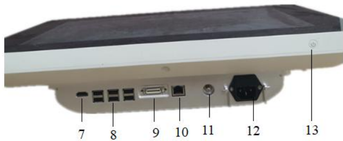
Figure 2-2 Main Unit Interface
