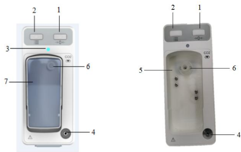
Figure 2-8 CO2 Front View
