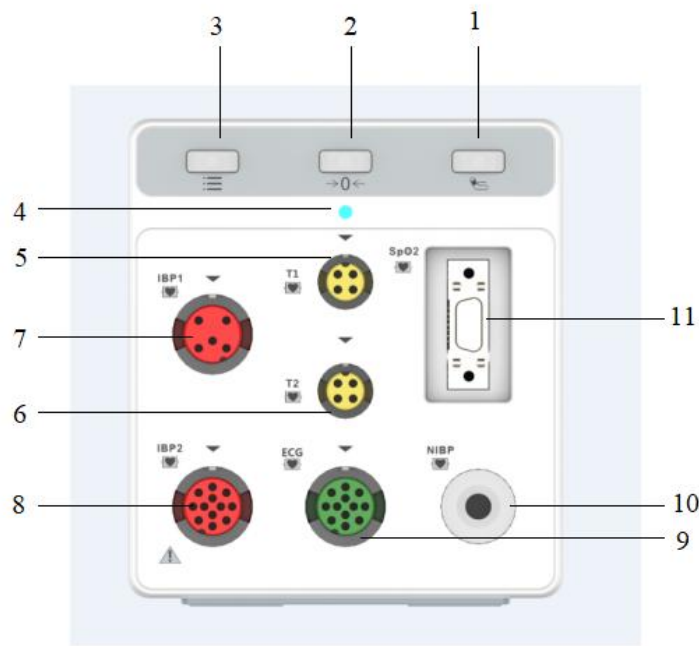
Figure 2-5 P6 Front View
