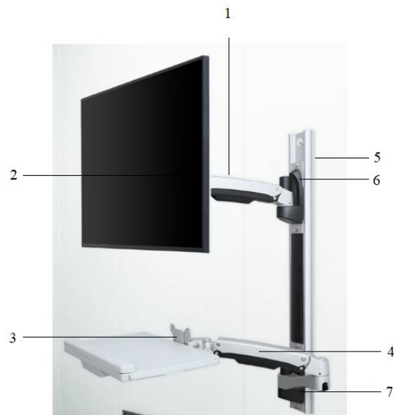
Figure 2-10 Monitor Mount Rendering
