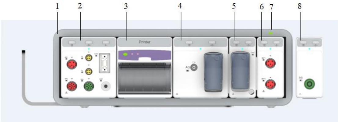
Figure 2-3 Satellite Module Rack (SMR) Front View
