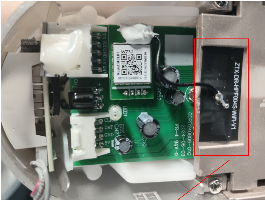
WiFi/BLE Antenna
