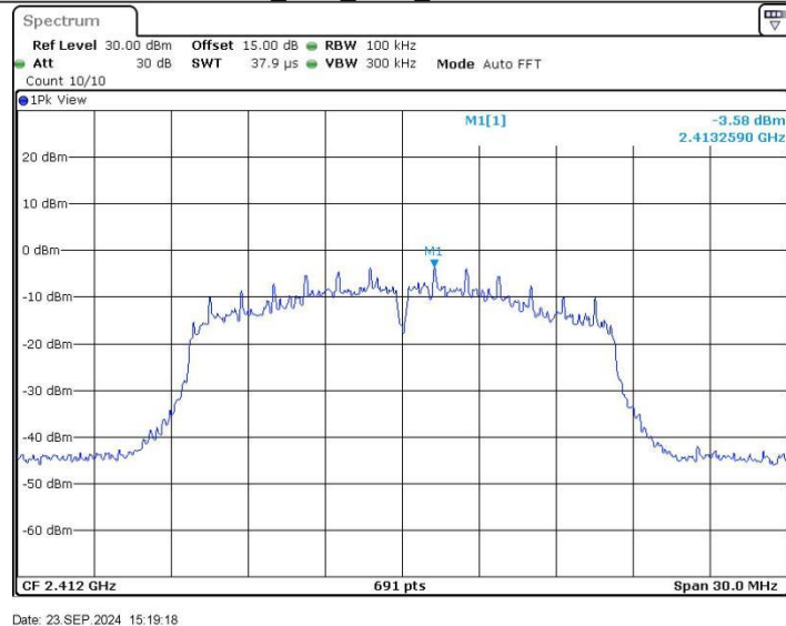
11G_Ant1_2412_0~Reference
