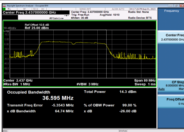
99% Bandwidth-802.11n(HT40),2437MHz ,Ant0
