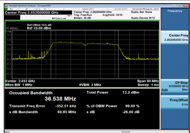
99% Bandwidth-802.11n(HT40),2452MHz ,Ant0
