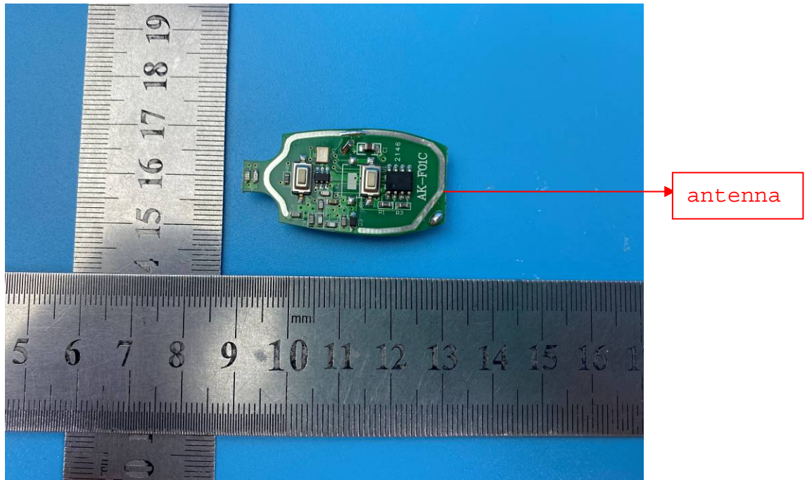
INTERNAL PHOTO OF SAMPLE PCB
