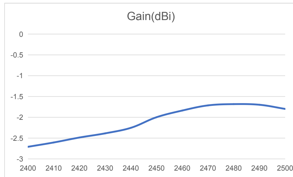
Gain line chart
