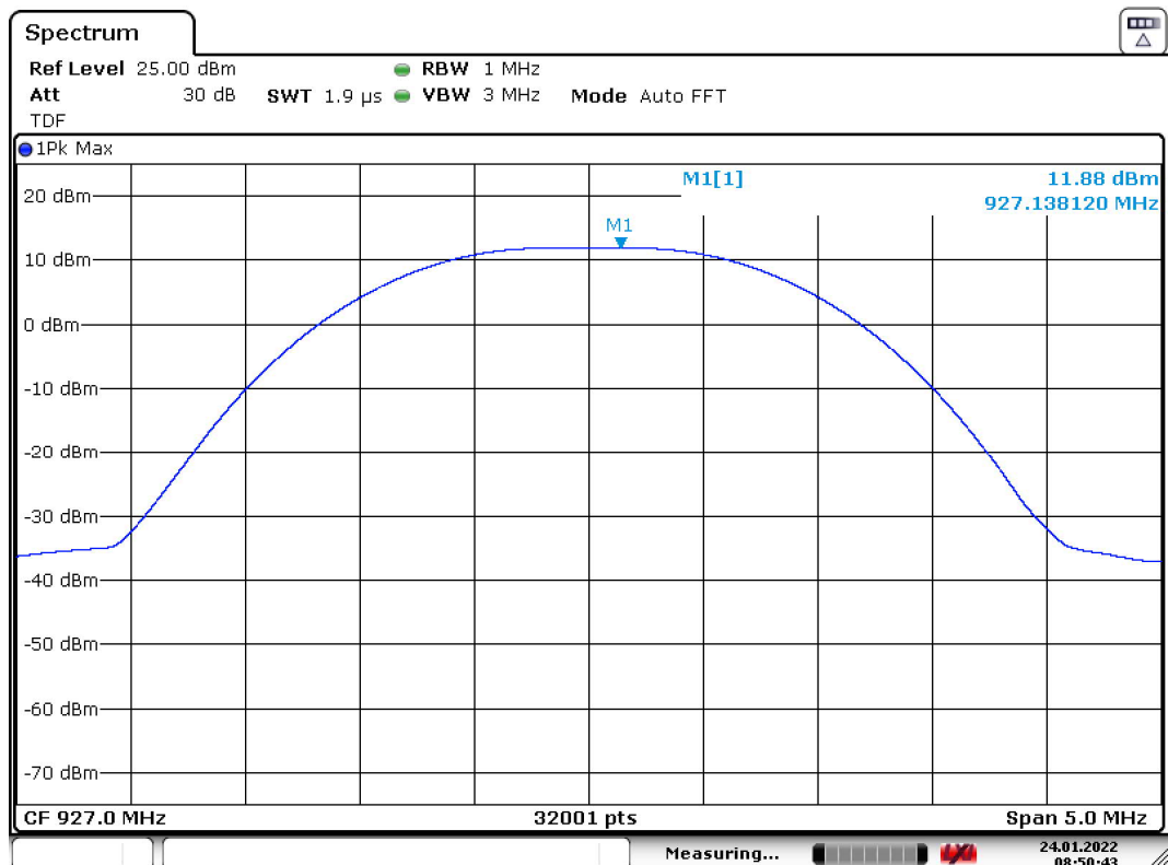
Figure 4: Conducted power, Channel HIGH
